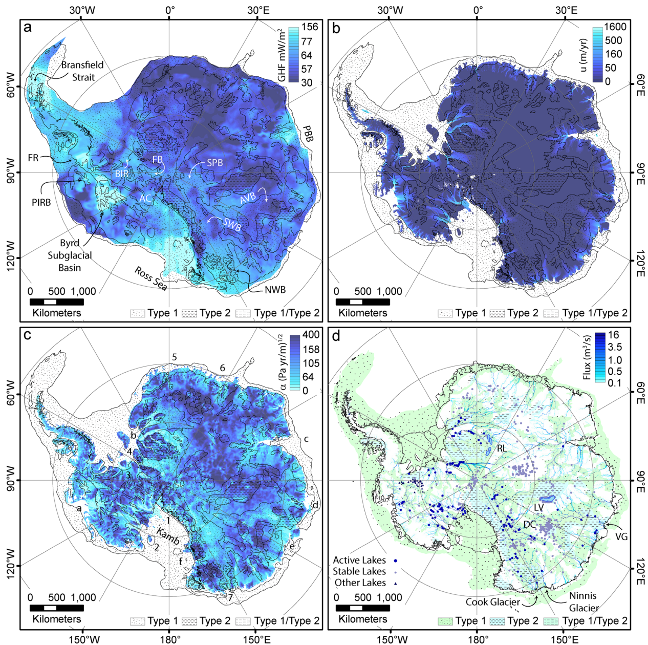
Figure 16. Influences on ice-sheet dynamics showing basins over (a) geothermal heat flux estimated from geophysical data (Lösing & Ebbing, 2021) (b) surface ice sheet velocity derived from InSAR phase mapping (Mouginot et al., 2019) (c) inferred basal friction coefficient derived by inverting for basal conditions using the Ice sheet and Sea level System Model (Dawson et al., 2022) and (d) subglacial hydrology, including subglacial lakes (Livingstone et al., 2022), and a modern-day drainage network (Le Brocq et al., 2013). Numbers indicate ice stream systems with sedimentary basins beneath fast flowing ice including 1-Mercer and Whillans, 2-Bindschadler and MacAyeal, 3-Institute, 4-Academy and Support Force, 5-Jutulstraumen, 6-West and Central Ragnhild, 7-Cook. Letters indicate ice stream systems with basins upstream including (a) Thwaites and Pine Island, (b), Recovery and Slessor, (c) Lambert, Mellor and Fisher, (d) Denman and Scott, (e) Totten, (f) David, Skelton and Byrd. FR, Ferrigno Rift; PIRB, Pine Island Rift Basin; BIR, Bungenstock Ice Rise; AC, Amundsen Coast Basin; FB, Foundation Basin; SPB, South Pole Basin; AVB, Aurora-Vincennes Basin; SWB, Southern Wilkes Basin; NWB, Northern Wilkes Basin; RL, Recovery Lakes; LV, Lake Vostok; DC, Dome C. An unannotated version of this figure is available in Figure S5 in Supporting Information S1.
