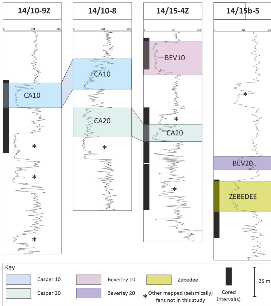
Fig. 4. Wireline logs from wells drilled through the three fans in this study. Gamma Ray (GR) data is provided, showing low values to the left (sandier) and higher values to the right (muddier). The position of the core points within the available well dataset that intersect the three fans is provided (black boxes). Fan system/lobe geobodies are marked, with fan bases/tops interpreted from seismic interpretations data, and checked based on well response (i.e. aligned with nearest sandstone bases). Wells have been correlated where possible (BGS © UKRI 2022).
