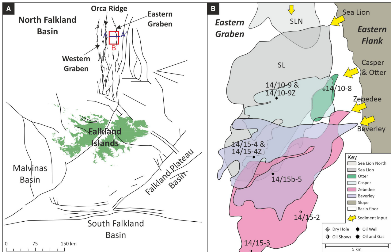
Fig. 2. Location maps and fan outlines. (A) The Falkland Islands and four offshore sedimentary basins: Malvinas Basin, South Falkland Basin, Falkland Plateau Basin and the North Falklands Basin (NFB). The NFB comprises a number of different offset depocentres; however, this study focusses on the ‘Eastern Graben’. The location of line A–A’ in Fig. 3 is shown, represented by an east–west profile across the area of interest; red box denotes position of (B). (B) Mapped polygons that outline the distribution or known extent of the Casper, Zebedee and Beverley fans of this study. For context, the position and known distributions of the Sea Lion North (SLN), Sea Lion and Otter fans have been provided. Three key sediment entry points are shown on these maps with the Sea Lion feeder representing the most northerly point, Otter and Casper sharing an input point, with Zebedee and Beverley entering the basin from the southern-most channel (BGS © UKRI 2022).
