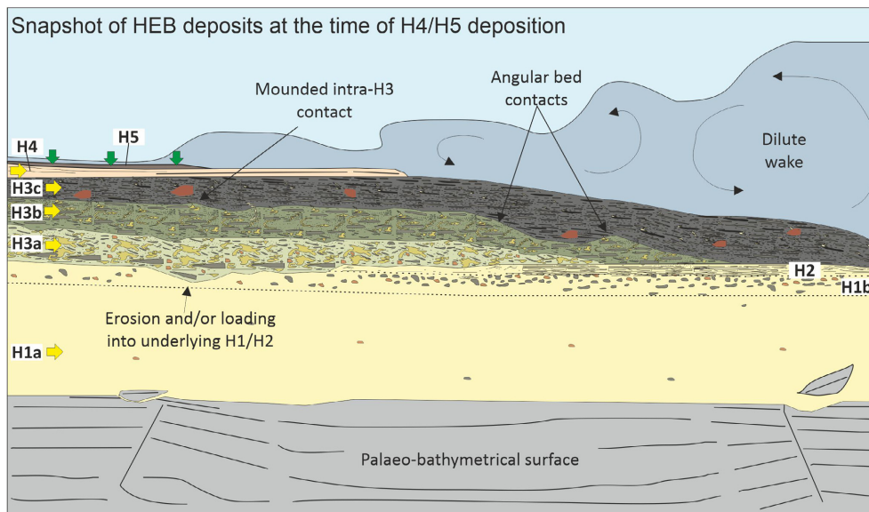
Fig. 12. Schematic model of hybrid event bed emplacement, with particular attention to the H3a, H3b and H3c sub-units. Yellow arrows denote approximate flow direction; green arrows indicate vertical settling. The model represents a ‘snapshot’ at the time of H4/H5 deposition, towards the end of hybrid event bed emplacement. It illustrates the character of ‘H-sequence’ units and sub-units identified in this study, along with their ‘inter-H’ associations (for example, bed contact relationships), and lateral distributions during the emplacement of a single hybrid event bed (BGS © UKRI 2022).
