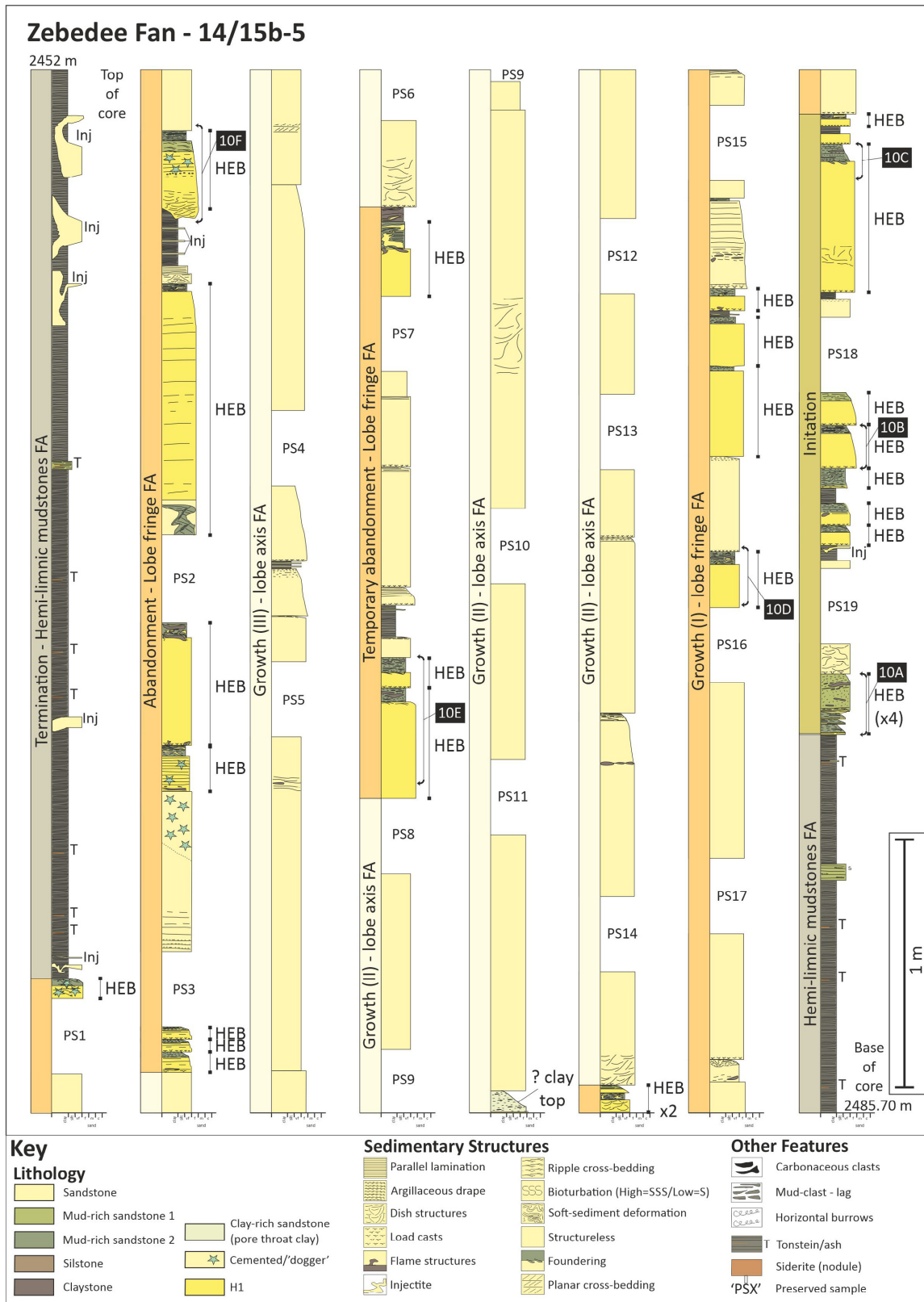
Fig. 15. Sedimentary logs of the Zebedee Fan deposits intersected in well 14/15b-5 (for well location, see Fig. 6) (BGS © UKRI 2022).
