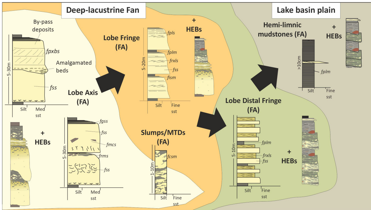
Fig. 19. Idealized facies associations for deep-lacustrine fan systems, based on data from this study, augmented with models from previous studies (after Dodd et al. , 2019). The proximal to distal and/or axial to lateral variability in sedimentology depicts decreasing energy and down-flow transition of flows, in terms of both high-density turbidites and hybrid event beds. (BGS © UKRI 2022).
