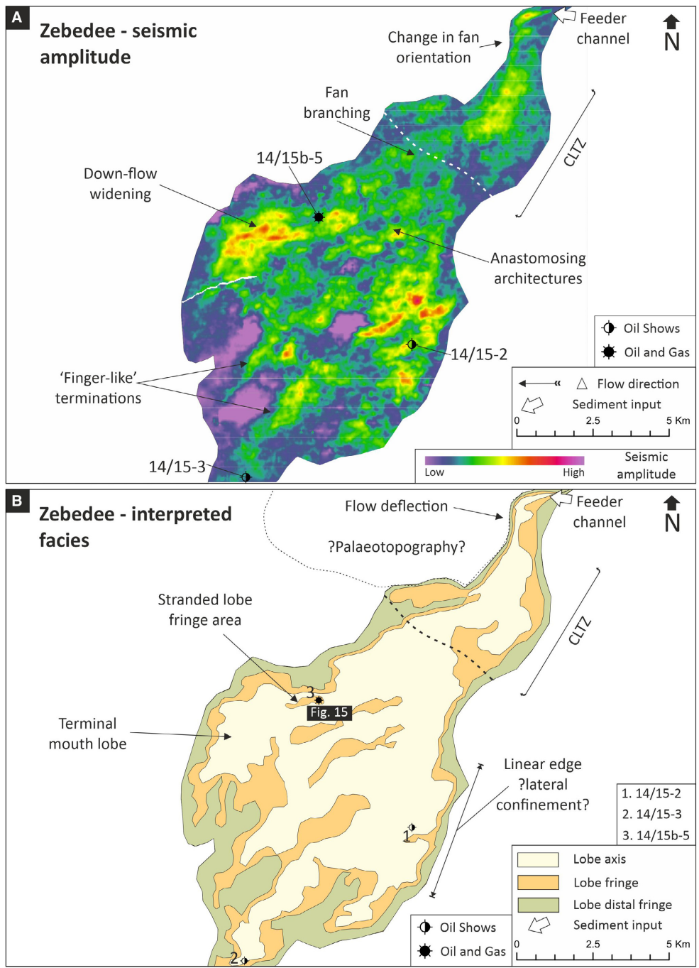
Fig. 6. The planform seismic character and interpreted facies of the Zebedee Fan. (A) Seismic amplitude maps of the Zebedee Fan. (B) Interpreted facies maps from the Zebedee Fan (BGS © UKRI 2022).
