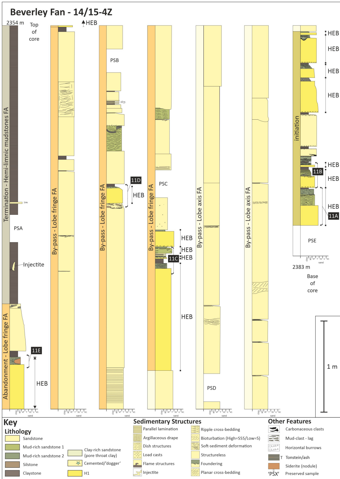
Fig. 17: Sedimentary logs of the Beverley Fan deposits intersected in well 14/15-4Z (for well location, see Fig. 7) (BGS © UKRI 2022).
