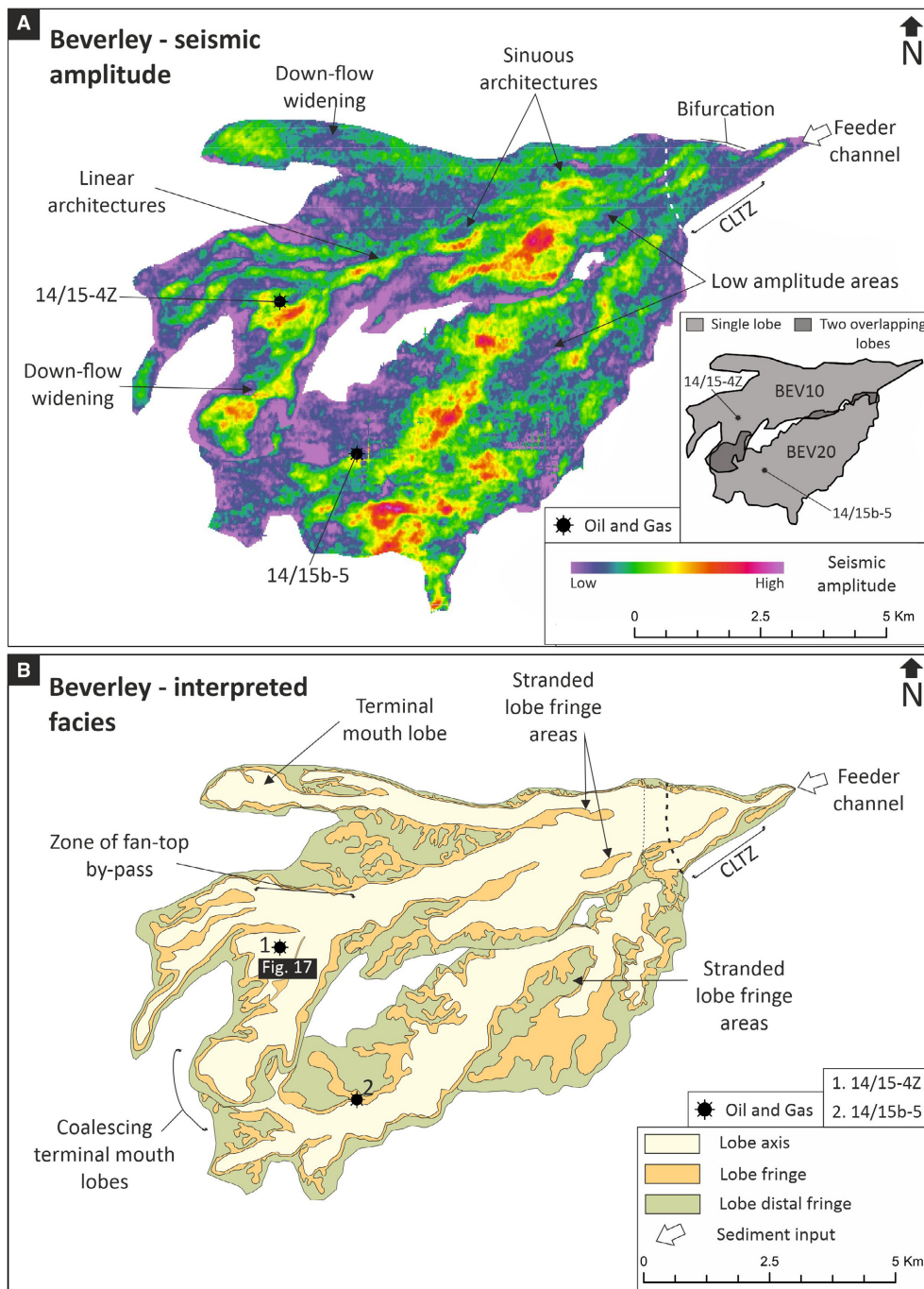
Fig. 7. The planform seismic character and interpreted facies of the Beverley Fan. (A) Seismic amplitude maps of the Beverley Fan. (B) Interpreted facies maps of the Beverley Fan (BGS © UKRI 2022).
