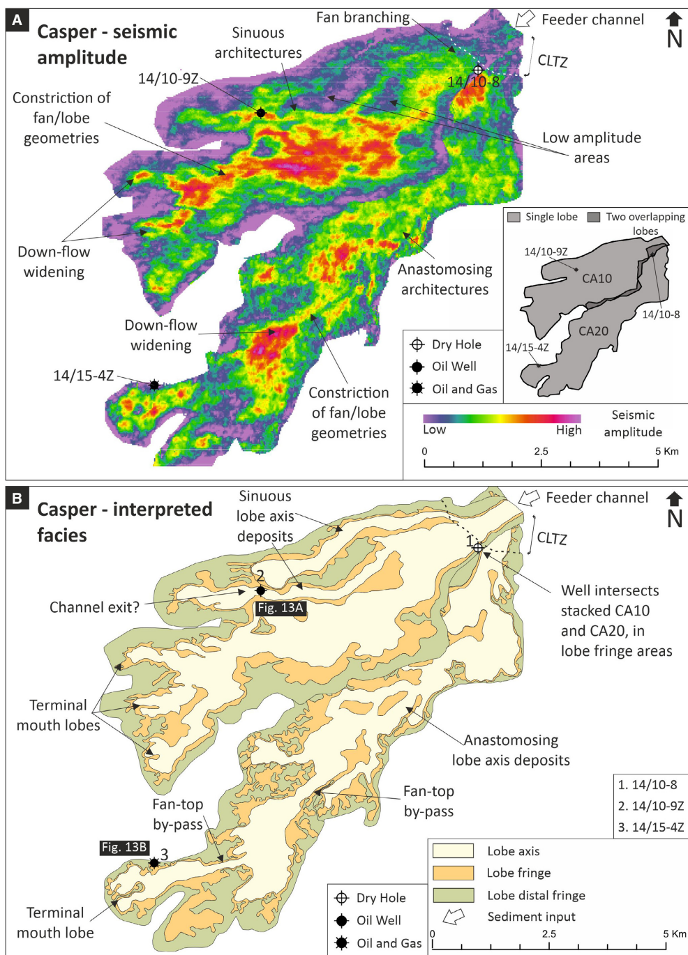
Fig. 5. The seismic character and interpreted facies of the Casper Fan. (A) Seismic amplitude maps of the Casper Fan. The Casper Fan is composed of two lobes, termed CA10 and CA20 (see inset map). A range of internal seismic architectures can be observed from different parts of the fan (see labelled arrows). (B) Interpreted facies maps from the Casper Fan. Three wells intersect Casper, 14/10-8, 14/10-9 and 14/15-4. Core exists from the lobe axis in 14/10-9 (see Fig. 13A), and the lobe fringe in 14/15-4 (see Fig. 13B) (BGS © UKRI 2022).
