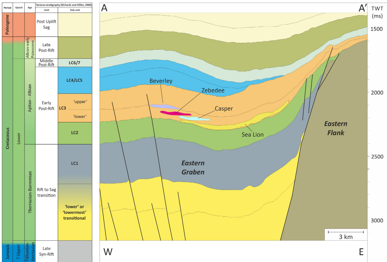
Fig. 3. Stratigraphic framework for the North Falklands Basin, and accompanying east–west oriented geoseismic line showing the overall structure of the Eastern Graben. The stratigraphic position of the fans contained within the study has been marked, all within the LC3 unit (BGS © UKRI 2022).
