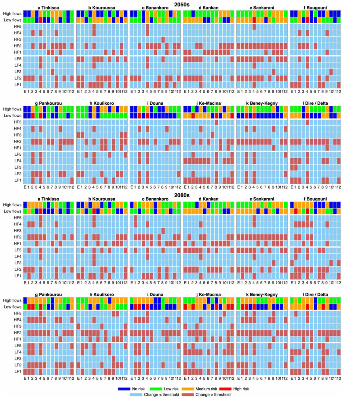
Figure 2 | ERA environmental flow results for 12 gauging stations in the Upper Niger for the 2050s and 2080s. The lower part of each subplot identifies whether individual high (H)- and low (L)-flow MFRIs are above the thresholds associated with an assumed significant change. The top part of each subplot presents the traffic-light colour-coded classification of risks of ecological change for high and low flows. Results are shown for the ensemble mean (E) and each of the 12 GCM groups.
