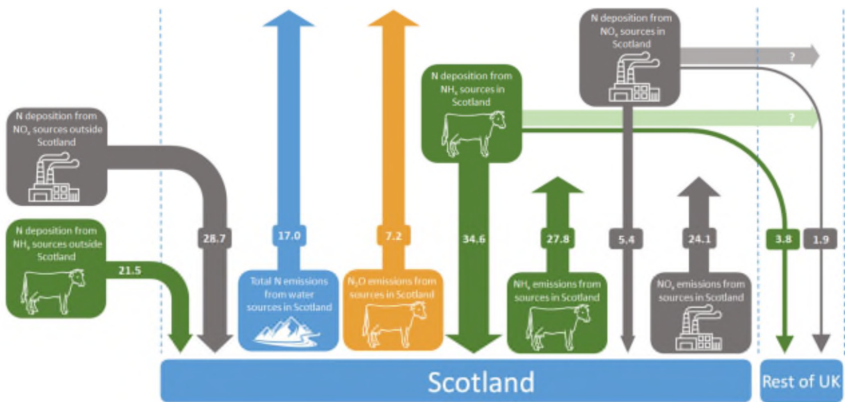
Figure 2: Atmospheric nitrogen budget for Scotland from the CBED model ( \text{kt N yr}^{-1} ), with atmospheric emissions from the NAEI and source apportionment and import/export derived from work by Bealey and Dore (2017) and Smith et al. (2018). Only \text{NO}_x and \text{NH}_x emissions are considered for N deposition, \text{N}_2\text{O} etc. remain in the atmosphere. N.B. values may not add up due to rounding.
