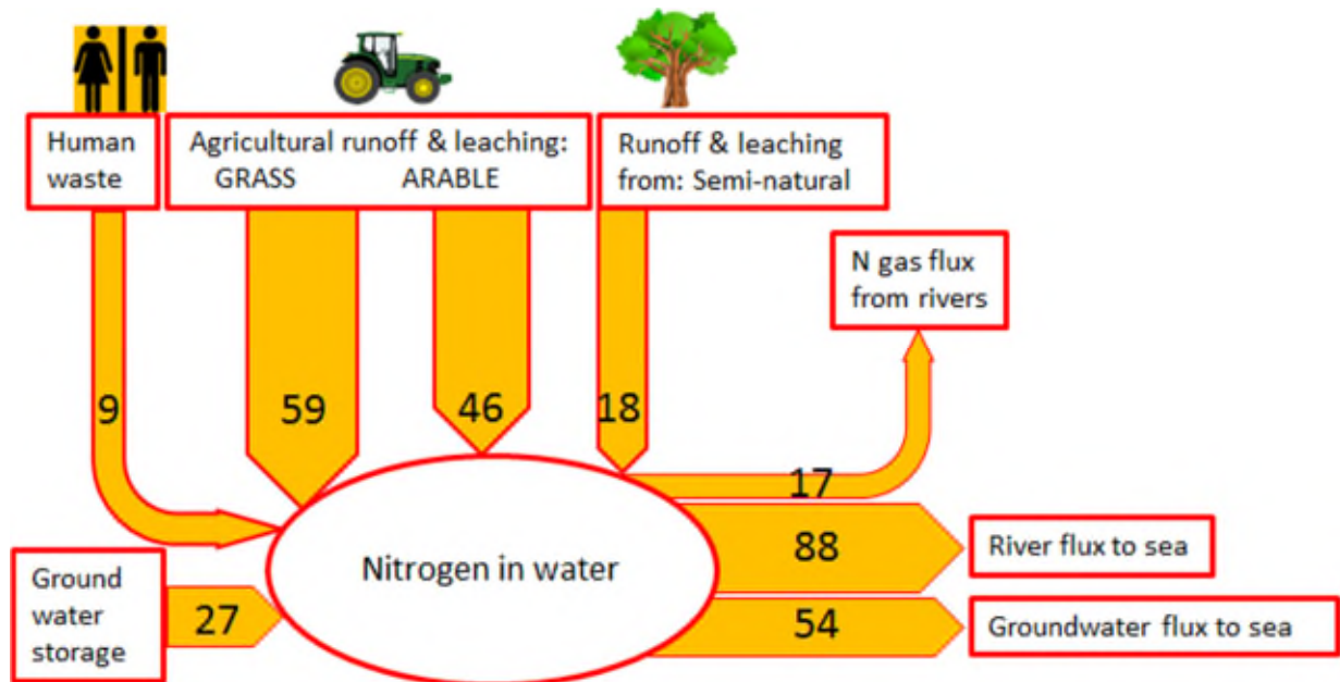
Figure 1. Hydrosphere/soil nitrogen budget (2010) using outputs from the LTLS-IM macronutrient model (kt N yr -1 ).
