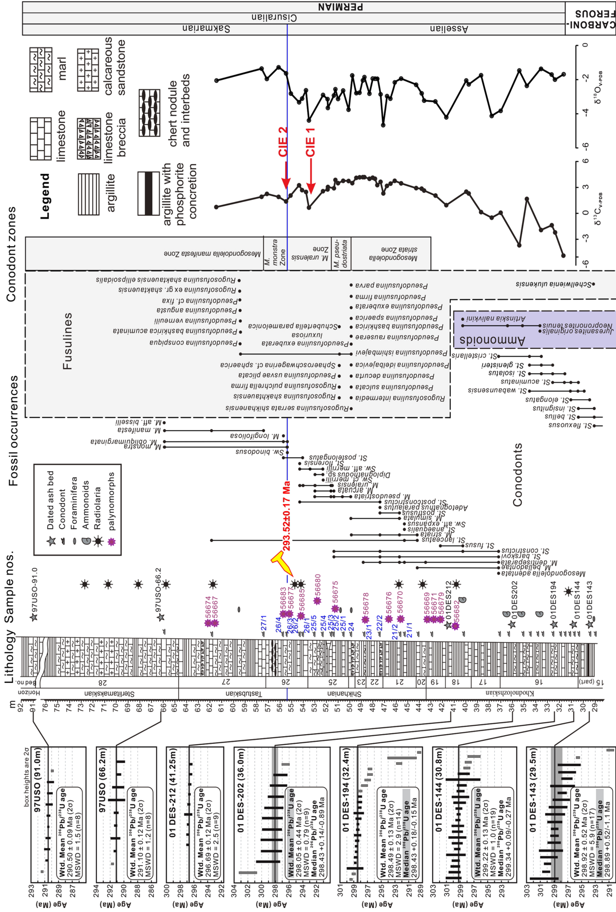
Figure 4. Composite data of the Usolka section showing the lithology, biostratigraphy, geochronology (after Schmitz and Davydov, 2012) and chemostratigraphy (Zeng et al., 2012). Ammonoids are only available from the Upper Carboniferous and fusulinaceans are only distributed in the Asselian and Sakmarian. Conodont, fusulinacean, radiolarian, ammonoid and palynological marks on the right side of the lithologic column represent samples collected. Conodont sample numbers are in blue, palynological numbers are in purple. Sample numbers with DES or USO are geochronological numbers. Sample numbers throughout the column also refer to the sample numbers specified in the description of the section. CIE=carbon isotope excursion.
