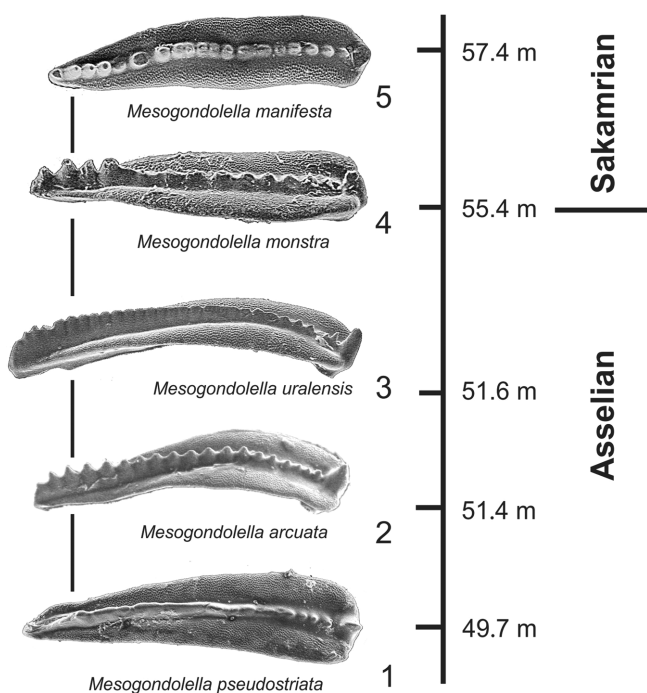
Figure 8. The evolutionary lineage of the genus Mesogondolella in the Asselian-Sakmarian transitional interval.
