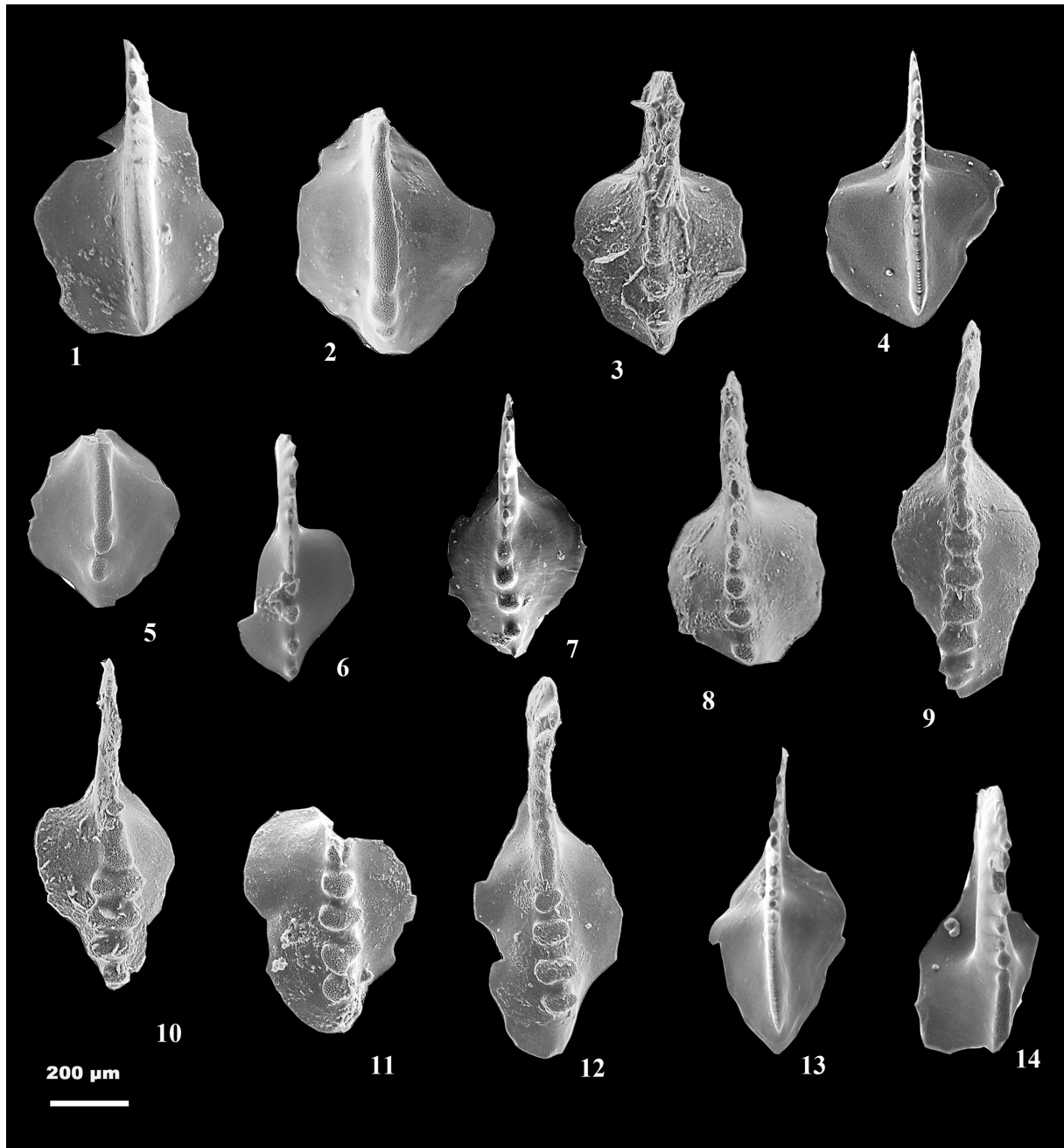
Figure 7. Key Sweetognathus species around the Asselian-Sakmarian boundary at the Usolka and Kondurovsky sections in the southern Urals. 1, 2. Sweetognathus expansus (Perlmutter): 1 – Specimen U17-25, Usolka section, Bed 14; 2 – Specimen U37A-1, Usolka section, Bed 21; 3. Sweetognathus aff. merrilli Kozur: 3 – Specimen U32A-2; 4. Sweetognathus aff. stevensi (Clark and Carr), Specimen K36-18, Kondurovsky section, Bed 18; 5 – 7. Sweetognathus aff. merrilli Kozur: 5 – Specimen K36-16 (form transitional from Sw. stevensi to Sw. aff. merrilli ); Kondurovsky section, Bed 16; 6 – Specimen K36-20; 7 – Specimen K36-20b; Kondurovsky section, Bed 18; 8 – 12. Sweetognathus binodosus Chernykh: 8 – Specimen U32A-3; 9 – Holotype U32A-6; 10 – Specimen U32A-7; 11 – Specimen U32A-4; 12 – Specimen U32A-5; Usolka section, Bed 26/3; 13. Sw. aff. stevensi (Clark and Carr), the middle part of Bed 16; 14. forms transitional from Sw. aff. stevensi (Clark and Carr) to Sw. aff. merrilli Kozur, upper part of Bed 16, Kondurovsky section.
