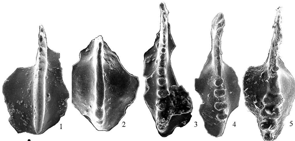
A Evolutionary trend of species of Sweetognathus in the Usolka section
