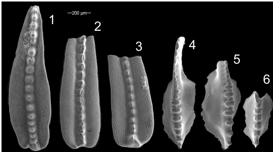
Figure 12. Conodonts around the base of Sakmarian at Carlin Canyon in northern Nevada, USA. 1. Mesogondolella monstra (transitional? with M. striata ), Sample 684; 2. M. monstra , Sample 684; 3. M. monstra (transitional? with M. obliquimarginata , Sample 685; 4. Sweetognathus binodosus , Sample 685; 5. Sw. binodosus , Sample 685; 6. Sw. binodosus , Sample 684. Material is from the unpublished MSc thesis of Elinda Dehari at the University of Calgary. Sample 685 is about 2 m higher than Sample 684 in a section that is several hundred metres thick; both are from the lower Buckskin Mountain Formation. These specimens occur above the last Streptognathodus in the section including St. fusus and St. postfusus .
