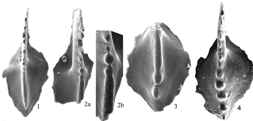
B Evolutionary trend of species of Sweetognathus in the Kondurovsky section
