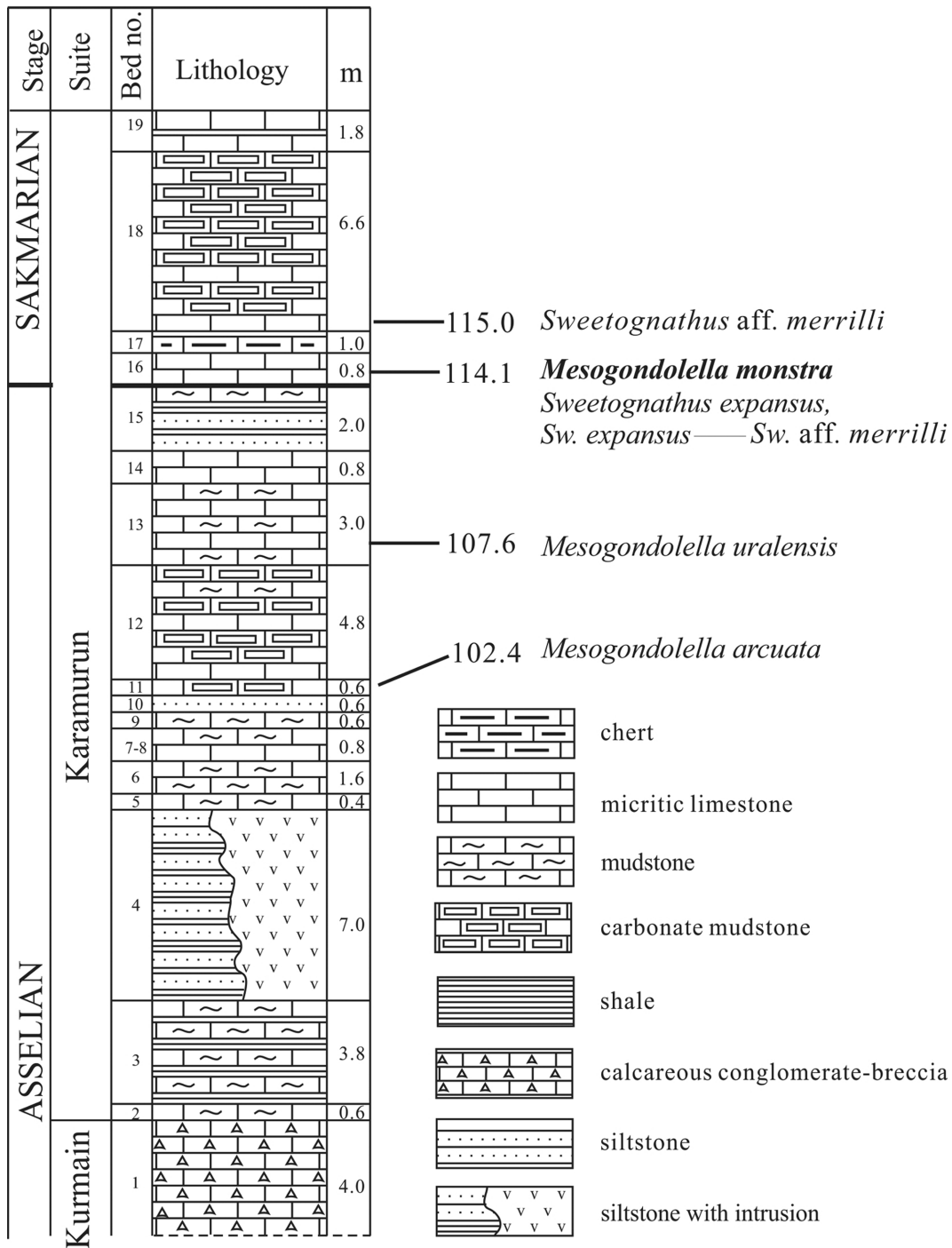
Figure 5. Stratigraphic column of the Asselian-Sakmarian interval with the characteristic species and zones of conodonts of the Kondurovsky section.
