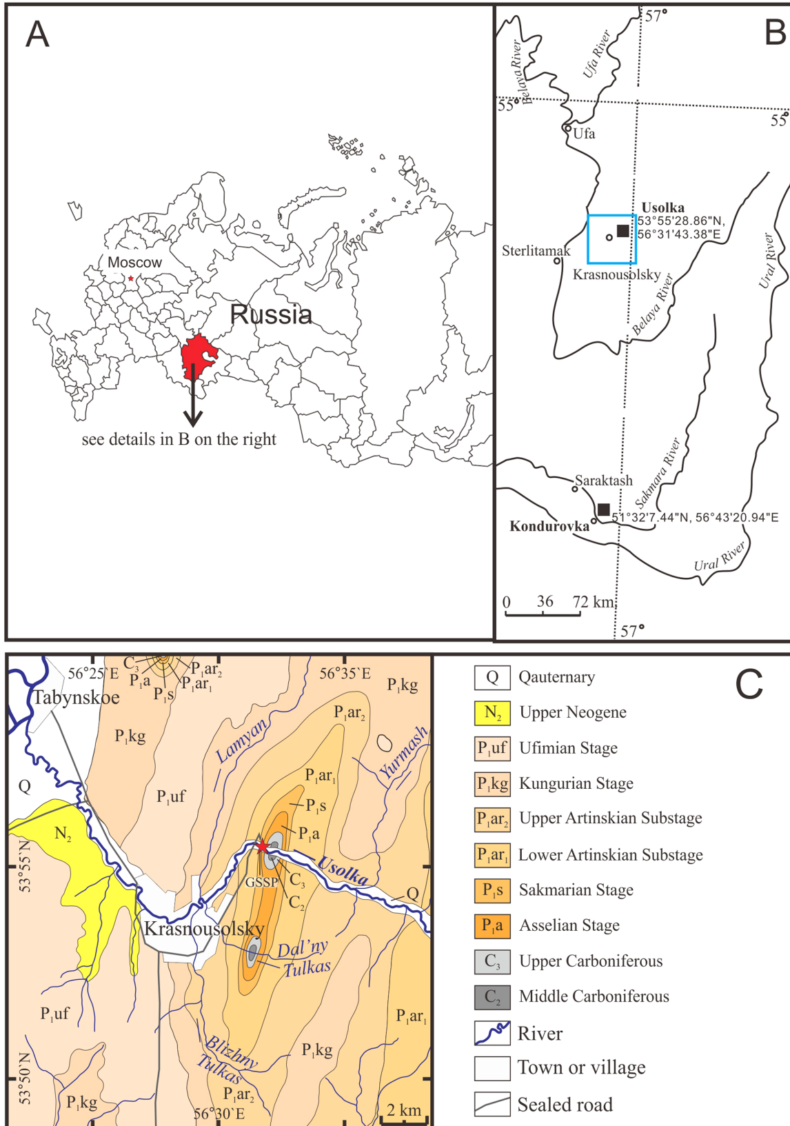
Figure 1. (A) Location of Usolka section in Republic Bashkortostan, Russia (Bashkortostan is marked in red); (B) Location of the Usolka and Kondurovsky sections; (C) Geological map, showing the studied area and the location of the GSSP section for the base of the Sakmarian Stage (indicated by red star).
