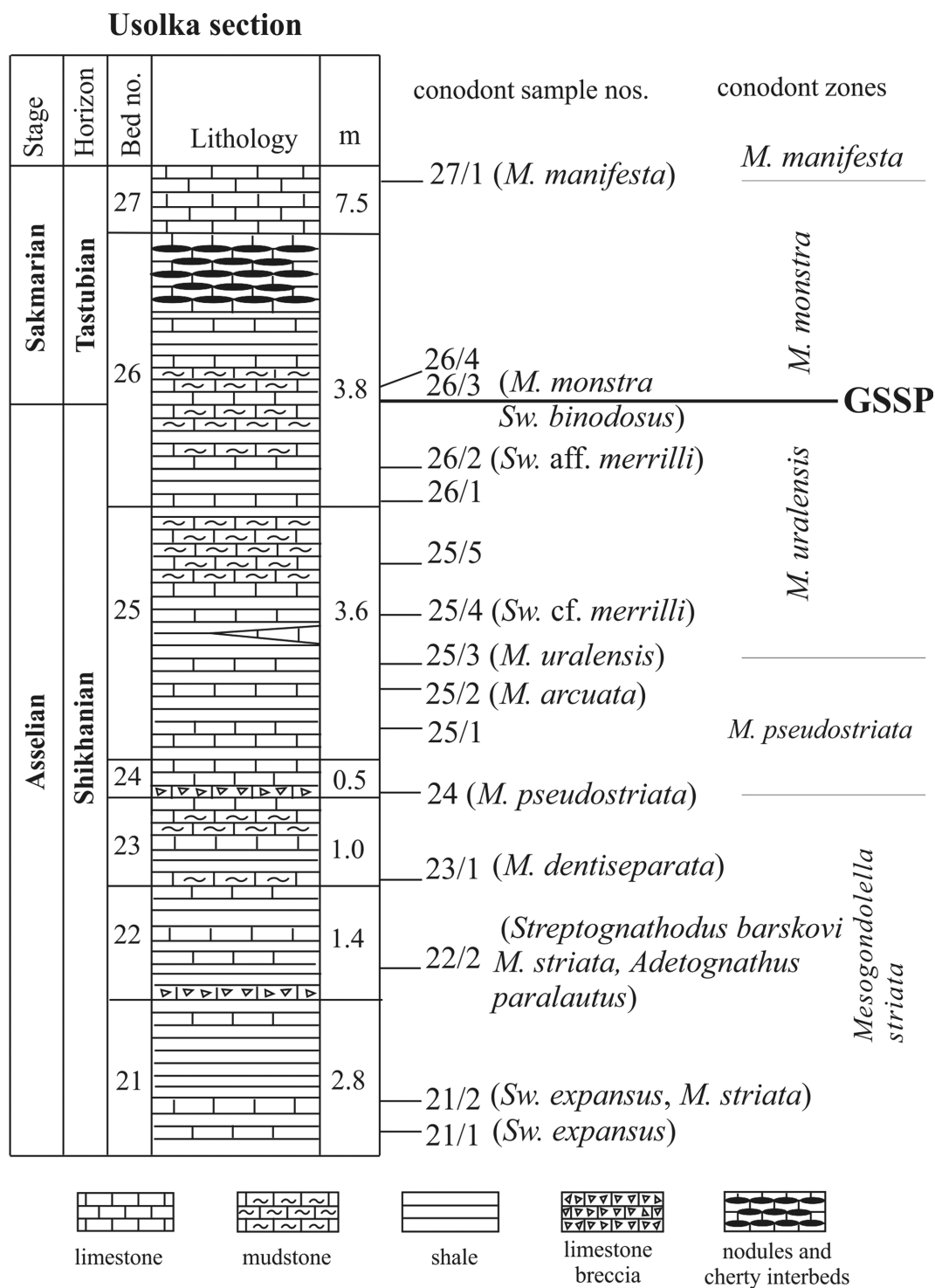
Figure 3. Stratigraphic column of the Asselian-Sakmarian interval with the characteristic species and zones of conodonts of the Usolka section.
