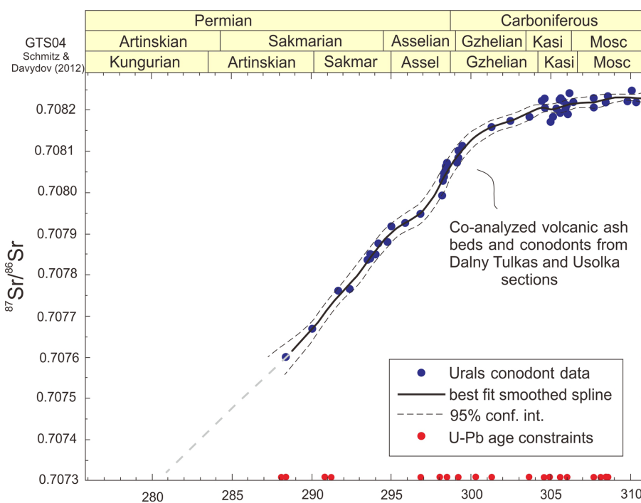
Figure 11. Age model for Sr-isotopic work by Mark Schmitz at the Dalny Tulkas and Usolka sections in southern Urals (modified from Henderson et al., 2012).
