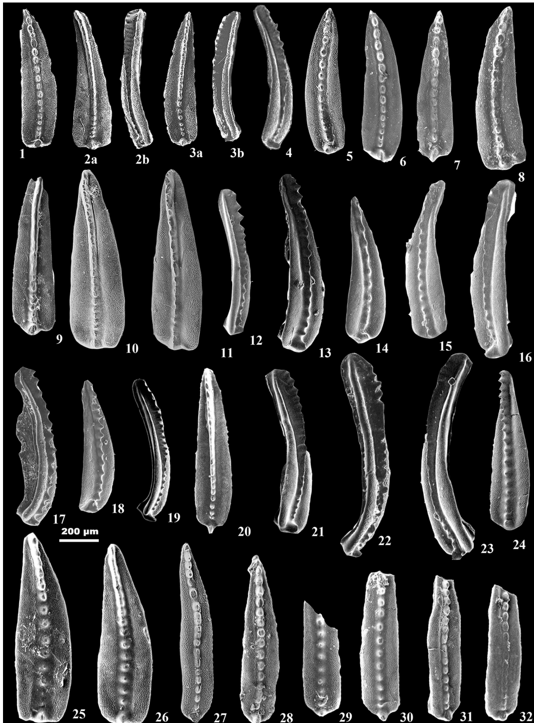
Figure 6. Key Mesogondolella species around the Asselian-Sakmarian boundary at the Usolka and Kondorovsky sections in the southern Urals. 1. Mesogondolella striata (Chernykh); Specimen U34-8; Usolka section, Bed 22/2; 2. M. pseudostrata (Chernykh); Specimen U37-21, Usolka section, Bed 25/2; 3. M. uralensis (Chernykh); Specimen U38-7; Usolka section, Bed 25/3; 4. M. uralensis (Chernykh). Specimen K35-14, Kondurovsky section, Bed 13. 5-8. Mesogondolella striata (Chernykh): 5 – Specimen U34-4; 6 – Specimen U34-5; 7 – Specimen U34-6; 8 – Specimen U34-7; Usolka section, Bed 21/1; 9, 10. Mesogondolella pseudostrata (Chernykh): 9 – Specimen U37-19; 10 – Specimen U37-31; Usolka section, Bed 25/2; 11. Mesogondolella pseudostrata (Chernykh) (transitional to M. obliquimarginata (Chernykh), Specimen U37-33; Usolka section, Bed 25/2; 12-18. Mesogondolella arcuata Chernykh: 12 – Specimen U34-47; Usolka section, Bed 25-2; 13 – Specimen K35-5m; 14 – Specimen K35-4; 15 – Specimen K35-2; 16 – Specimen K35-1; Kondurovsky section, Bed 10; 17 – Specimen K35-9; 18 – Specimen K35-10; Kondurovsky section, Bed 12; 19 – 23. Mesogondolella uralensis (Chernykh): 19 – Specimen U38-9; 20 – Specimen U38-2; 21 – Specimen U38-6; 23 – Specimen U38-5; Usolka section, Bed-26/1; 22 – Specimen U37-21; Usolka section, Beds-25/5; 24-26. Mesogondolella monstra Chernykh: 24 – Specimen K36-8; Kondurovsky section, Bed 16; 25 – Specimen U32-14; 26 – Specimen U32-15; Usolka section, Bed. 26/3; 27-32. Mesogondolella manifesta Chernykh: 27 – Holotype, U38-43; 28 – Specimen U38-47; 29, Specimen U38-32; 30 – Specimen U38-45; 31 – Specimen U38-46; 32 – Specimen U38-44; Usolka section, Bed 27/1.
