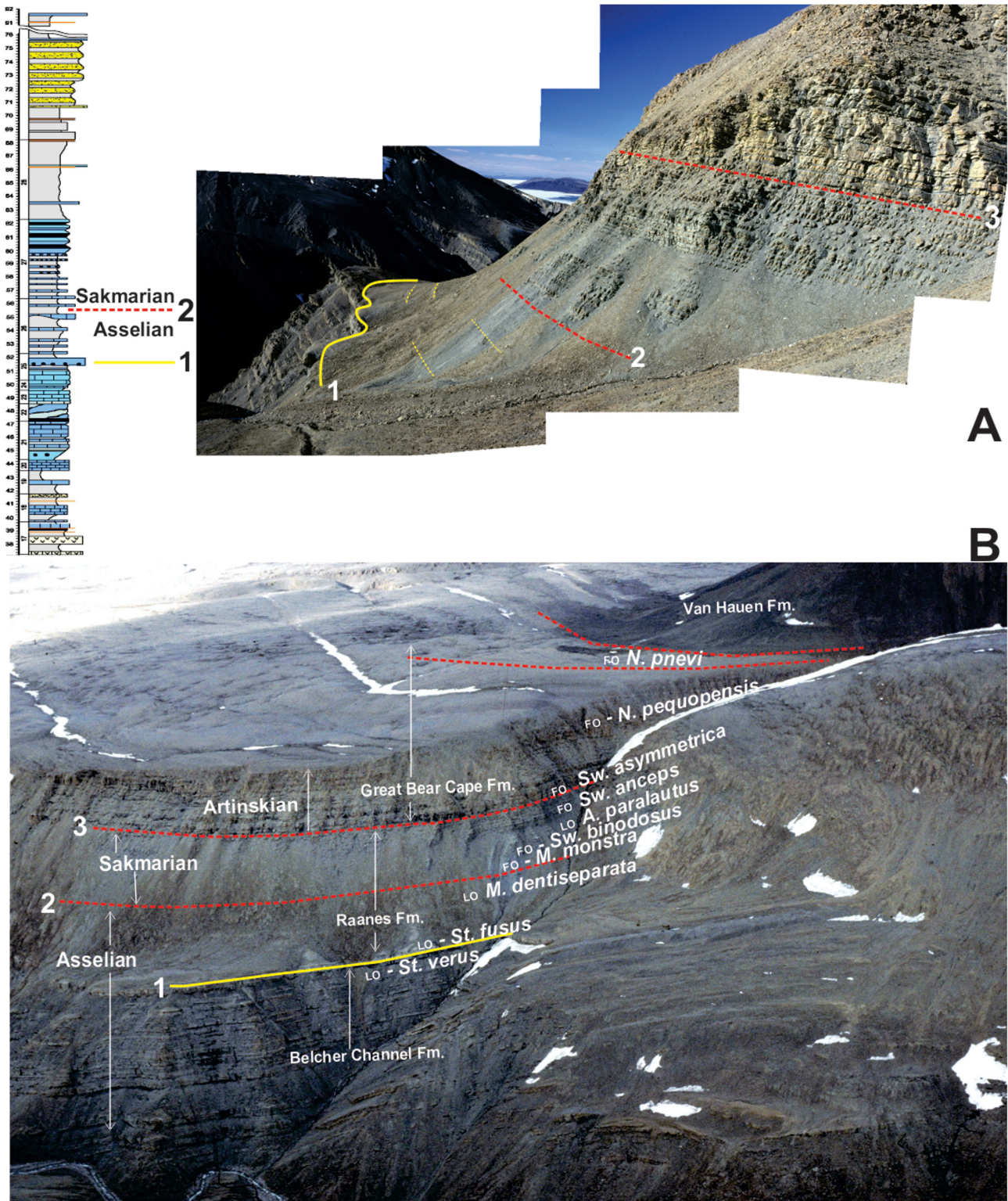
Figure 10. Two views of the East Blind Fiord section in the Canadian Arctic (78°24'N; 085°35'W) are shown as a means of correlation based on lithologic pattern and biostratigraphy. A. View to the SW from the section. B. View to the west from helicopter. Level 1 (solid yellow line) represents a SB and significant change in carbonate sedimentation from cyclothems and photozoan assemblages below and in two minor cyclothems (yellow dashed lines) above. This is compared to a change in lithology at Usolka (colored stratigraphic column top left). Level 2 is maximum flooding surface of first of two long duration shallowing upward cycles with heterozoan assemblage. Level 2 correlates with FO of Mesogondolella monstra (M.) and thus the Asselian–Sakmarian boundary; FO of Sweetognathus (Sw.) binodosus is slightly higher. The last occurrence (LO) of Carboniferous holdover taxa including Streptognathodus (St.) and Adetognathus (A.) are shown. Surface 3 is the FO of Sweetognathus asymmetrica and the base of the Artinskian. The thickness between surfaces 1 and 3 is about 170 m. A thin unit of Kungurian is also shown (see Mei et al., 2002) with Neostreptognathodus (N.) pnevi as well as the major latest Kungurian–Roadian transgressive succession of the Van Hauen Formation.
