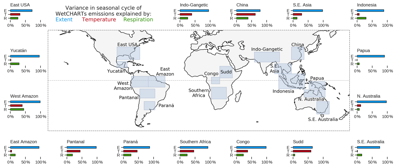
Figure 3. Explained variance ( R^2 ) calculated as the individual partial correlation between the seasonal cycle of the WetCHARTs CH 4 emissions and the seasonal cycles in the wetland extent fraction, temperature dependency and heterotrophic respiration for each region that were used to derive the WetCHARTs emissions. These values are averaged across all ensemble members to give an indicative value for the sensitivity of each region to the different driving parameters. Note that due to potential cross-correlations, it is not necessarily expected that the percentages sum to 100 %.
