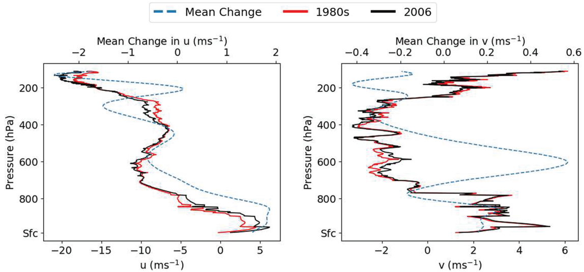
FIGURE 5 Control profile (black) for u and v with the ERA-Interim reanalysis trend from 1982–2017 deduced (red). The change between profiles is shown in blue (dashed)
