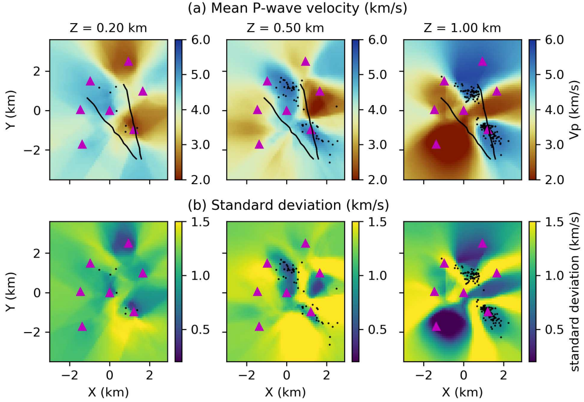
Figure A1. Horizontal slices through the 3D P-wave velocity model obtained using body wave travel time only. Key as in Figure 6.
