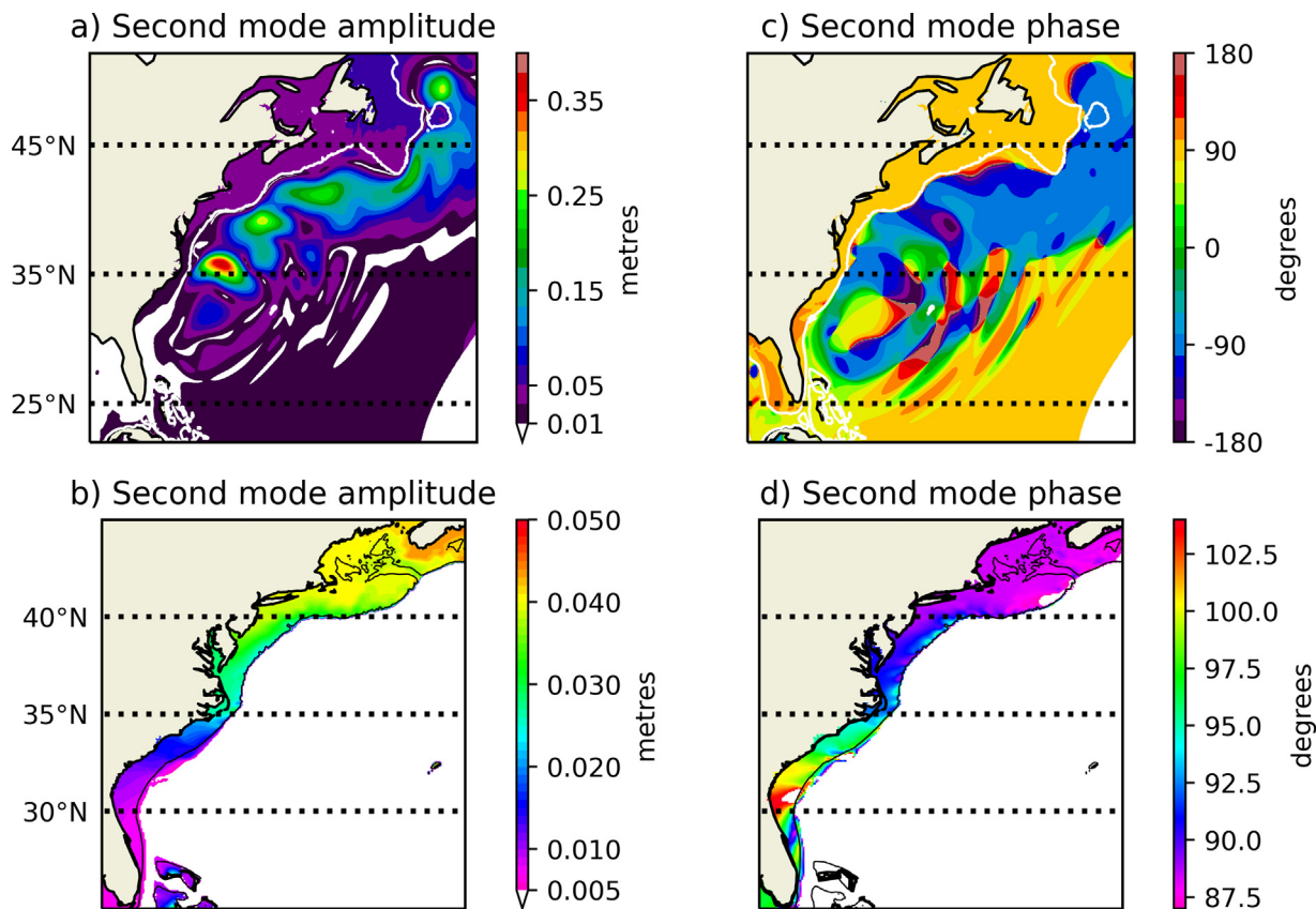
Fig. 6. As in Fig. 4 but for closed northern and southern boundaries.
