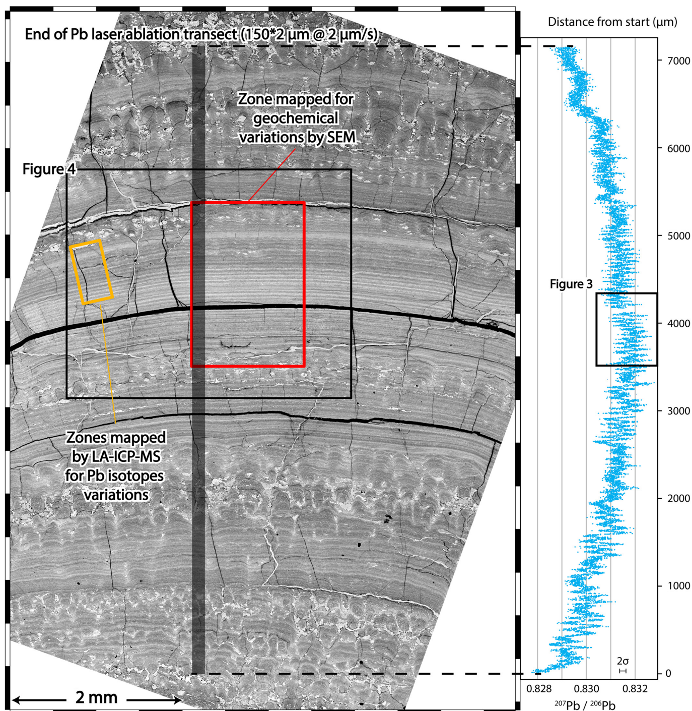
Fig. 2. Backscatter electron microscope image of the area studied in sample 085_004 showing intervals of laminar Fe-Mn oxides alternating with a columnar texture in which the intercolumnar space is filled by carbonate-fluoro-apatite (Josso et al., 2020b). The transect and zones analysed for Pb isotopes by LA-MC-ICP-MS and phase mapping by SEM are shown in the overlay. The black rectangles represent the zones shown in Figs. 3 and 4. The ^{207}\text{Pb}/^{206}\text{Pb} ( \pm 0.015\% , 2\sigma ) isotope profile used for cyclostratigraphy is shown on the right hand side. The complete dataset is available in supplementary information (DOI: https://doi.org/10.5285/7a9eb43f-a5c4-450c-9fe1-c60f2703a1d1 ).
