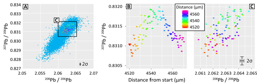
Fig. 7. (A) ^{208}\text{Pb}/^{206}\text{Pb} vs. ^{207}\text{Pb}/^{206}\text{Pb} plot of the entire transect. Note how the data plot along a single trend suggesting simple binary mixing. (B) Extract of a single ^{207}\text{Pb}/^{206}\text{Pb} oscillation, colour coded as a function of distance in the record (Fig. 2). (C) Spread of the single oscillation in Pb-Pb space (duplicated in panel A). The similar slope between the whole transect and each oscillation indicates that a two end-member mixing regime is likely to be responsible for the long- and short-term Pb isotope variations in this record.
