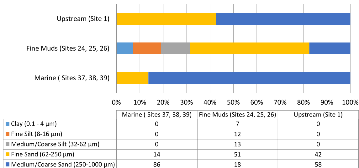
Fig. 5. Grain size distribution of samples from the Conwy Estuary.
