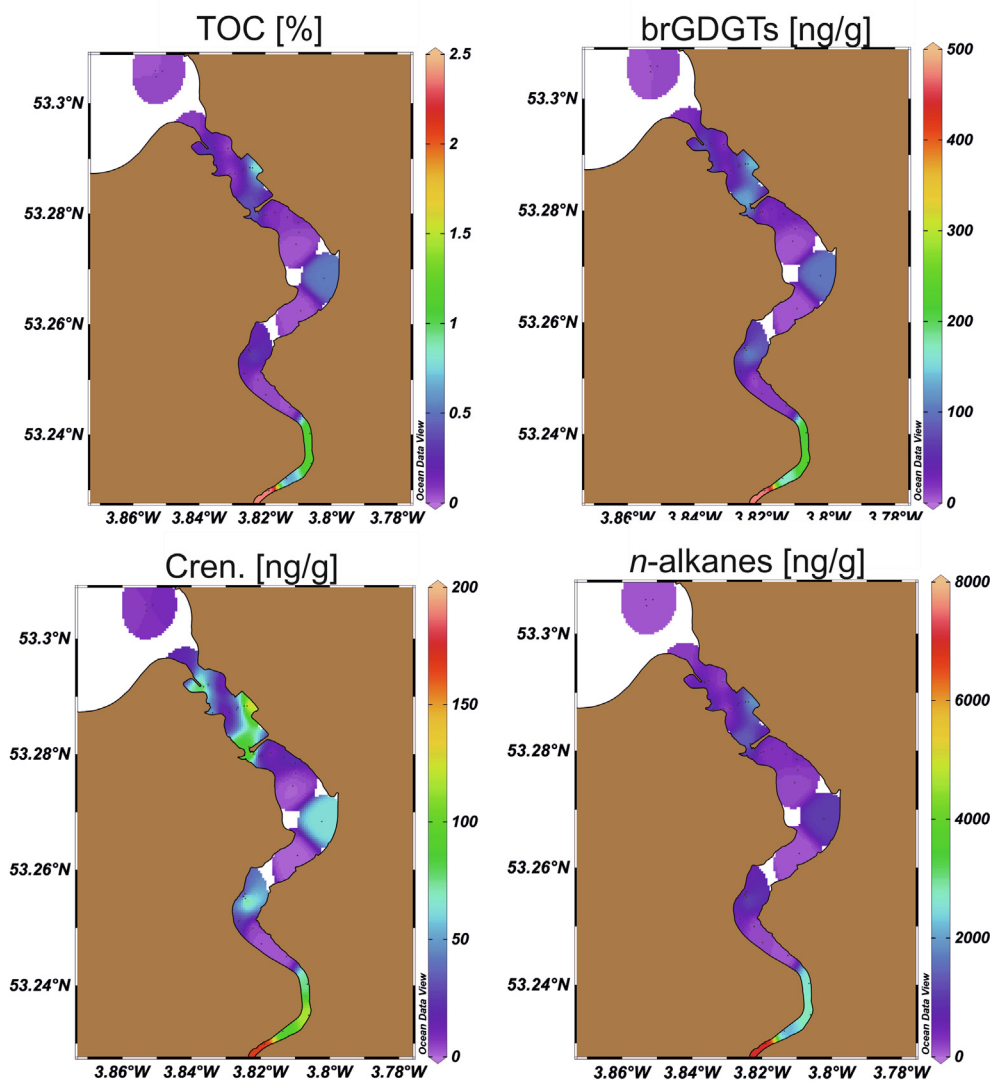
Fig. 2. Longitudinal distribution (from land to sea) of TOC and biomarkers (ng/g) along the Conwy Estuary.
