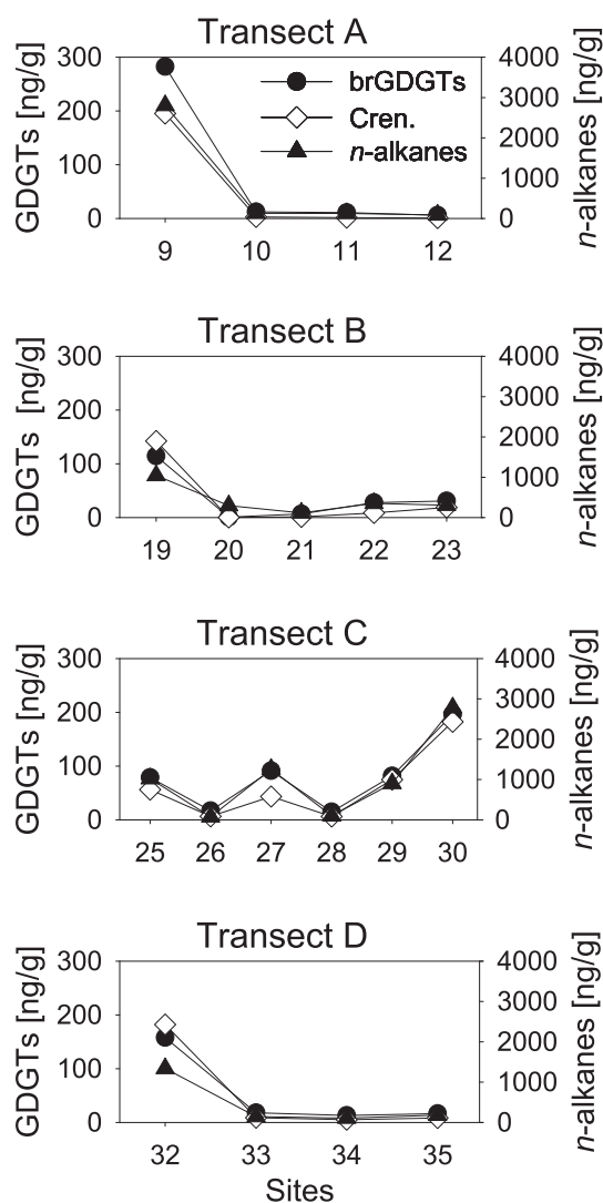
Fig. 3. Biomarkers distribution along transects A–D.
