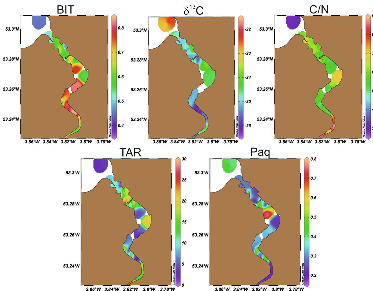
Fig. 4. Terrestrial vs aquatic carbon input proxies along the Conwy Estuary.
