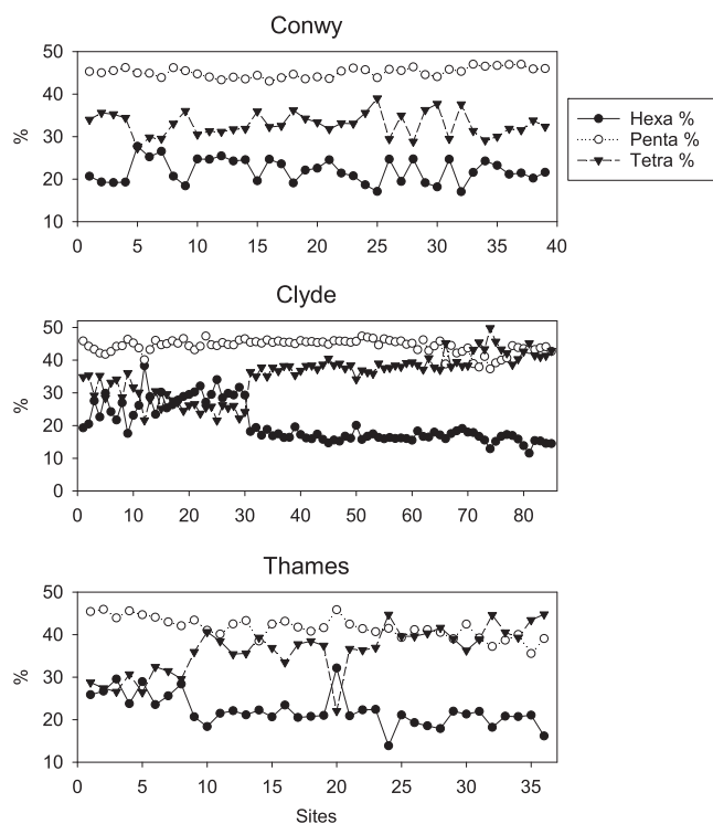
Fig. 8. Longitudinal variations of the fractional abundance of the tetra-, penta- and hexamethylated brGDGTs in the Conwy Estuary, the Clyde river-estuary and the Thames Estuary.
