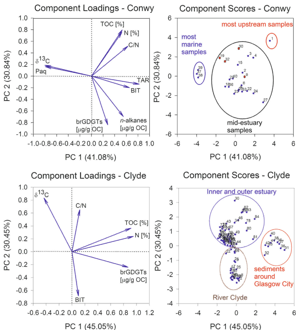
Fig. 9. Component loading and scores for the Conwy Estuary and Clyde river-estuary (the Clyde river dataset is from Lopes dos Santos and Vane, 2019).
