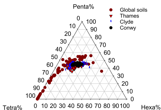
Fig. 7. Ternary plot of fractional abundances of the brGDGTs from the Conwy Estuary together with the global soils (De Jonge et al., 2014b) and sediments from the Thames and the Clyde (Lopes dos Santos and Vane 2016, 2019).
