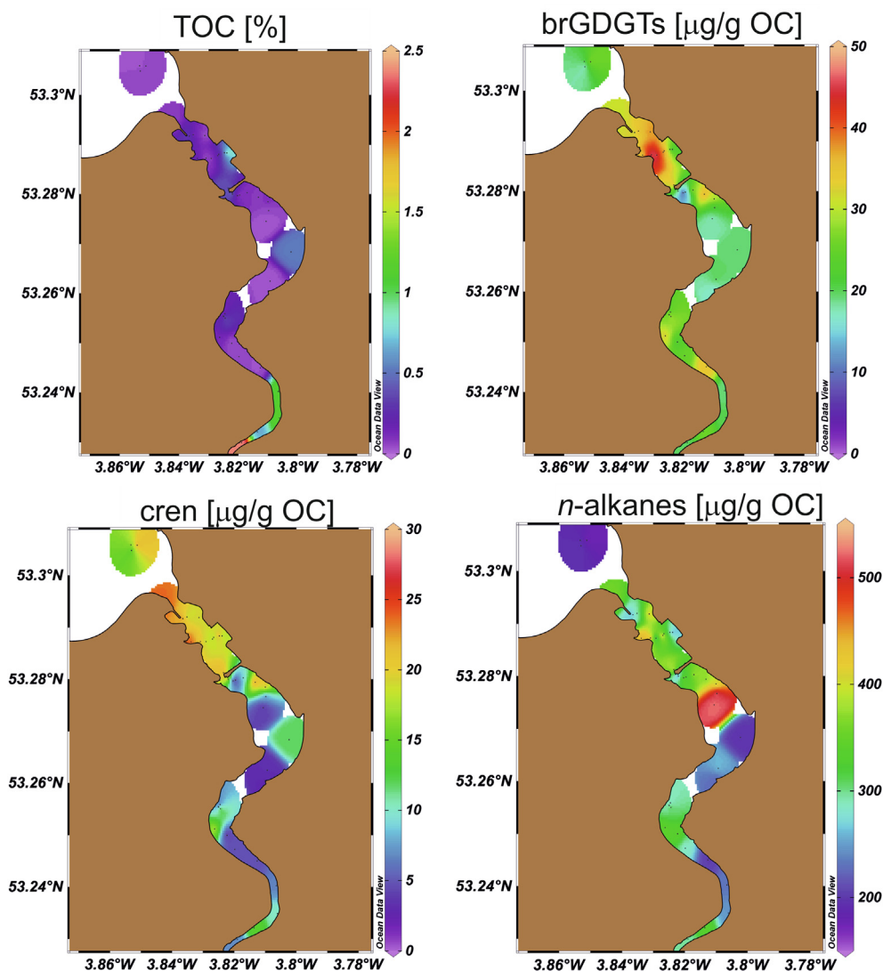
Fig. 6. Longitudinal distribution (from land to sea) of TOC and normalized concentrations ( \mu\text{g/g OC} ) of biomarkers along the Conwy Estuary.
