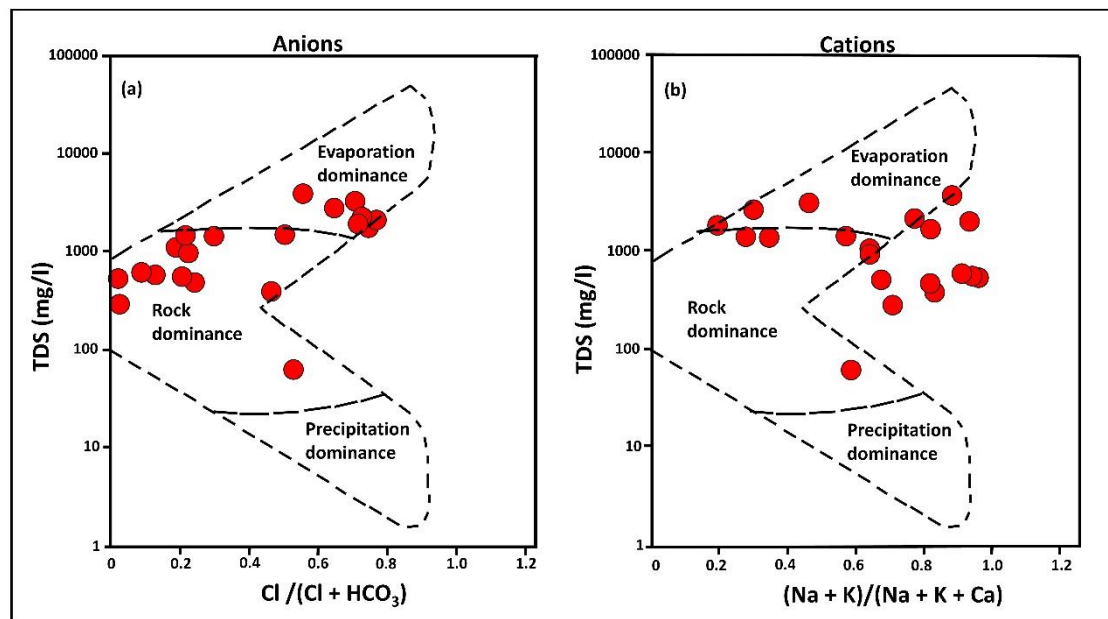
Figure 6. Gibbs plots showing (a) Total Dissolved Solids (TDS) vs. \text{Cl}/(\text{Cl} + \text{HCO}_3) and (b) TDS vs. \text{Na} + \text{K}/(\text{Na} + \text{K} + \text{Ca}) to illustrate the dominant processes governing groundwater chemistry in Makueni County.
