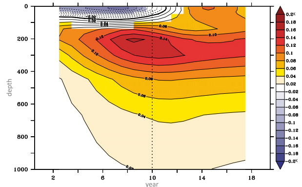
FIG. 2. Time series of ensemble mean global mean area-weighted temperature anomaly (K) with respect to the 140-yr control. Annual means are plotted, and a 4-yr boxcar filter is applied to smooth the data. Color shading indicates values that are significantly different from the control simulation at the 95% confidence level. The dotted vertical line separates the hiatus period (years 1–10; doubled vertical diffusivity) from the surge period (years 11–20; standard vertical diffusivity).
