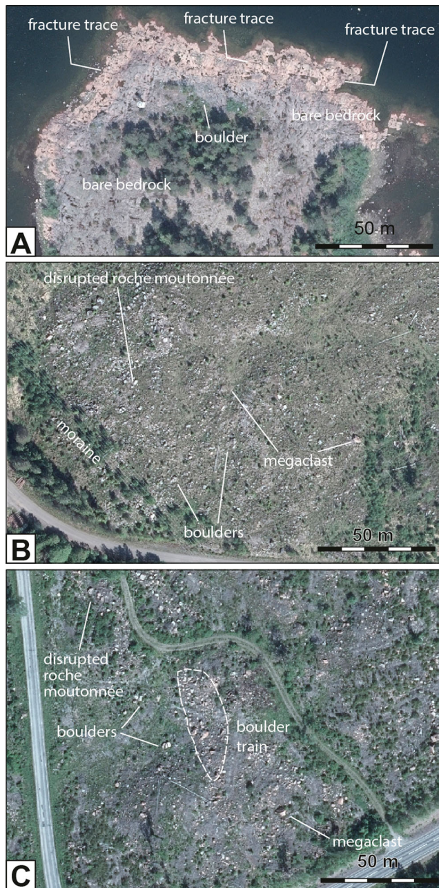
Figure 3. Contrasting rock surfaces without and with boulder spreads, showing the different density of boulders at the surface. Aerial photos from Lantmäteriet. (A) Abraded and plucked bedrock surface within weakly streamlined terrain and lacking in boulder spreads at Stånggrundet, c. 3 km east the Forsmark power station (Lat. 60.398645°N; Long. 18.222194°E). (B) Gunnarsbo boulder spread, c. 300 m west of the Forsmark power station (Lat. 60.402475°N; Long. 18.144887°E). (C) Boulder spread c 1 km SSE of Bladåker, near Lake Vällén (Lat. 59.991028° N; Long. 18.269045°E).
