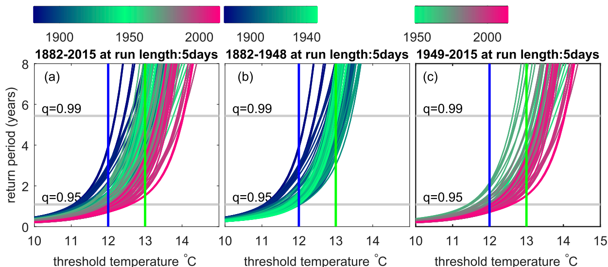
FIG. 2. Average return periods (ordinate) for runs of five consecutive days on which the daily maximum temperature is above a given threshold (abscissa). The curves are constructed from cdfs estimated from nine consecutive winter (DJF) seasons centered on each of the years 1882–2015. Equation (3) relates these cdfs to the return period for a warm spell of 5-day duration. Color indicates the sample central year in the time sequence: (a) all sample center years, (b) first half of the sample, and (c) second half of the sample. Horizontal lines indicate the 0.99 and 0.95 quantiles of each of the nine winter aggregate cdfs via Eq. (3). Vertical lines indicate 12° (blue) and 13°C (green).
