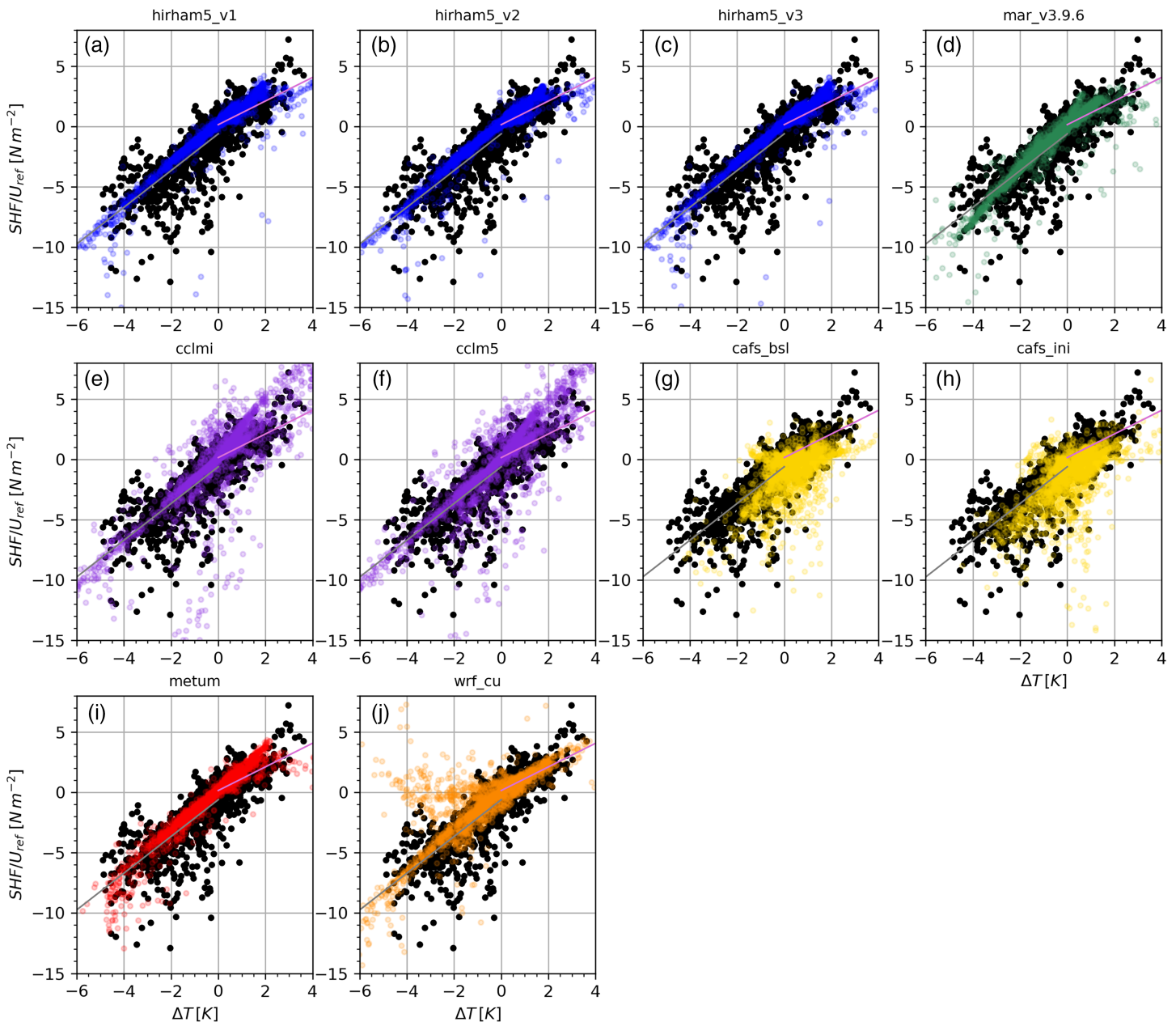
Figure 6. Covariability between the sensible heat flux ( SHF , W/m^2 ) weighted by the reference-level (10–12 m, depending on model) scalar wind speed ( U_{ref} , m/s) and the near-surface (10–12 m, depending on model) air temperature minus surface temperature difference ( \Delta T , K) for observations (black) and each regional climate model (colors, see title for model name). The gray line is the linear regression for the observations of scaled SHF for \Delta T < 0 K; the pink line is the linear regression for observations when \Delta T > 0 K. Statistics are valid for the full Arctic Clouds in Summer Experiment (ACSE) campaign, 5 July at 01:00 UTC through 3 October at 07:00 UTC.
