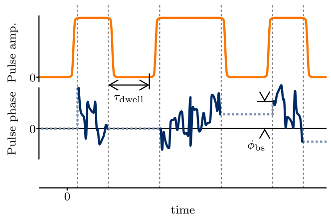
Figure 5. Illustration, not to scale, of an optimized interferometer sequence. Three pulses, as depicted in figure 4, are combined, with a time \tau_{\text{dwell}} between the light of one pulse turning off and the subsequent pulse turning on. Fringes are measured by measuring the fraction of atoms in the excited state at the end of the sequence as a function of a phase offset \phi_{\text{bs}} applied to the phase sequence for the final beamsplitter pulse.
