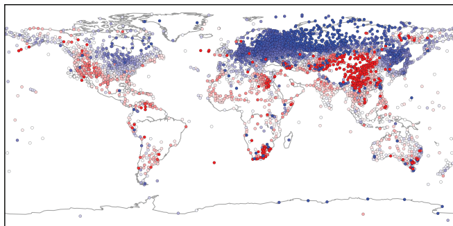
(a) 20CRv2c, 1960
