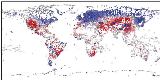
(c) 20CRv2c, 1980
