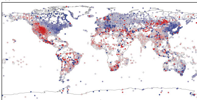
(f) 20CRv3, 2000
