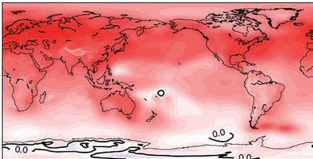
(b) 20CRv3
