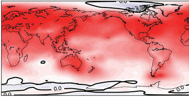
(b) 20CRv3
