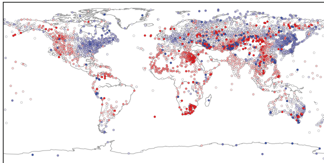
(b) 20CRv3, 1960
