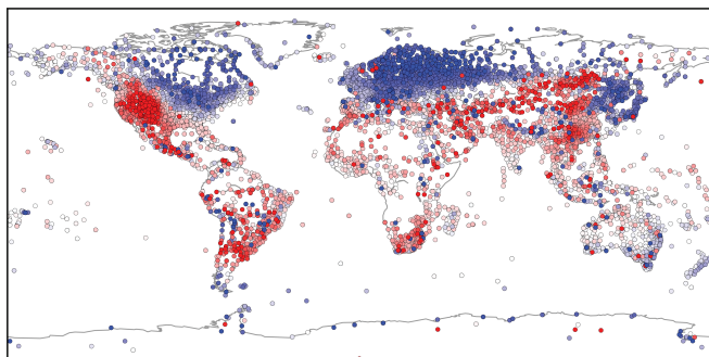
(e) 20CRv2c, 2000
