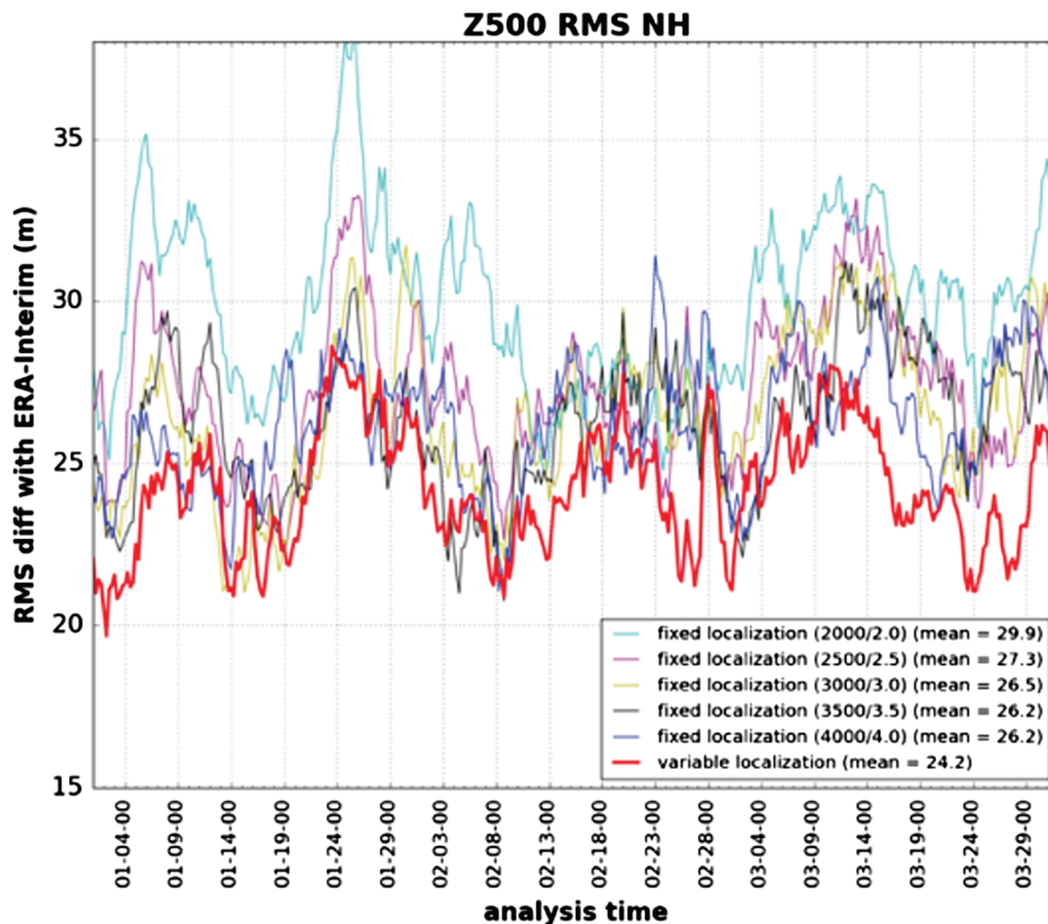
FIGURE D3 Time series of 500 hPa geopotential height error (relative to ERA-Interim reanalyses) for the experiments described in the text
