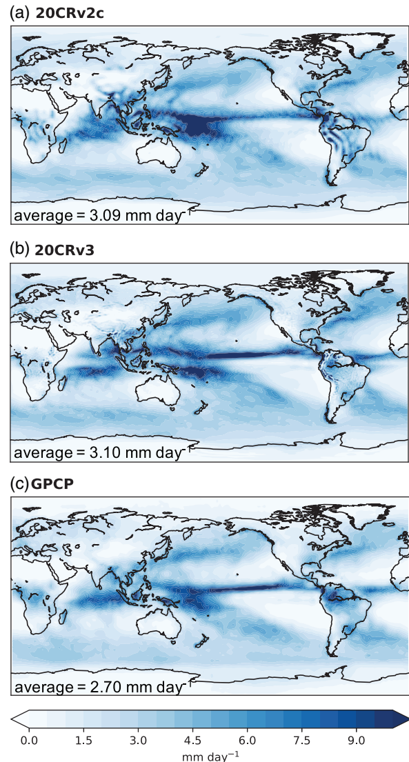
FIGURE 9 Maps of the year 2002 annually averaged forecasted precipitation rate (mm/day) in (a) 20CRv2c, (b) 20CRv3, and (c) the GPCP satellite/gauge blended fields
