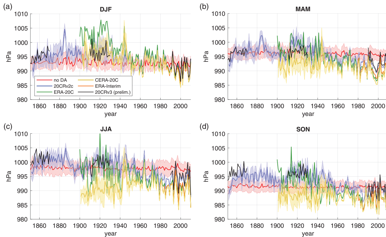
FIGURE 17 Time series of seasonal sea-level pressure poleward of 60^{\circ}\text{S} from 20CRv2c (blue), ERA-20C (green), CERA-20C (gold), ERA-Interim (orange), a non-assimilating model simulation using the 20CRv2c system (red), and preliminary 20CRv3 data without confidence intervals (black). Shading represents one ensemble standard deviation when available
