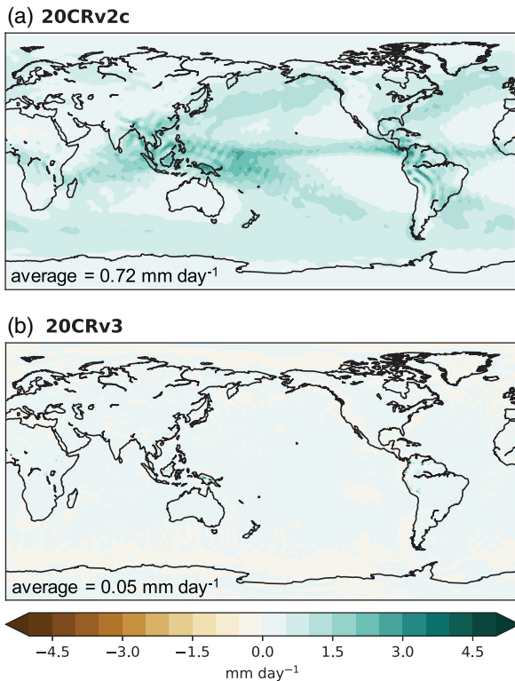
FIGURE 8 Maps of the year 2002 annually averaged differences (mm/day) between 3–6 hr forecasted precipitation rate and 0–3 hr forecasted precipitation rate in (a) 20CRv2c (which uses the digital filter) and (b) 20CRv3 (which uses the IAU instead of the digital filter). In a perfect system, these differences would be approximately zero
