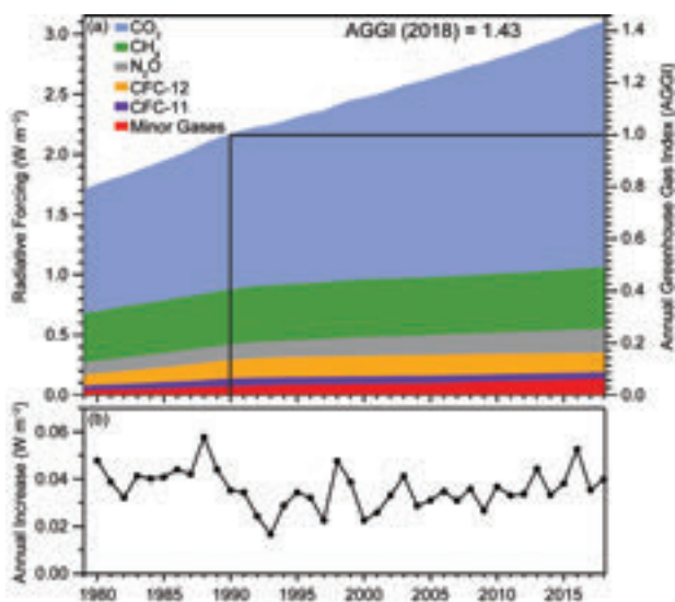
FIG. 2.46. (a) Direct radiative forcing (W m -2 ) due to 5 major LLGHG and 15 minor gases (left axis) and the associated values of the NOAA AGGI (right axis), and (b) annual increase in direct radiative forcing (W m -2 ). Solid black lines indicate that the AGGI had a value of 1.0 in 1990.
