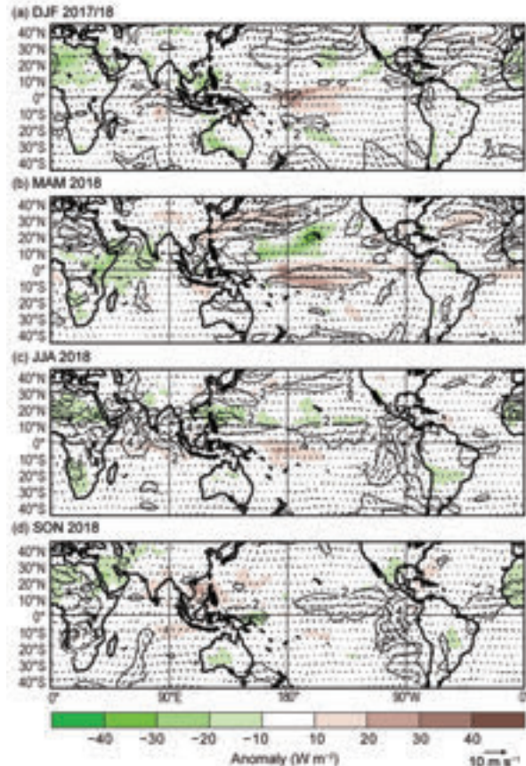
FIG. 4.4. Anomalous 850-hPa wind vectors and speed (contour interval is 2\text{ m s}^{-1} ), and anomalous OLR (shaded, \text{W m}^{-2} ), during (a) DJF 2017/18, (b) MAM 2018, (c) JJA 2018, and (d) SON 2018. Anomalies are departures from the 1981–2010 monthly means. Wind data are from the NCEP–NCAR reanalysis (Kalnay et al. 1996) and OLR are from AVHRR (Liebmann and Smith 1996).
