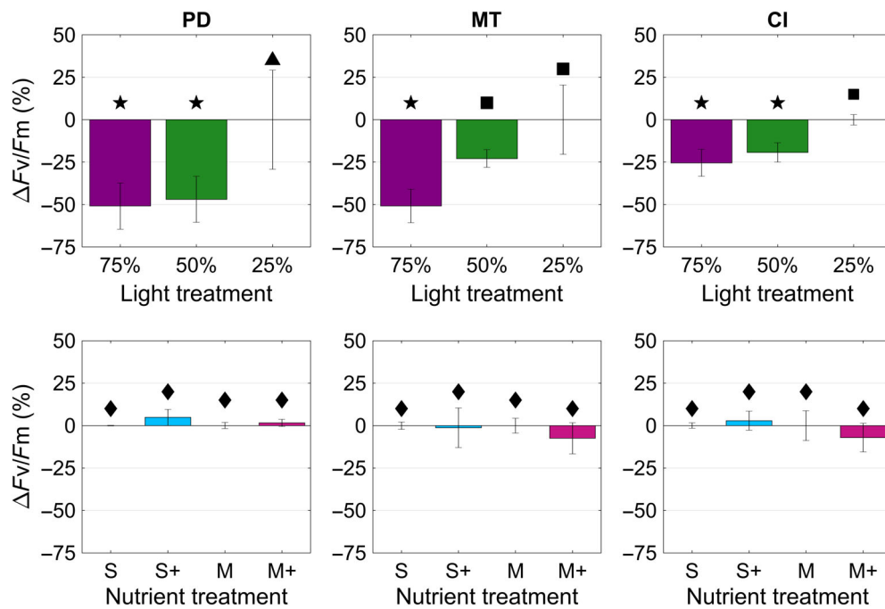
Fig. 7. Relative change (%) and standard deviation in photosynthetic efficiency ( \Delta F_v/F_m ) at T_f for PD (left), MT (middle), and canyon near CI (right) compared to T_i of the control treatment. Results shown for (top) light experiments, with treatments as percentage of surface irradiance (75%, 50%, and 25%) and where control is the lowest irradiance; (bottom) for nutrient experiments, where controls are shown as surface (S) and mix (M) with the corresponding iron addition treatments (S+ and M+). Different symbols denote treatments and timepoints that were found to be significantly different ( p < 0.05 ) within the same experiment and same region (each panel).
