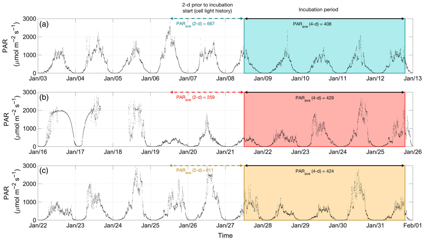
Fig. 2. Surface PAR ( \mu\text{mol m}^{-2} \text{s}^{-1} ) for the period preceding and during each experiment: (a) PD, (b) MT, and (c) region near CI. Incubation periods indicated by the colored box. Also reported are the Average incident PAR for the 2-d period prior to water collection (dashed colored arrow) which sets the phytoplankton light history and the 4-d average incident PAR (solid black arrow) which is used to calculate the light levels at each light treatment during incubation (Table 2).
