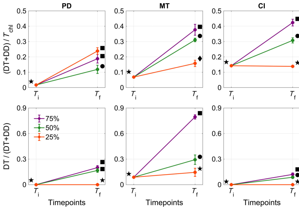
Fig. 6. Pigment ratios indicative of photoprotective strategies for the light treatments. Ratios involve diatoxathin (DT), diadinoxanthin (DD), and/or total chlorophyll ( T_{chl} ), at initial setup ( T_i ) and after 4 d ( T_f ) for PD (left), MT (middle), and canyon near CI (right). Light treatments are shown as the percentage of surface irradiance (75%, 50%, and 25%). Different symbols denote treatments and timepoints that were found to be significantly different ( p < 0.05 ) for the same ratio and same region (each panel).
