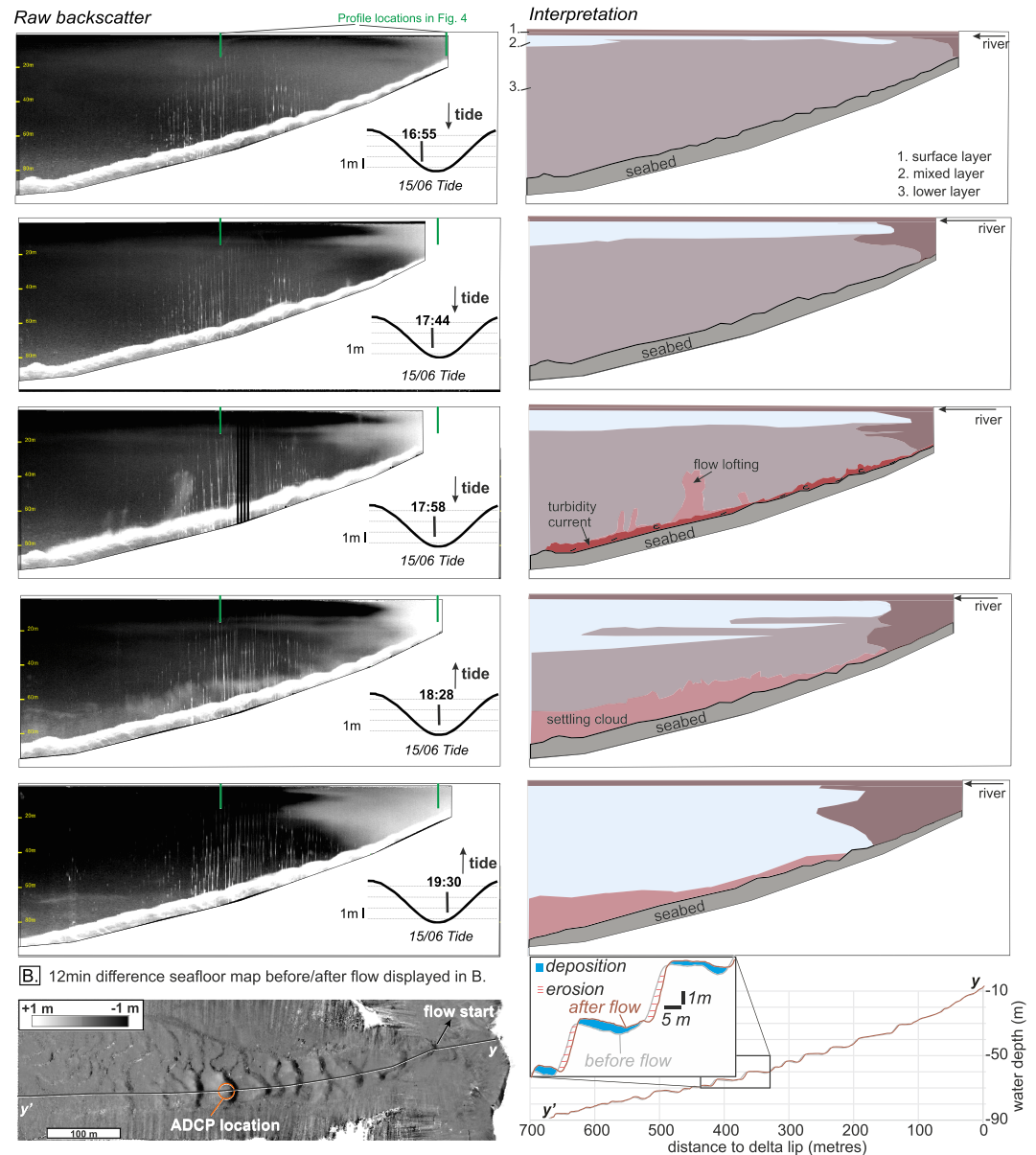
Figure 5. (a) Left column: Five water column transects imaged by a 500-kHz M3 echosounder on 15 June 2015 along profile track shown in Figure 2c. Right column: Interpretation and transects timing according to tides. (b) Difference map between seafloor morphology 12 min before/after the turbidity current. The turbidity current caused up to 2 m of erosion and up to 1 m of deposition.
