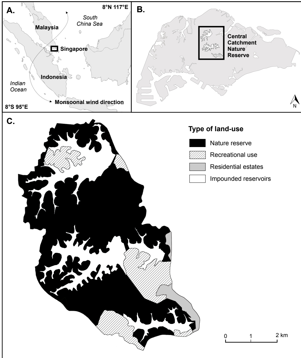
Figure 2. Geographical location of the study site. A. Map of Singapore and its neighbouring countries, Malaysia and Indonesia, along with the general wind flow patterns in the region during the northeast and southwest monsoons. B. Relative position of the Central Catchment Nature Reserve on the mainland of Singapore. C. Land-use and catchment map of the Central Catchment Nature Reserve.
