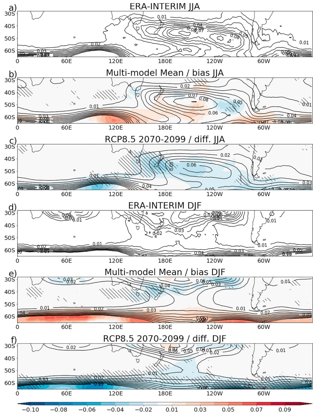
Figure 3. Blocking frequency biases and future projections in the Southern Hemisphere for winter (a–c) and summer (d–f): (a, d) The ERAI mean blocking frequency for each gridpoint; (b, e) the mean of all CMIP5 models for the historical experiment (contours) minus ERAI (colors); (c, f) the mean of all CMIP5 models for the RCP 8.5 scenario from 2070–2099 (contours) minus the historical experiment (colors). The contour interval for all plots is 0.01, and hatching indicates that 80% of models agree on the sign of the difference. The blocking frequency is given as the fraction of blocked days. CMIP5 = Coupled Model Intercomparison Project Phase 5; JJA = June–August; ERAI = ERA-Interim; DJF = December–February.
