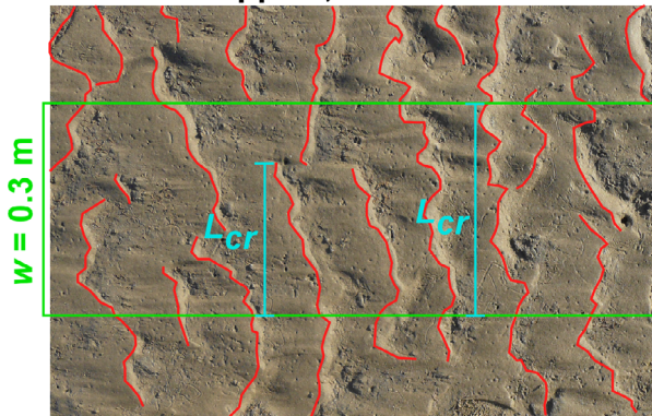
Bed 7: 2D ripples, 24.7% mud
