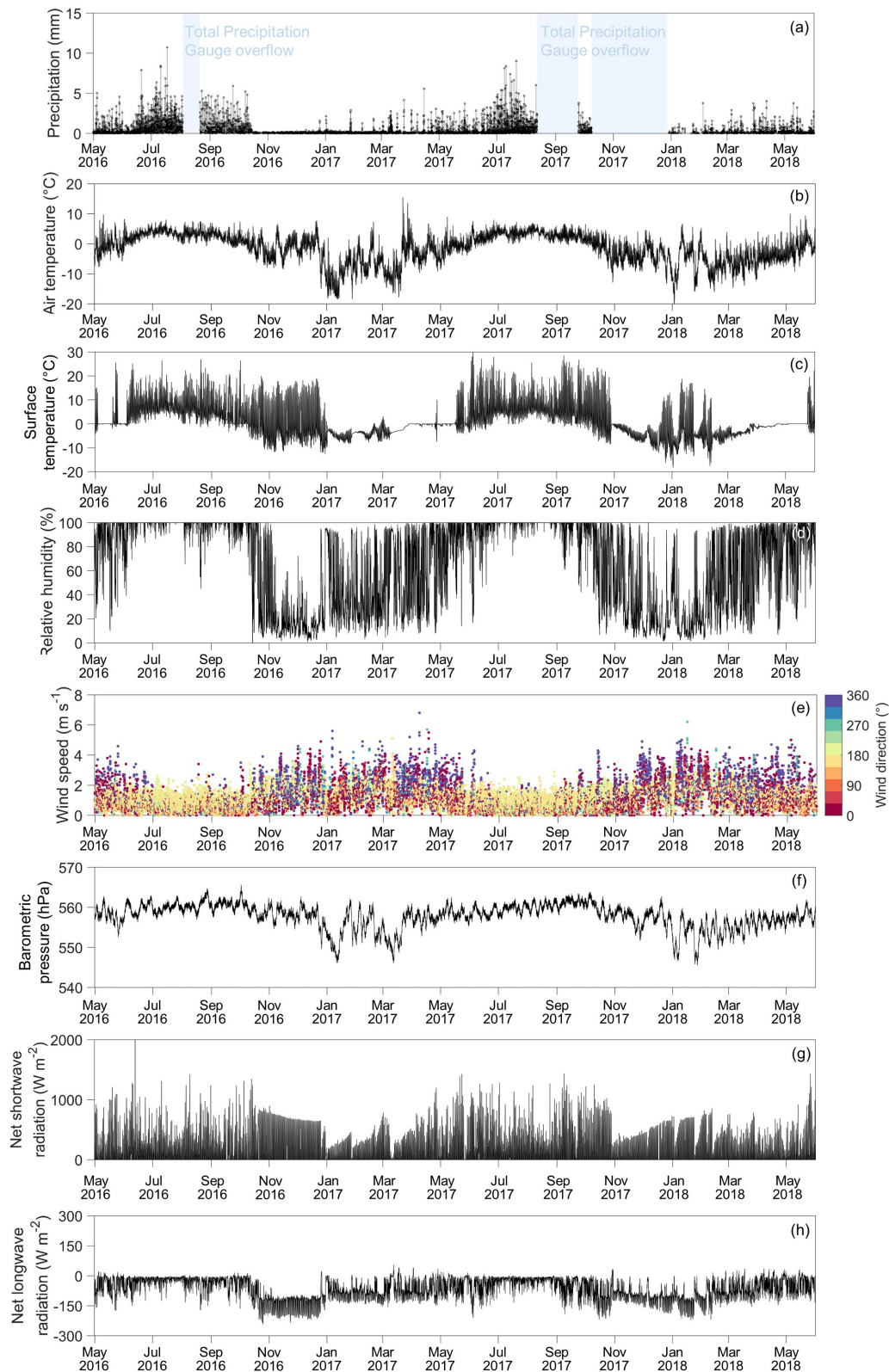
FIGURE 3 | Hourly meteorological data measured by the automatic weather station between May 2016 and June 2018. (a) Precipitation from the Total Precipitation Gauge, (b) air temperature, (c) surface temperature, (d) relative humidity, (e) wind speed and direction, (f) barometric pressure, (g) net shortwave radiation and (h) net longwave radiation.
