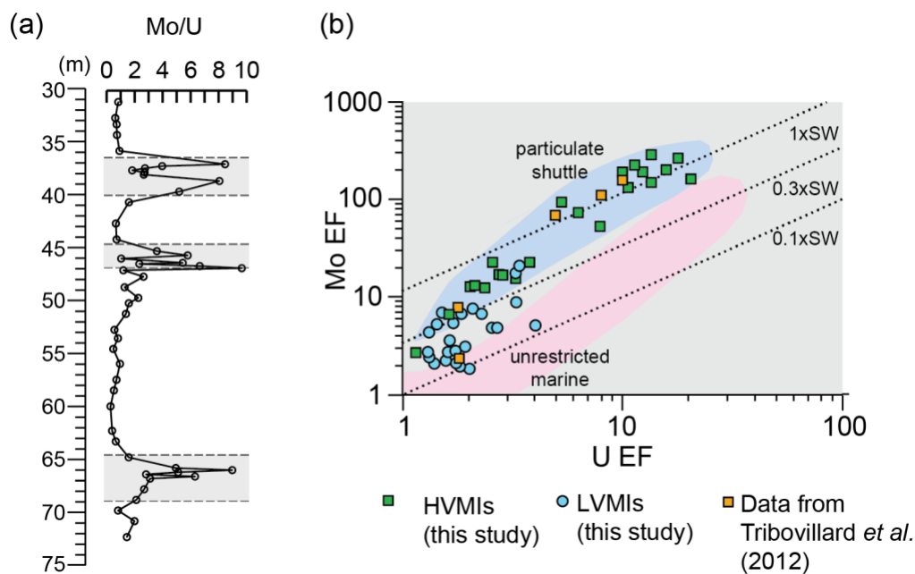
5 Figure 8: a) Depth plot Mo/U (ppm/ppm) (after Algeo and Tribovillard (2009)). Grey panels depict the higher variability mudstone intervals (HVMI) defined in this study, b) scatter plot of Mo EF versus U EF calculated relative to Post Archean Average Shale (PAAS; Taylor and McLennan (2001)(after Tribovillard et al., 2012). Lower variability mudstone interval (LVMI) samples are indicated by blue circles, HVMI are indicated by green squares. Data from the Eberston core by Tribovillard et al., (2005) are represented by orange squares. Dashed lines are modern day seawater, 0.3 x modern day seawater and 0.1 x modern day seawater values shown for reference. The particulate shuttle is mapped in blue and unrestricted marine setting is mapped in pink. Axes are logarithmic.
