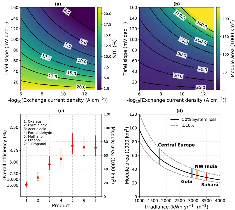
Figure 1. Theoretical efficiency limits and module area for the -10\text{Gt CO}_2\text{ yr}^{-1} scenario. (a) STC efficiency limit of a dual-junction absorber for formic acid (without system loss) as a function of exchange current density and Tafel slope. (b) Resulting module area at Sahara irradiance and 50% system loss. (c) STC efficiency and module area required under Sahara irradiance for a selection of products at 50% system loss. Error bars indicate 40% and 60% loss, respectively. (d) Module area for formic acid production over the yearly irradiance at 50% (solid line), as well as 40% and 60% (dashed lines) system loss. Vertical lines mark typical irradiances accessible to a two-axis tracker.
