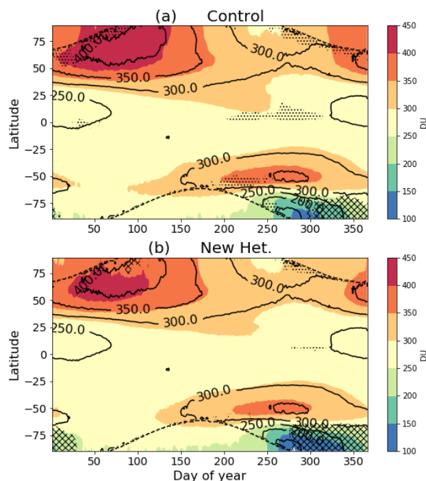
Figure 4. Zonal mean total column ozone climatology (1996–2009, excl. 2002) of the (a) control and (b) “New Het.” runs. Contours show the NIWA-BS data, crosshatching/stippling indicates where the model under/overestimates NIWA-BS data by more than 30 DU. Dashed contours mark the absence of NIWA-BS data.
