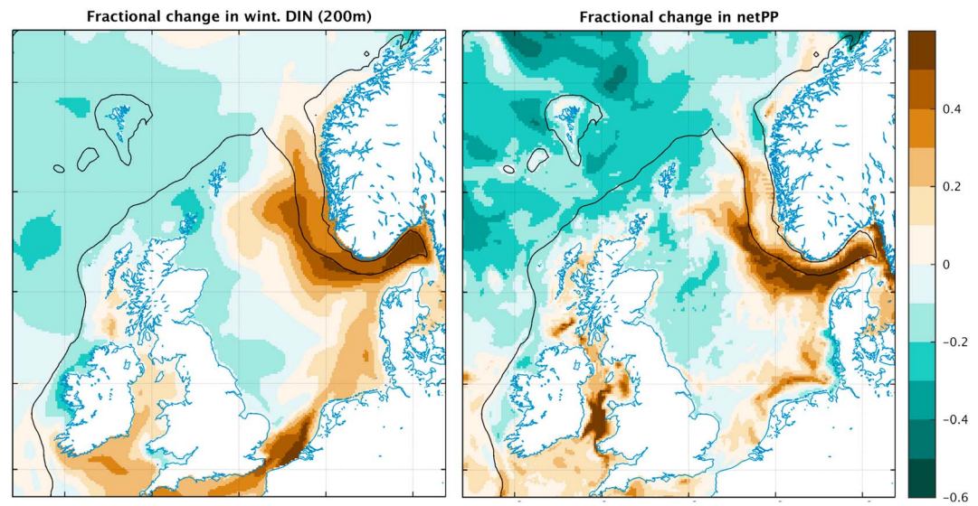
Figure 4. Fractional change (future/present-1) of winter dissolved inorganic nitrogen (DIN) and annual net primary production (netPP) from the ERSEM ecosystem model in E1.
