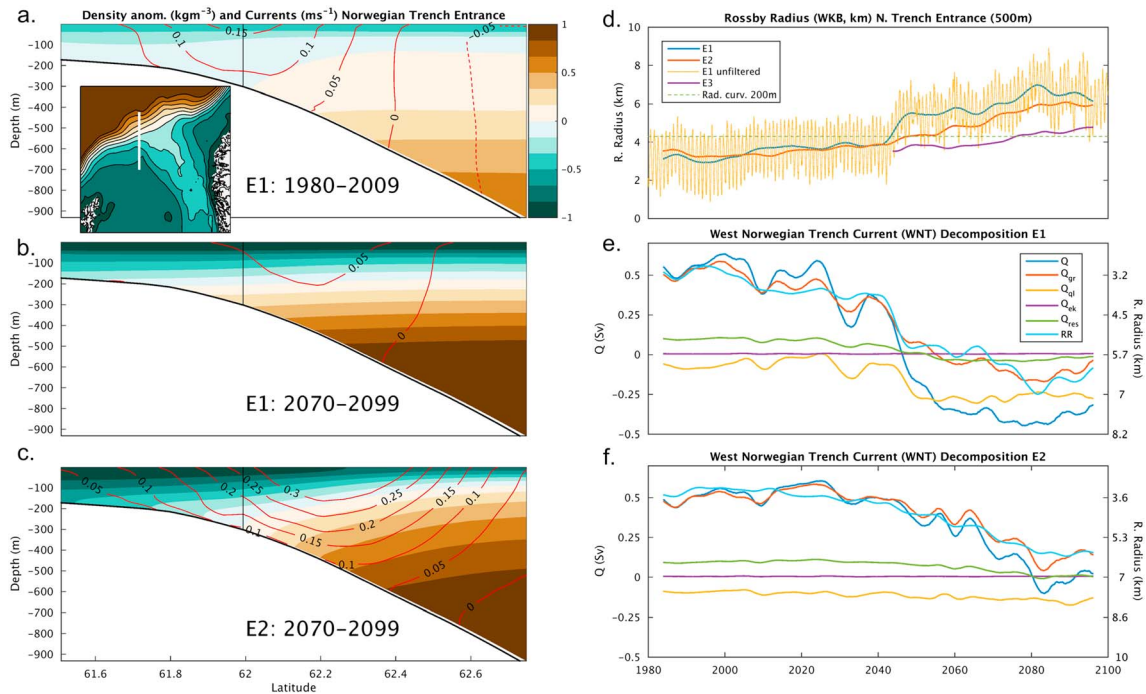
Figure 3. Latitude-depth cross sections of density anomaly (colors) and velocity (contours) at the entrance to the Norwegian Trench in E1: present (a) and future (b) and E2: future (c). The vertical line indicates the depth of the deepest isobath that turns the corner to enter the Norwegian Trench. The insert shows isobaths at this entrance and the location of this section. The inflow is diagnosed using time series (d) of Rossby radius (first baroclinic, estimated from WKB approximation; Chelton et al., 1998) at the 500-m isobath for E1, E2, and E3 and the geostrophic decomposition (equation (2)) for E1 (e) and E2 (f), filtered as in Figure 2.
