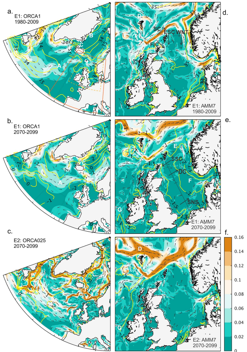
Figure 1. Depth mean currents (0 to 200 m) from the two driving global NEMO models (a–c) and downscaled results (d–f) for a subregion (dashed box in a) of the regional model (solid in a, and Figure S1). Colors show speed ( \text{ms}^{-1} ), and arrows show direction. Top figures show mean present-day conditions; center (E1) and bottom (E2) show mean end-of-century conditions. Yellow contours in (a) and (d) show surface salinity, and in (b), (c), (e), and (f) show the salinity differences between future and present. (d) and (e) also show the sections used for time series and geostrophic analysis (Figures 2 and 3), with arrows indicating the direction of positive transport. SC = slope current; ESC = East Shetland Current; WNT = West Norwegian Trench Current; FIC = Fair Isle Current; DC = Dooley Current; SNS = southern North Sea Current.
