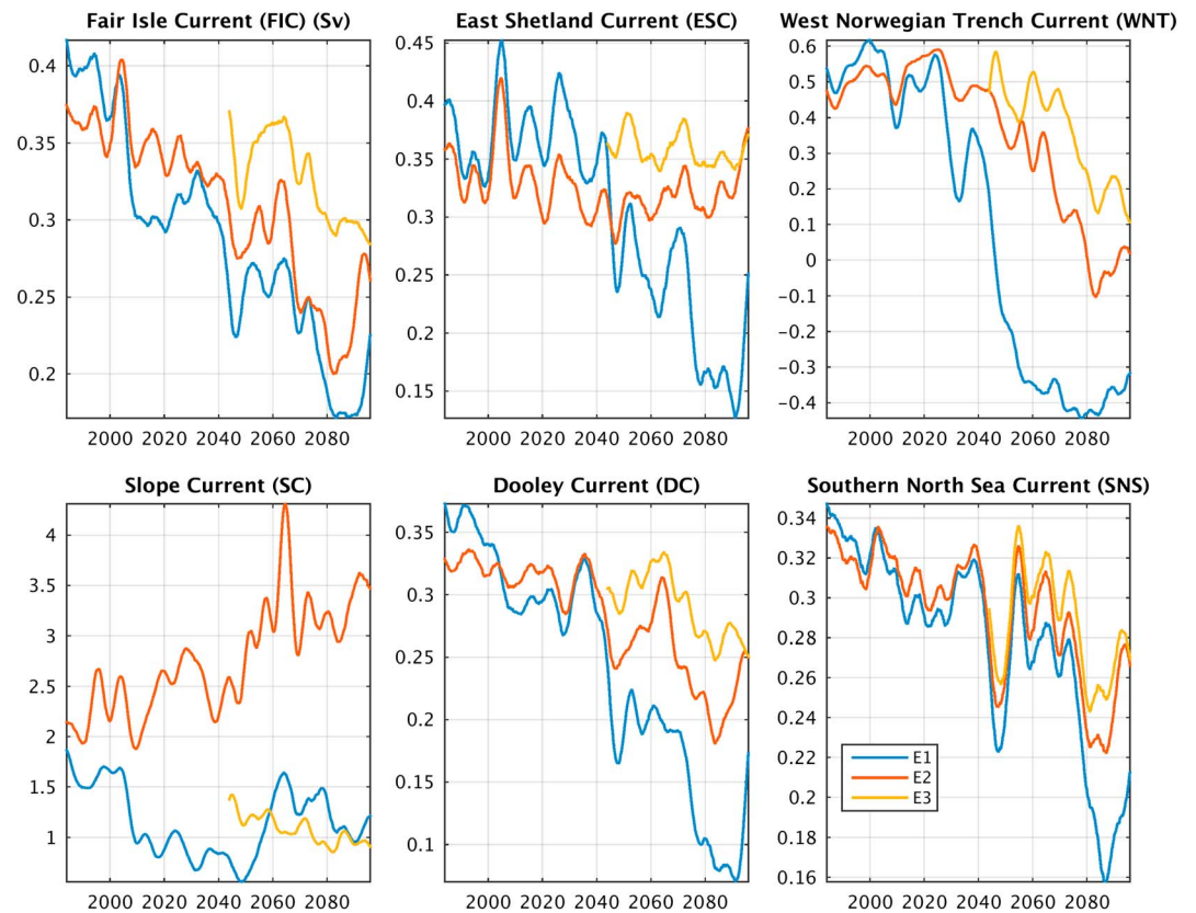
Figure 2. Time series of volume transport (Sv) for six sections in Figure 1. Monthly data is Gaussian filtered, \sigma = 2 years. Experiment E3 is restarted from E1 at 2040 with ocean boundary conditions taken from 1980 to 2009.
