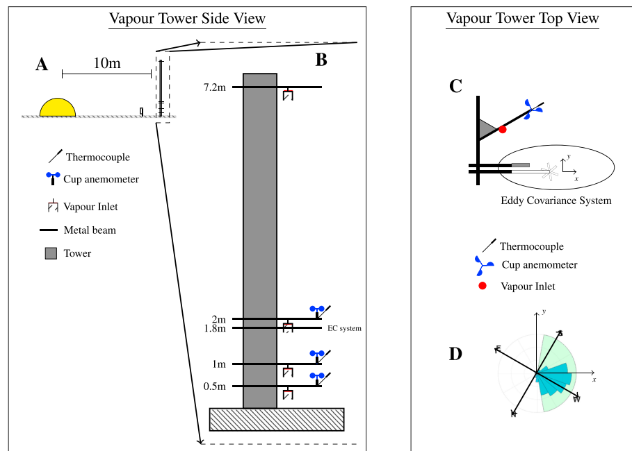
Figure 1. Schematic overview of the field site and instrument configuration. Side view: (a) Position of the tent, CR3000 micrologger, and vapor tower. The prevailing wind is approximately from right to left (see d). Vertical discretization of the model domain representation the lower boundary in contact with the snow surface. (b) Approximate position of vapor inlets, cup anemometers, fine-wire thermocouples, and the eddy covariance system. Top view: (c) Relative position of vapor inlets, cup anemometers, thermocouples, and eddy covariance instruments on each beam. A KH20 hygrometer and CSAT3 ultrasonic anemometer comprise the eddy covariance system. Note that instruments are not drawn to scale. The x - y coordinate system is the internal coordinate system of the ultrasonic anemometer. (d) The wind rose observed by the ultrasonic anemometer (10-min averages) where directions are given both with respect to the orientation of the anemometer ( x - y coordinate system) and the approximate north-south compass (N-S, E-W). The green wedge indicates the angles within 80^\circ of the x axis of the CSAT3.
