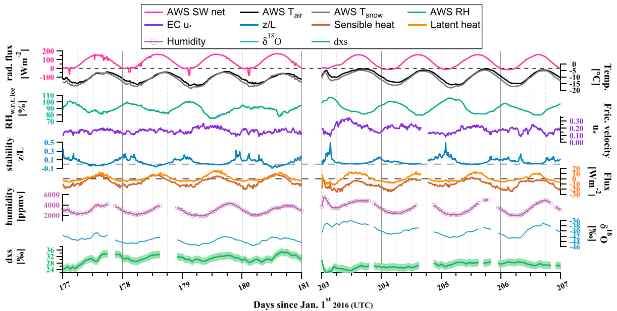
Figure 2. (left) June period (DOY 177–181, 25–29 June). (right) July period (DOY 203–207, 21–25 July). From above: Program for Monitoring of the Greenland Ice Sheet automatic weather station (AWS) observations of net incoming shortwave (SW) radiation, air and snow surface temperature, and relative humidity (RH) with respect to ice. Eddy Covariance observations of friction velocity, atmospheric stability ( z/L ) evaluated at a height of 1.8 m, and turbulent sensible and latent heat flux. Specific humidity, \delta^{18}\text{O} , and dxs measured by the CRDS at 2 m above the snow surface. The shading on both \delta^{18}\text{O} and dxs indicates one measurement uncertainty. DOY = day of year.
