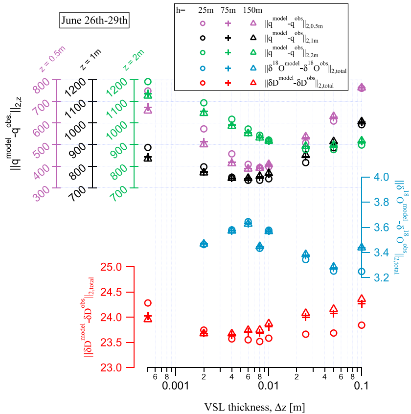
Figure 4. June period model-data misfit dependency on the thickness of the viscous sublayer (VSL) \Delta z for three different values of h : 25 (circles), 75 (crosses), and 150 m (triangles). (top) Humidity misfit for each individual level; the misfit at the 0.5-m level (purple) is consistently smaller than that at the 1- (black) and 2-m (green) levels. (middle) Total \delta^{18}\text{O} model-data misfit (blue). (bottom) Total model-data misfit for \delta\text{D} (red).
