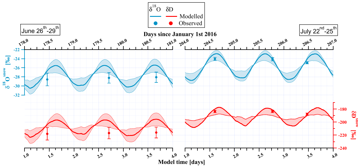
Figure 6. Snow isotopic composition using the ice-vapor fractionation coefficient from Ellehoj et al. (2013), assuming equilibrium fractionation in the viscous sub-layer. (left) June period. (right) July period. For each period, three observations of snow isotopic composition are also shown. The standard deviation ( \sigma_{\text{snow}} ) on the mean observed snow isotopic composition is comparable to the marker size for the July period.
