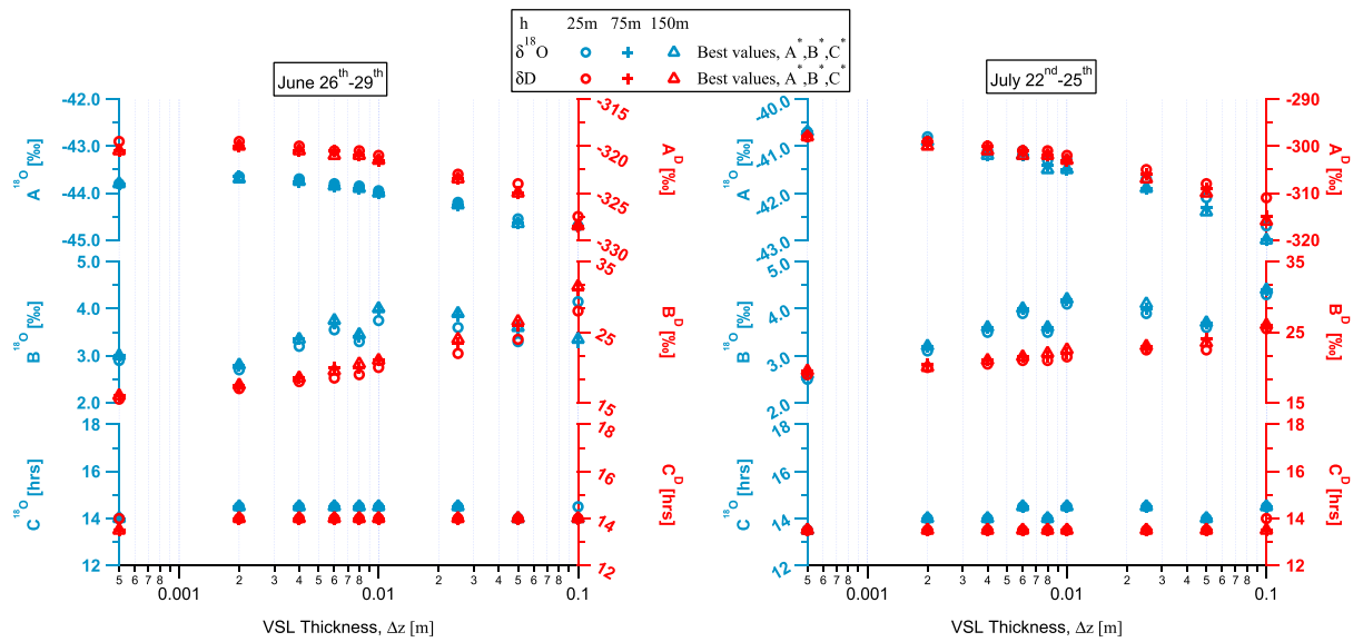
Figure 3. Values of the coefficients A^* , B^* , and C^* in equation (4) for different combinations of viscous sublayer (VSL) thickness ( \Delta z , x axis) and atmospheric boundary layer height ( h , symbols—see key), shown for both (blue) \delta^{18}\text{O} and (red) \delta\text{D} producing the best fit to the observations. (left) June period. (right) July period.
