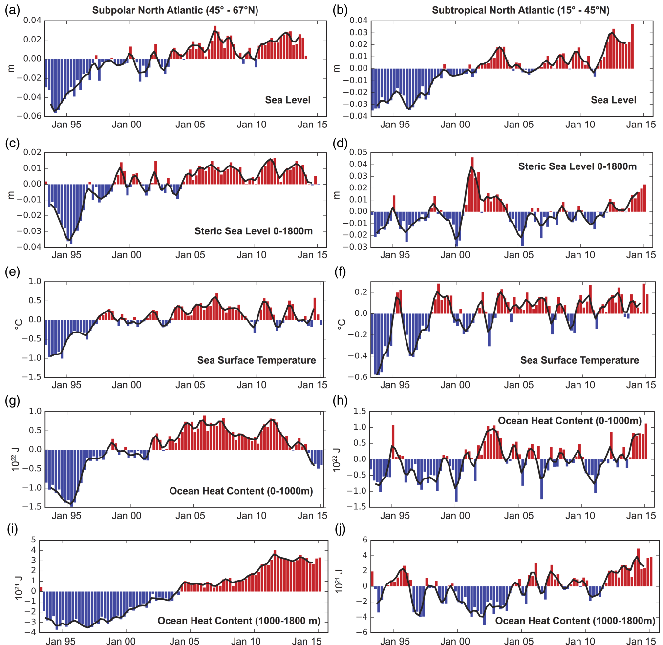
FIGURE 12 Time series of North Atlantic subpolar (left column) and subtropical (right column) sea level, SST and ocean heat content anomalies. (a,b) Sea level change (m), and (c,d) Steric sea level change (m), all anomalies from 1993 to 2014 mean seasonal means. (e,f) SST anomalies from the 1993 to 2014 seasonal means. (g,h) A 0–1,000 m ocean heat content anomaly from 1993 to 2015 seasonal mean and (i,j) Same except 1,000–1,800 m. Sea level and SST data are from the ESA-CCI project (Hollmann et al. , 2013; Merchant et al. , 2014; Ablain et al. 2015, 2017). Heat content anomalies derived from EN4 data sets (Good et al. , 2013) ( www.metoffice.gov.uk/hadobs/en4/ ) [Colour figure can be viewed at wileyonlinelibrary.com ]
