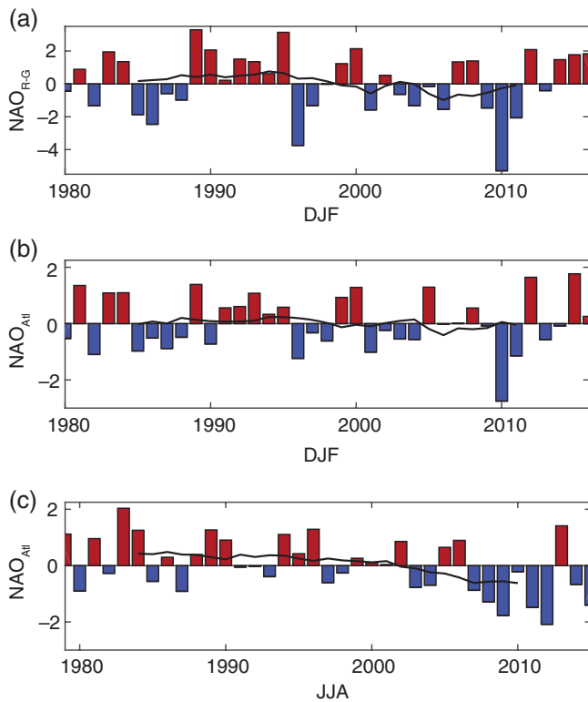
FIGURE 1 (a) NAO index estimated from the normalized difference of surface pressures at Reykjavik and Gibraltar. Each of the surface pressure time series is normalized by their respective standard deviation (SD), so the index is dimensionless. (b) DJF Atlantic NAO index estimated as the surface pressure principal component time series over the region 60^{\circ} – 0^{\circ} W, 30^{\circ} – 70^{\circ} N. The principal component time series is normalized by its SD, so the index is dimensionless. (c) JJA Atlantic NAO index otherwise as (b). All plots: The bars indicate the seasonal mean values and the thick black line indicates an 11-year running mean [Colour figure can be viewed at wileyonlinelibrary.com ]
