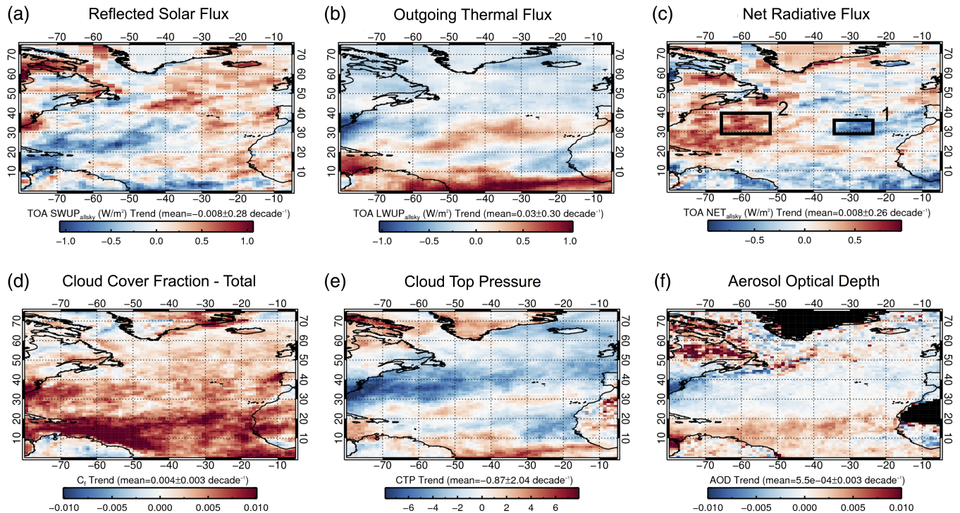
FIGURE 9 Trends in the anomalies computed from the monthly mean top of atmosphere (a) outgoing shortwave, (b) outgoing longwave, and (c) net radiative flux computed using All-sky monthly mean CERES-EBAF during the period 2006–2016 over the North Atlantic region (note positive is a net downwards flux in c). The MODIS MOD08_M3 product also displays (d) All-sky cloud cover fraction, (e) cloud top pressure and (f) AOD. Trends are computed using the period 2006–2016 over the North Atlantic region. Two boxes are displayed showing regions with substantial cooling (box 1 in the East Atlantic) and warming (box 2 in the West Atlantic). Mean trends of the anomalies are reported as a change per decade. Regions in black contain missing data [Colour figure can be viewed at wileyonlinelibrary.com ]
