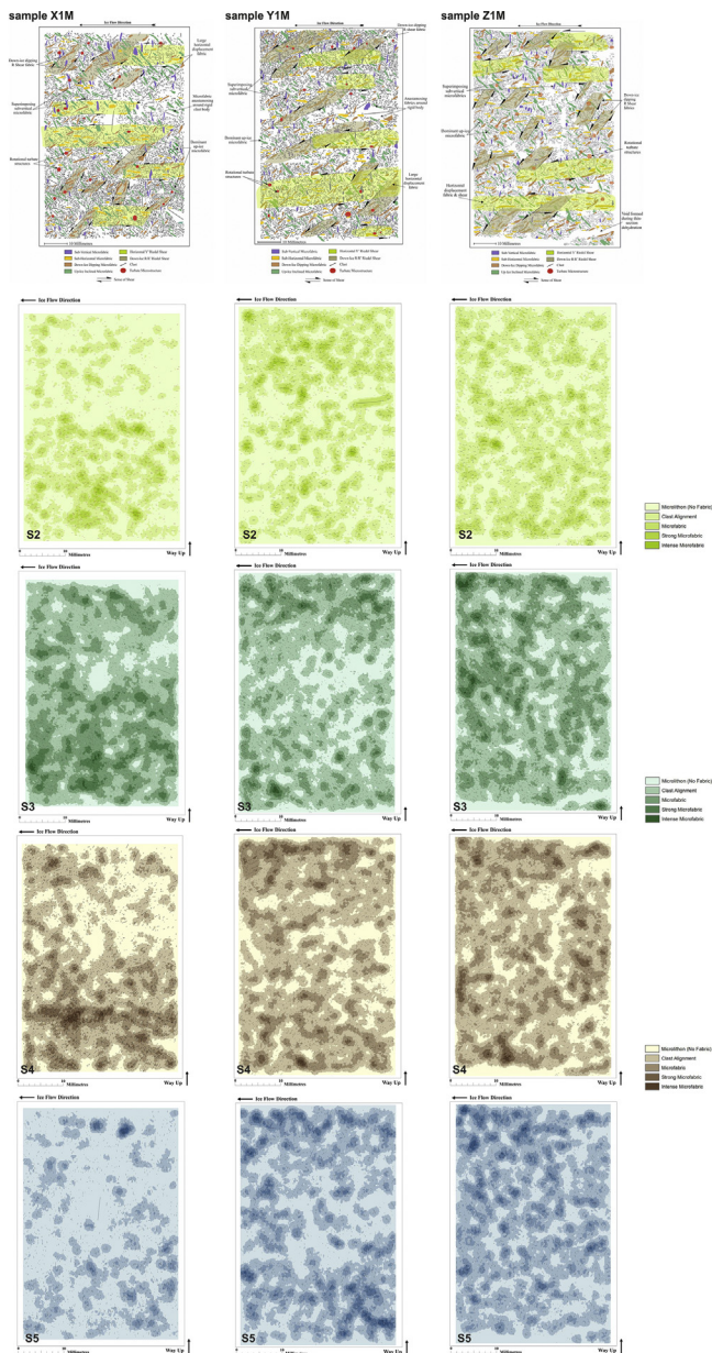
Fig. 8. Microstructural maps and automated clast density maps of the main clast microfabrics (S2, S3, S4, S5) identified within samples X1M, Y1M and Z1M.
