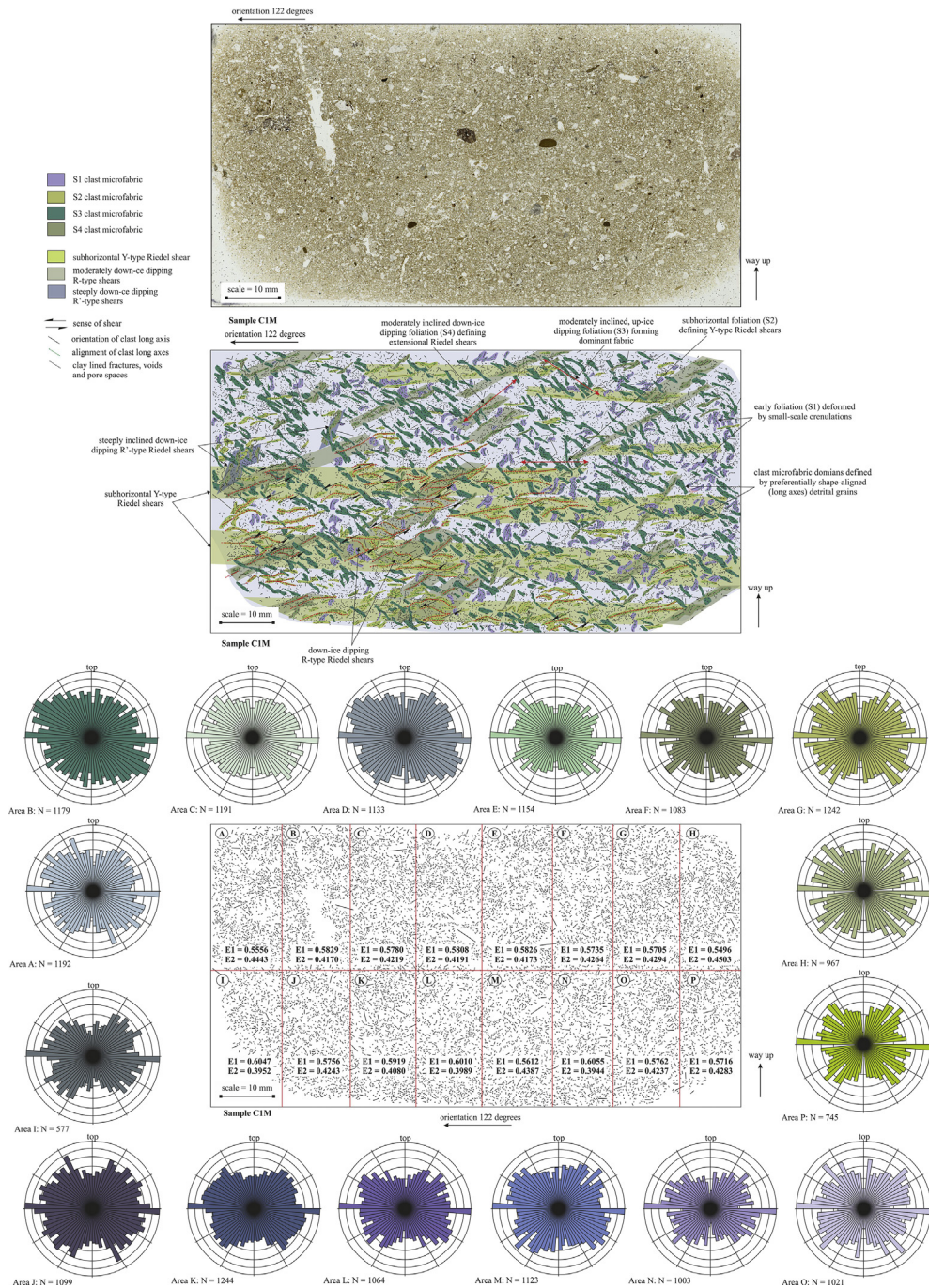
Fig. 2. Microstructural map and high resolution scan of thin section C1M. The orientation of the long axes of sand to granule sized clasts included within the diamicton are shown on a series of rose diagrams. The thin section has been subdivided into 16 subareas and the E1 and E2 eigenvalues calculated for each area (see text for details).
