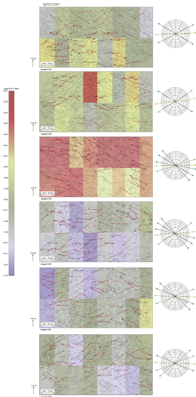
Fig. 13. Variation in E1 eigenvalues calculated for the thin sections (C1M to C6M) showing the variation in relative fabric strength both with an individual thin section and vertically through the diamicton at site C. Red colours represents areas of the thin sections with higher E1 values (0.65–0.68) and purple low E1 values (0.53–0.51). (For interpretation of the references to colour in this figure legend, the reader is referred to the Web version of this article.)
