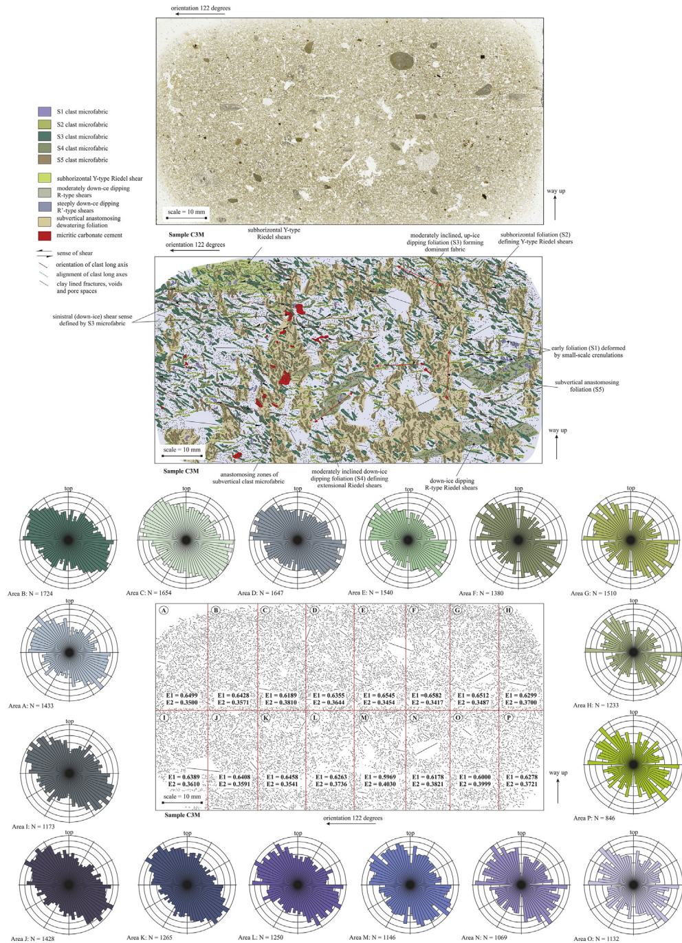
Fig. 4. Microstructural map and high resolution scan of thin section C3M. The orientation of the long axes of sand to granule sized clasts included within the diamicton are shown on a series of rose diagrams. The thin section has been subdivided into 16 subareas and the E1 and E2 eigenvalues calculated for each area (see text for details).
