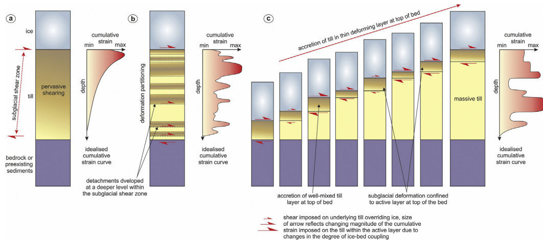
Fig. 17. Schematic profiles through the bed of a glacier and the resulting idealised cumulative strain curves: (a) Pervasive deformation throughout the subglacial shear zone with the amount of strain increasing upwards towards the ice-bed interface; (b) Deformation partitioning within the subglacial shear zone with localised detachments forming at deeper levels within the bed; and (c) Deformation confined to the “active” layer located at the top of the bed with shearing migrating upwards keeping pace with till accretion (cf. Larsen et al., 2004).
