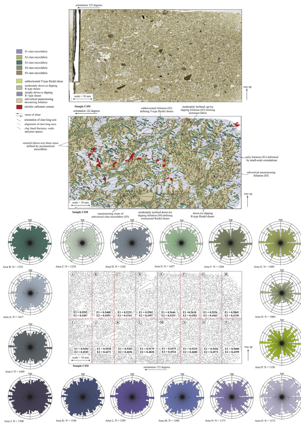
Fig. 5. Microstructural map and high resolution scan of thin section C4M. The orientation of the long axes of sand to granule sized clasts included within the diamicton are shown on a series of rose diagrams. The thin section has been subdivided into 16 subareas and the E1 and E2 eigenvalues calculated for each area (see text for details).
