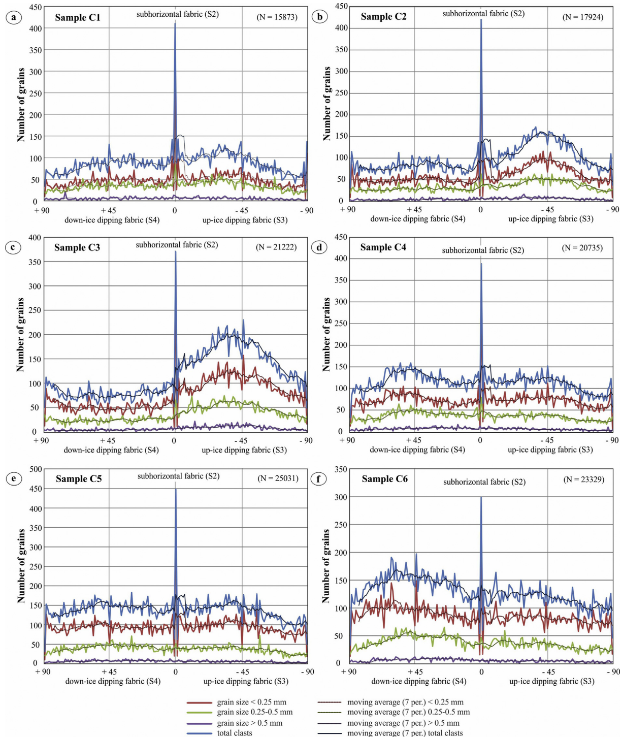
Fig. 11. Graphs showing the effects of grain size on clast microfabric development within the diamicton at site C. The long axis data for each thin section (C1M to C6M) are divided into three sets: (i) grains < 0.25 mm in length; (ii) grains between 0.25 and 0.5 mm in size; and (iii) grains over > 0.5 mm in length. The number of grains in each of the three classes is plotted against the orientation of their long axis ( 0^\circ represents horizontal). The large “spike” in the data set for the finest grains and total clasts at 0^\circ results from the unavoidable “snapping” to the horizontal of short long axes dipping at very low angles ( -2^\circ to +2^\circ ) during digitisation using CorelDraw. On Fig. 12 the data are plotted on a series of rose diagrams showing the dip of the long axes within the 2D plane of the thin section.
