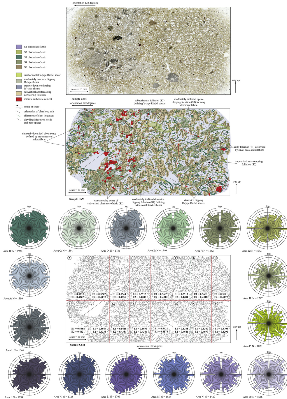
Fig. 7. Microstructural map and high resolution scan of thin section C6M. The orientation of the long axes of sand to granule sized clasts included within the diamicton are shown on a series of rose diagrams. The thin section has been subdivided into 16 subareas and the E1 and E2 eigenvalues calculated for each area (see text for details).
