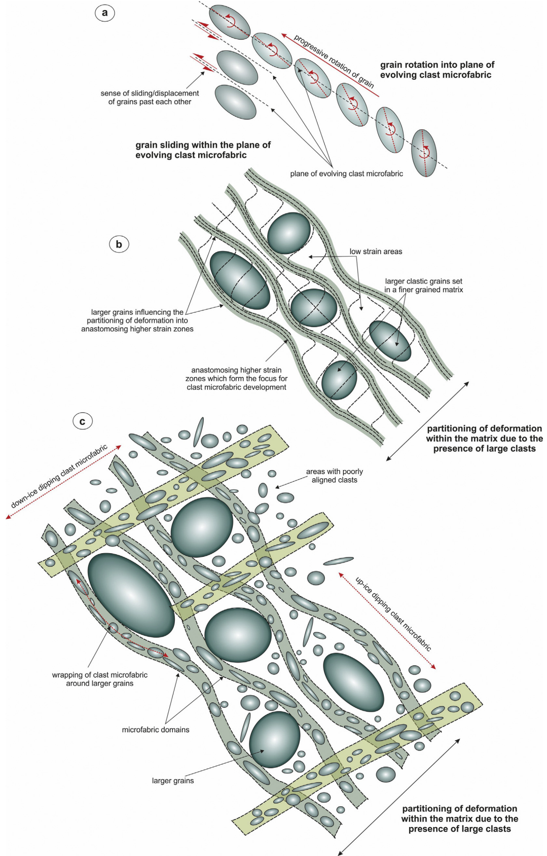
Fig. 16. (a) Cartoon showing the passive rotation of elongate clasts into the plane of the developing microfabric. Further deformation of clasts aligned within this fabric is thought to occur in response to grain sliding; (b) Strain field diagram modified from Bell et al. (1986) used here to show the proposed geometry of the strain field formed in response to the presence of large immobile clasts within a weaker deforming matrix; and (c) Schematic diagram showing the development of anastomosing clast microfibrils within a till defined by the preferred shape alignment of finer grained clasts. The spacing of the microfabric domains is controlled by the grain size and spacing of the larger sand to pebble sized clasts in response to deformation partitioning within the till.
