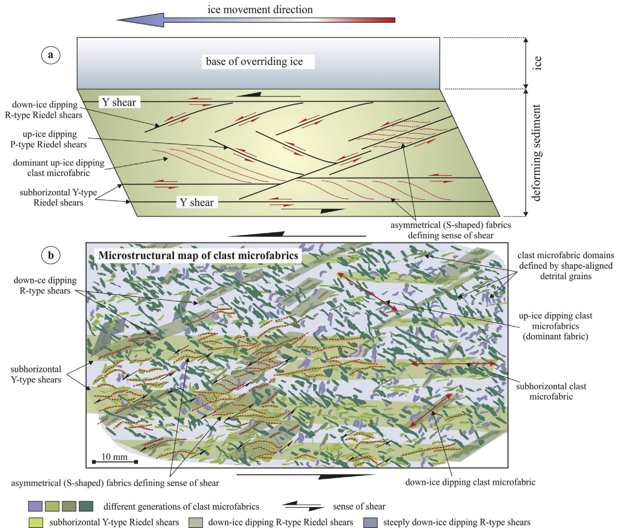
Fig. 10. (a) Diagram showing the relationships between the different sets of Riedel shears developed within the diamicton in response to deformation imposed by the overriding ice stream; and (b) Example of a detailed microstructural map of sample C1M. The coloured polygons represent the different generations of clast microfabrics, which define the Riedel shears, subhorizontal shear fabric and up-ice dipping foliation.
