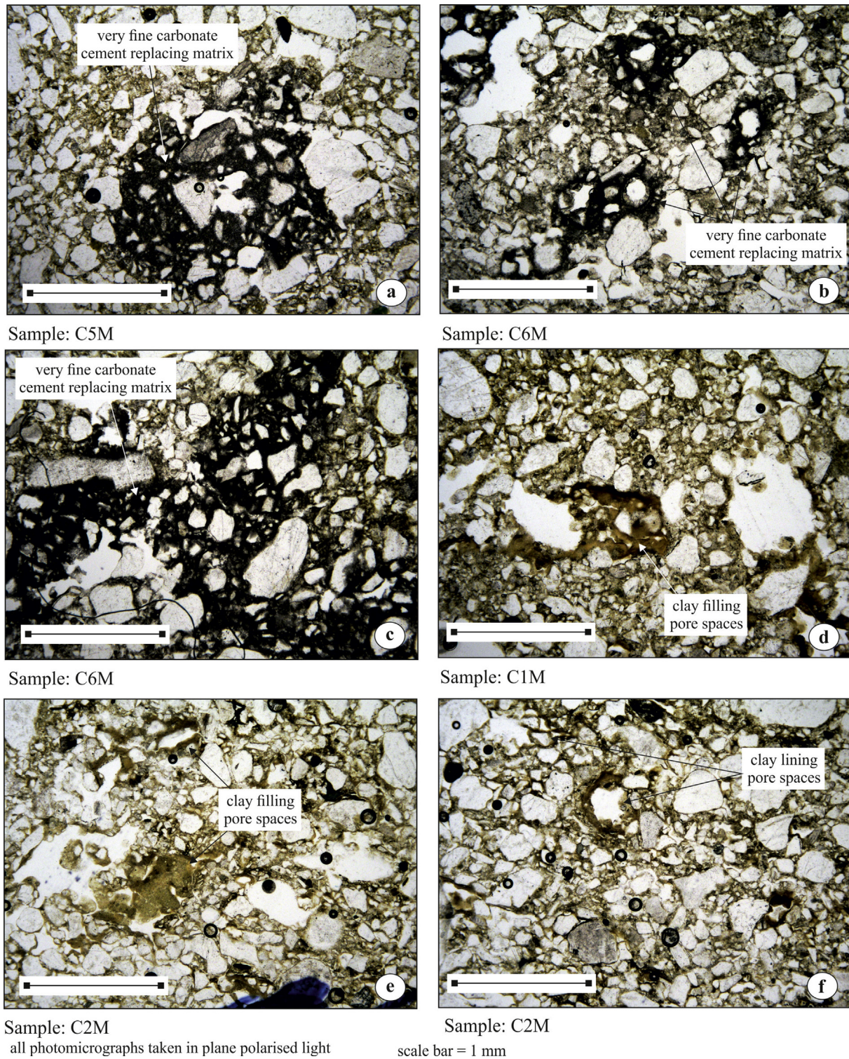
Fig. 9. Photomicrographs showing the fine-grained, dusty looking carbonate which locally replaces the matrix to the diamicton (a to c) and clay lined and filled pore spaces (d to f).
