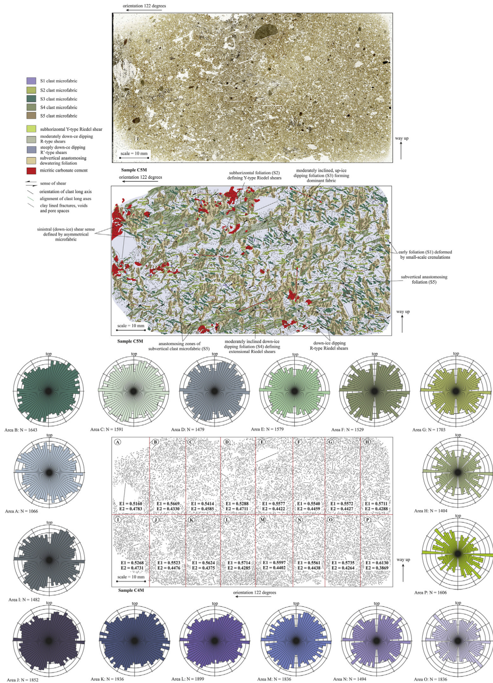
Fig. 6. Microstructural map and high resolution scan of thin section C5M. The orientation of the long axes of sand to granule sized clasts included within the diamicton are shown on a series of rose diagrams. The thin section has been subdivided into 16 subareas and the E1 and E2 eigenvalues calculated for each area (see text for details).
