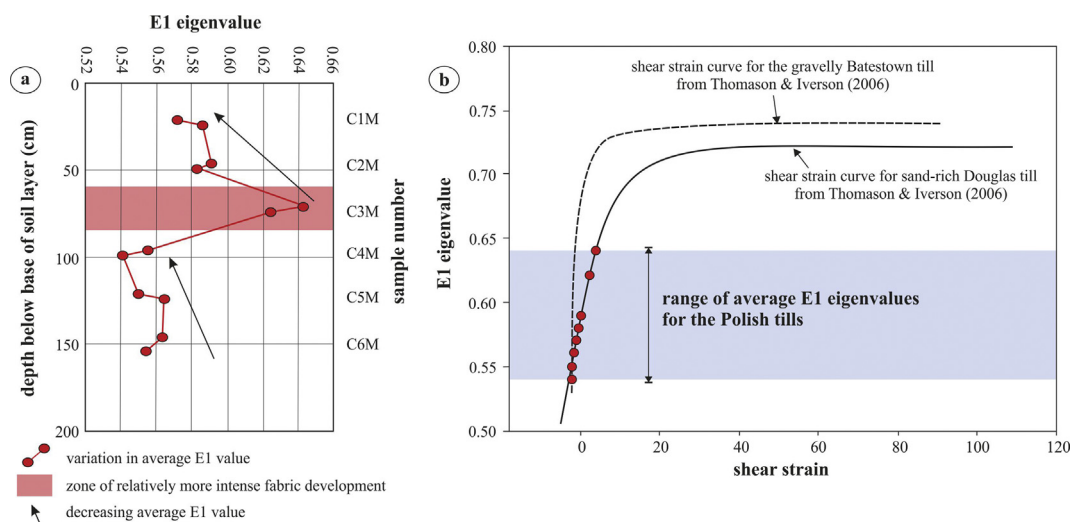
Fig. 14. (a) Plot showing the variation in average E1 eigenvalue calculated for each thin section (C1M to C6M) with respect to depth within the diamicton sequence; and (b) Plot of E1 eigenvalue against shear strain. The shear strain curves for the Batestown (gravelly) and Douglas (sand-rich) tills are taken from Thomason and Iverson (2006) and are used to obtain an estimate of the range of shear strains encountered by the diamicton exposed at site C.
