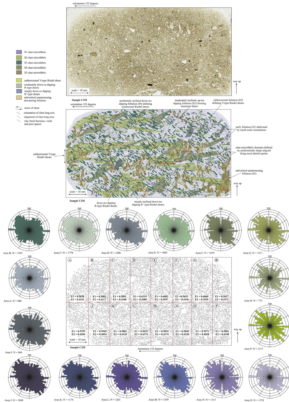
Fig. 3. Microstructural map and high resolution scan of thin section C2M. The orientation of the long axes of sand to granule sized clasts included within the diamicton are shown on a series of rose diagrams. The thin section has been subdivided into 16 subareas and the E1 and E2 eigenvalues calculated for each area (see text for details).
