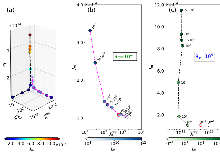
Figure A3. BISCLES L-curve analysis to select Tikhonov parameters \lambda_\phi and \lambda_C : (a) 3-D scatter plot of the model-data misfit J_m as a function of the regularisation terms J_C^{\text{reg}} and J_\phi^{\text{reg}} . (b) 2-D cross section for variable \lambda_\phi and \lambda_C fixed at 10^{-1} \text{ Pa}^{-2} \text{ m}^6 \text{ a}^{-4} . (c) Reverse case with constant \lambda_\phi at 10^9 \text{ m}^4 \text{ a}^{-2} and varying \lambda_C . The units of J_m and J_C^{\text{reg}} are \text{m}^4 \text{ a}^{-2} and \text{Pa}^2 \text{ m}^{-2} \text{ a}^2 , respectively. J_\phi^{\text{reg}} is unitless. Selected values are highlighted by red circles in (b) and (c) . The layout was inspired by Berger et al. (2016).
