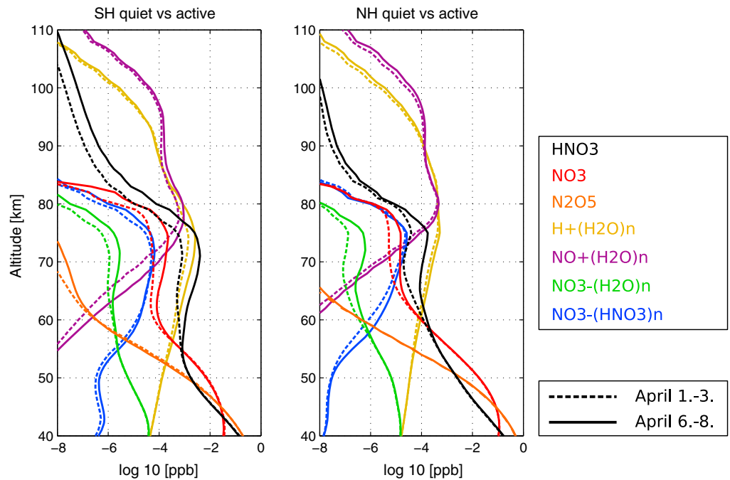
Figure 7. Vertical profiles of abundance of ion clusters and neutral species (in ppb, log10 scale). Three-day averages in quiet conditions (1–3 April, dashed lines) and active conditions (6–8 April, solid lines; southern hemisphere in left column, latitudes poleward of 50°S, and northern hemisphere in right column, latitudes poleward of 50°N) of the vertical profiles of abundance of the four key ion clusters and the neutral species HNO 3 , NO 3 , and N 2 O 5 in Whole Atmosphere Community Climate Model D -layer. All simulations are with medium-to-high energy electron included.
