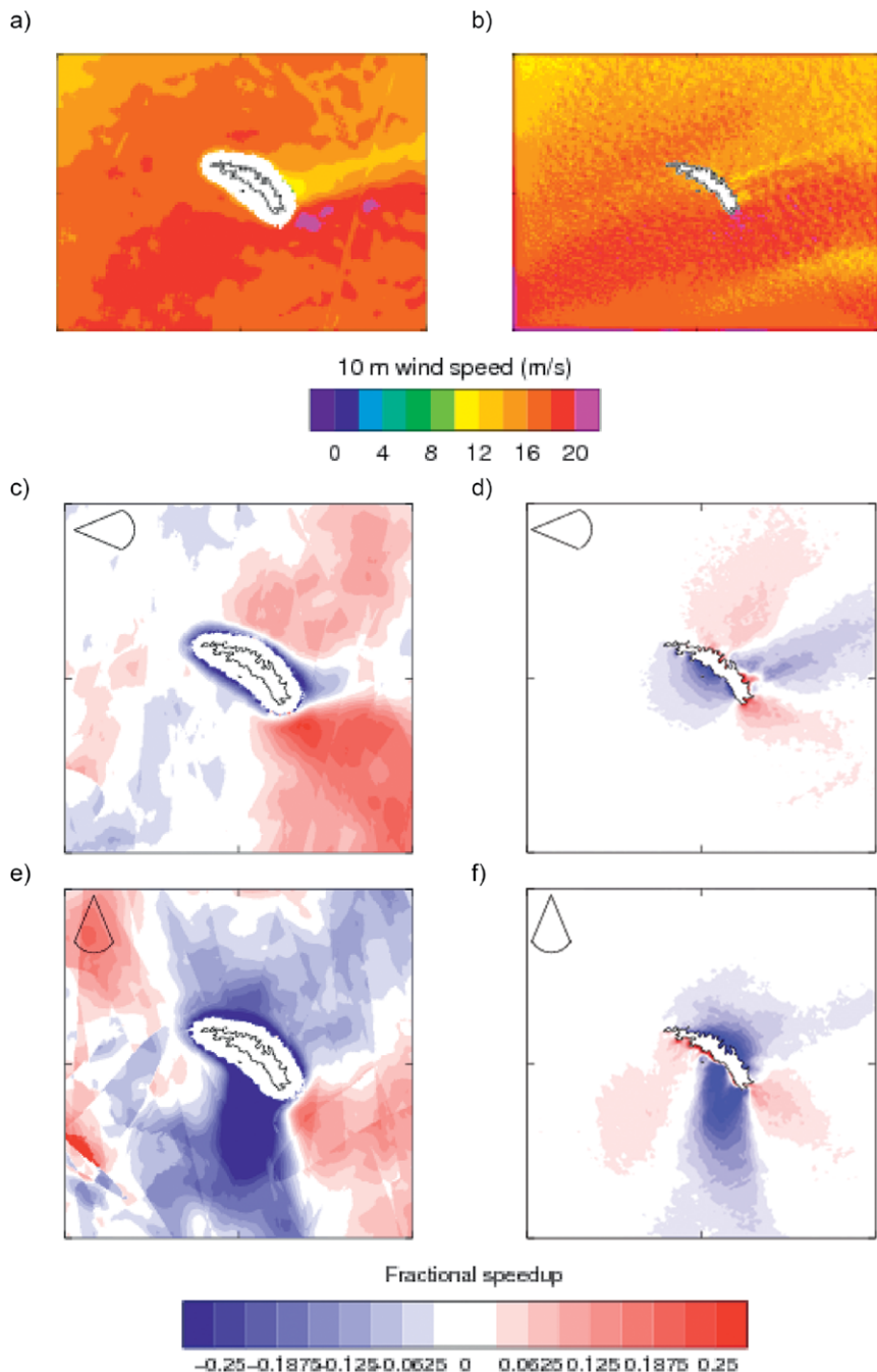
FIG. 8. The 10-m winds (a) measured by ASCAT near South Georgia on 5 Jul 2015 and (b) simulated by the UM on the 750-m grid. The ASCAT wind field in (a) is a composite of three scans taken at 0921, 1015, and 1103 UTC. The model wind field in (b) is an average over data at hourly intervals during the period 0900–1100 UTC from a simulation initialized at 0600 UTC. Also shown are the mean fractional speed-up \Delta s deduced from ASCAT winds for the Jun–Jul 2015 radiosonde campaign period during (c) westerly and (e) northerly flow and (d),(f) the respective equivalent 1.5-km model results. The segments in the upper-left corners of (c)–(f) indicate the range of wind directions considered.
