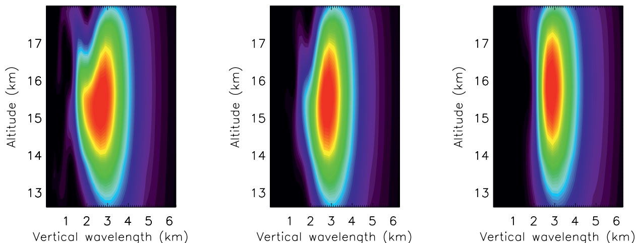
FIG. 7. Wavelet transforms of the temperature perturbation profiles for the (left) radiosonde, (center) low-resolution radiosonde, and (right) UM.
