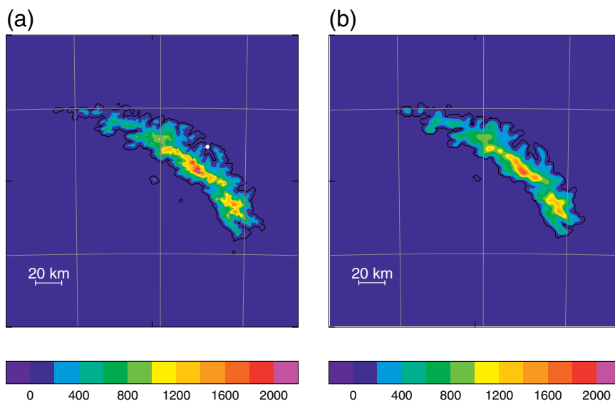
FIG. 1. The model orography for the UM limited-area simulations with (a) 750-m and (b) 1.5-km horizontal grid spacing. These data were created from SRTM digital terrain data with 3-arc-s resolution. Both panels show a zoomed-in view across South Georgia; the full extents of the model domains are considerably larger. Terrain heights are shown in meters (color contour interval: 400 m). Lines of constant latitude and longitude are shown with a 1° interval. The white dot in (a) marks the location of King Edward Point on the east coast.
