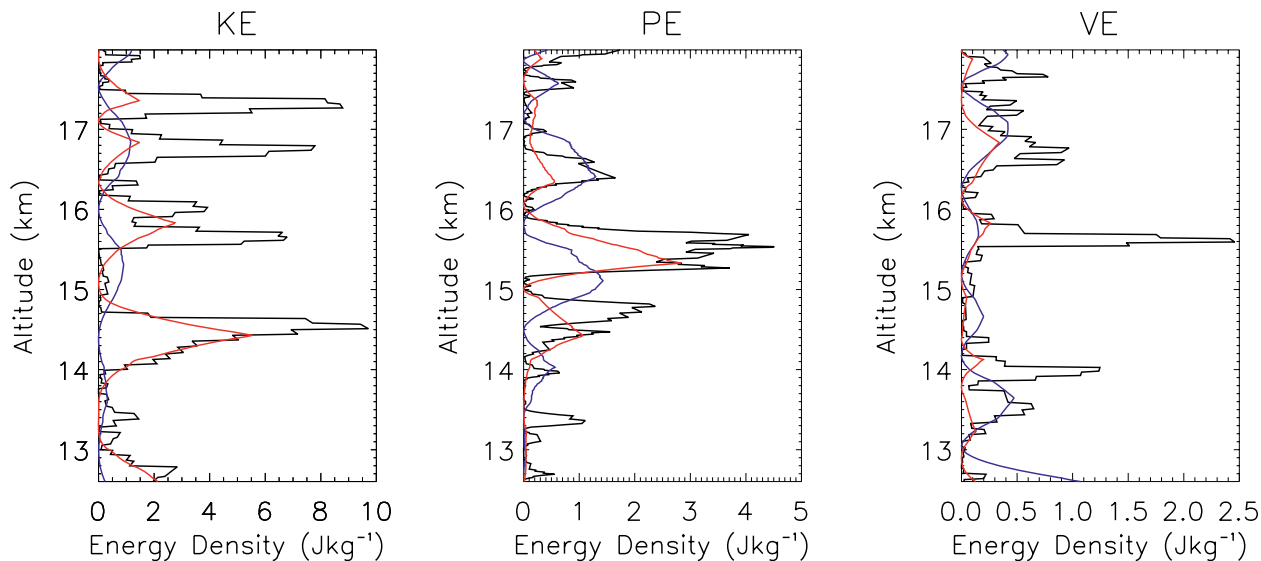
FIG. 6. (left) Kinetic energy density, (center) potential energy density, and (right) vertical energy density profiles for radiosonde (black line), UM (blue line), and low-resolution radiosonde (red line) on 5 Jul 2015. The y axis is altitude (km) and the x axis is energy density ( \text{J kg}^{-1} ).
