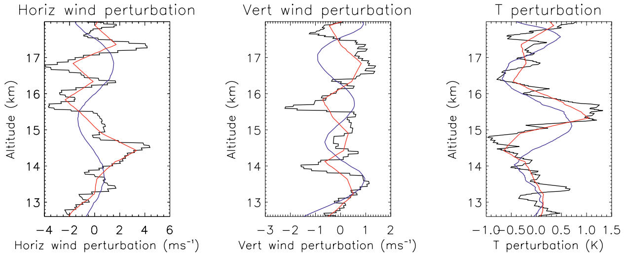
FIG. 5. (left) Horizontal wind perturbation, (center) vertical wind perturbation, and (right) temperature perturbation profiles for the 0853 UTC radiosonde (black line), the 1.5-km UM simulation (blue line), and the low-resolution radiosonde data (red line) on 5 Jul 2015.
