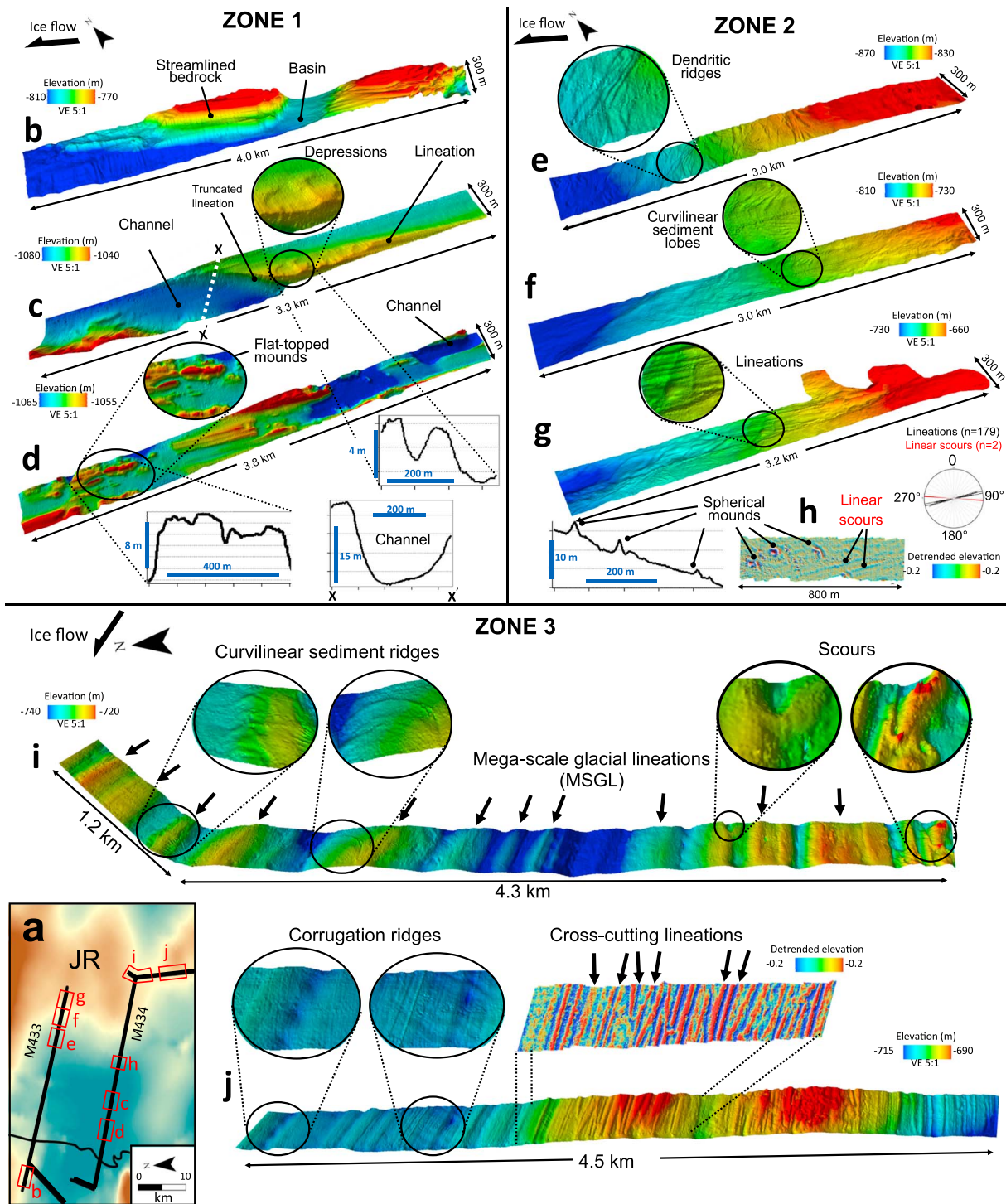
Figure 3. Three-dimensional surfaces of multibeam seafloor bathymetry. (a) Inset map showing the locations of Figures 3b–j. Multibeam surface imagery of seafloor topography and extracted topographic profiles in (b–d) Zone 1, (e–h) Zone 2, and (i and j) Zone 3. Location of Figure 3h is shown in the inset map and Figure 2e. Rose diagram next to Figure 3h shows the azimuth of lineations sampled from Zones 1–3 compared to linear scours in Figure 3h.
