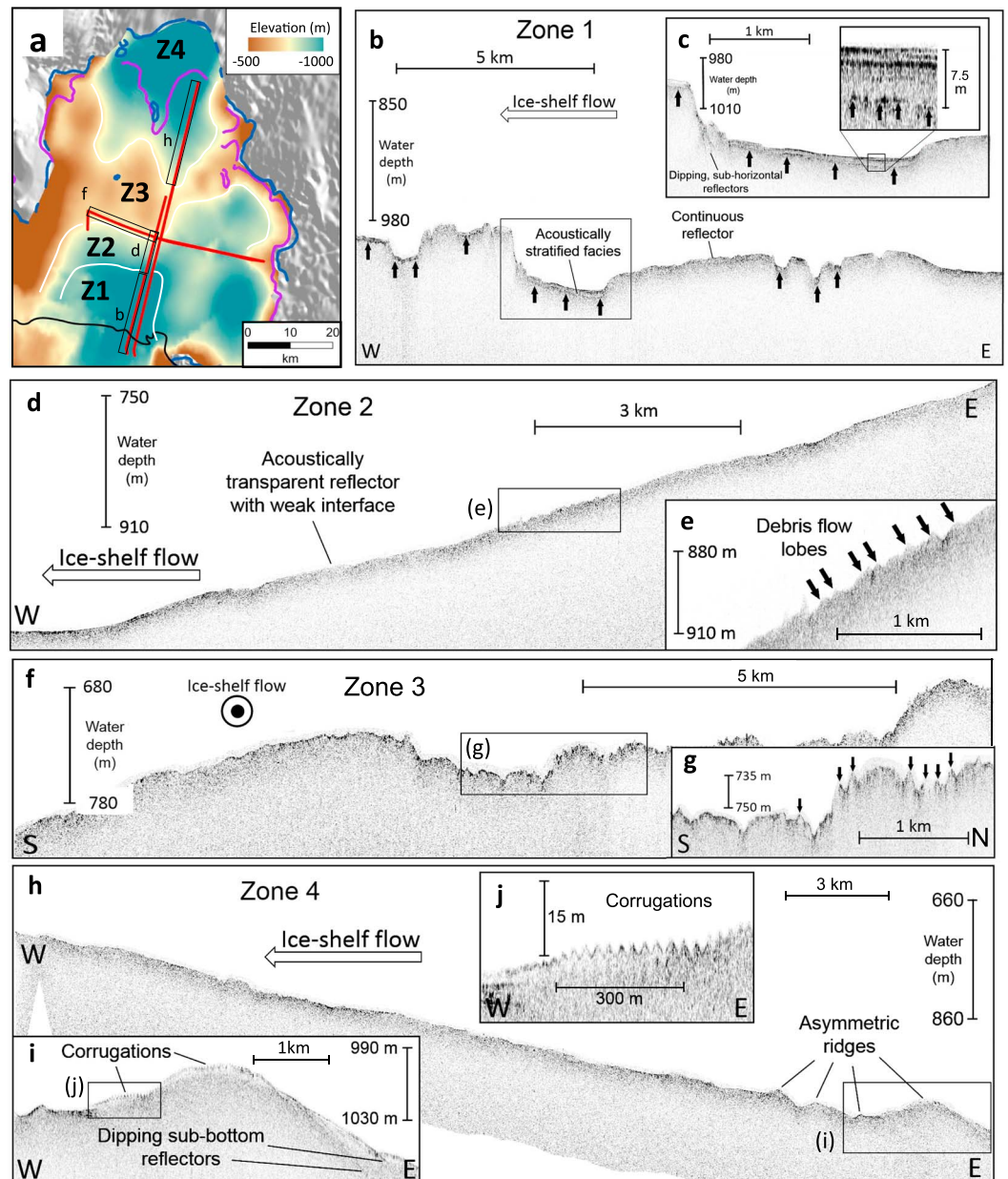
Figure 4. Acoustic sub-bottom profiler data. (a) Map of regional bathymetry and location of sub-bottom profiler surveys beneath Pine Island Glacier Ice Shelf. Black boxes denote sections of data shown in the main figure. (b) Rugged seafloor topography and acoustically stratified basins (black arrows) in Zone 1. (c) Close-up of an acoustically stratified basin showing up to 7.5 m of stratified sediments. Sediment thickness was calculated using an acoustic velocity of 1500 \text{ m s}^{-1} for sediments. (d) Acoustically transparent seafloor reflector of the seaward flank of Jenkins Ridge. (e) Close-up showing debris flow lobes (black arrows). (f) Profile across Jenkins Ridge showing a strong surface reflector and undulating seafloor. (g) Close-up showing mega-scale glacial lineations (black arrows). (h) Acoustically transparent seafloor reflector on the inland slope of Jenkins Ridge. (i) Close-up view of asymmetric ridges. (j) Close-up of corrugation ridges overprinting the crest of asymmetric ridges.
