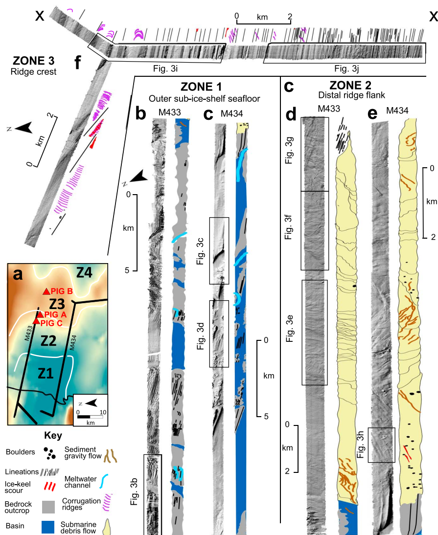
Figure 2. Sub-ice-shelf multibeam bathymetry data and geomorphological interpretation. (a) Map of regional bathymetry and location of multibeam surveys M433 and M434. Red triangles show the locations of sediment cores described in Smith et al. [2017]. Black line shows the ice-shelf front position in 2009. (b–f) Multidirectional relief-shaded multibeam topography plotted alongside corresponding geomorphological interpretations. Data width has been exaggerated by a factor of 2 for clarity. Black lines superimposed over debris flows delimit individual debris flow lobes. Black boxes show the location of three-dimensional surface imagery shown in Figure 3.
