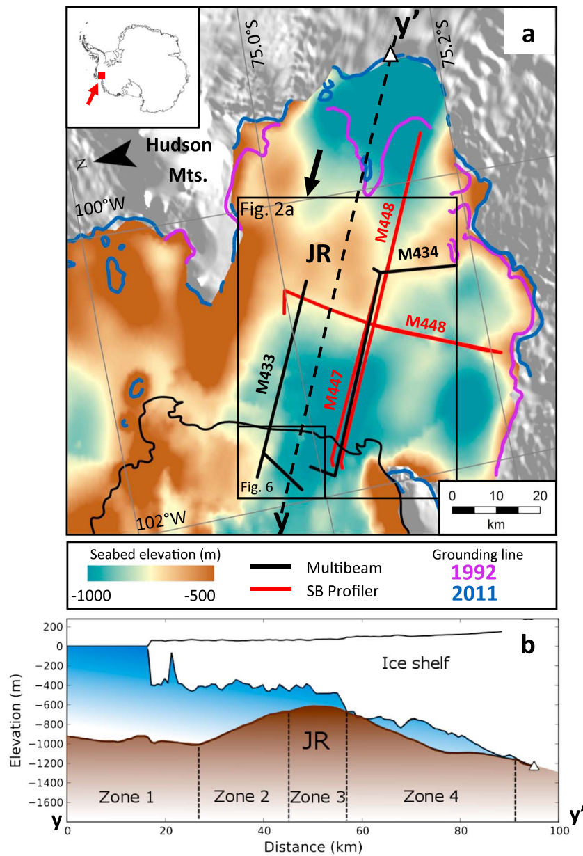
Figure 1. Map and locations of Autosub3 sub-ice-shelf missions beneath Pine Island Glacier Ice Shelf (PIGIS). (a) Sub-ice-shelf bathymetry derived from gravity inversion (see supporting information in Dutrieux et al. [2014a] for methodology) showing the location of Jenkins Ridge (JR) and Autosub3 mission tracks. Black line shows the ice-shelf front position in 2009. Boxes show areas covered by figures referred to later in text. Grounding line locations are from the MEaSURES data set [ Rignot et al. , 2011]. (b) Cross section of ice and seafloor geometry extracted from profile y-y' (dashed black line) showing geomorphic zones 1–4 (ice draft and bathymetry from Dutrieux et al. [2014a]; see their supporting information for methodology). Data for each zone are shown in Figures 2–4.
