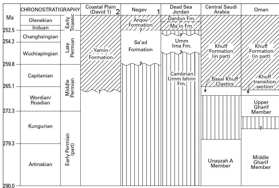
Fig. 11 - Correlation of the Permian-Triassic successions in the Levant and Arabian Plate. Cross-hatching indicates predominantly marine strata. 1) (Negev) after Eshet and Cousminer (1986); these authors regard the Arqov Formation as Permian in age; 2) Coastal Plain (David 1) after Korngreen et al. (2013); Dead Sea, Jordan, this paper; central Saudi Arabia and Oman after Angiolini et al. (2003) and Stephenson (2006).
