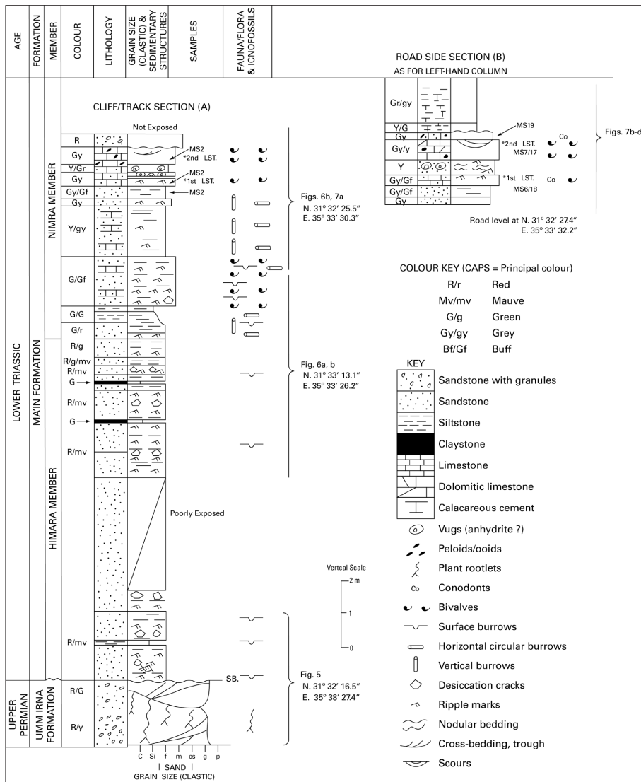
Fig. 3 - Graphic log of the Upper Permian to Lower Triassic succession in the studied Dyke Plateau section. Roadside section B is located 200 m east of the Cliff/track section A. SB is the sequence boundary between the Umm Irna and Ma'in formations. The approximate positions of Figs 5 to 7 are shown. MS indicates level of limestone samples.
