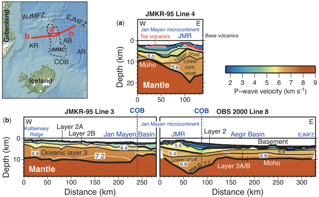
Fig. 9. P-wave velocity models at the Jan Mayen microcontinent: (a) JMCR-95 line 4 (after Kodaira et al. 1998b); and (b) JMCR-95 line 3 (after Kodaira et al. 1998a) and line 8 of the OBS 2000 survey (after Mjølde et al. 2008). Abbreviations: AB, Aegir Basin; AR, Aegir Ridge; COB, continent–ocean boundary; cont., continental; EJMfZ, East Jan Mayen Fracture Zone; HVLC, high-velocity lower crust; JMMC, Jan Mayen microcontinent; JMR, Jan Mayen Ridge; KR, Kolbeinsey Ridge; WJMfZ, West Jan Mayen Fracture Zone.
