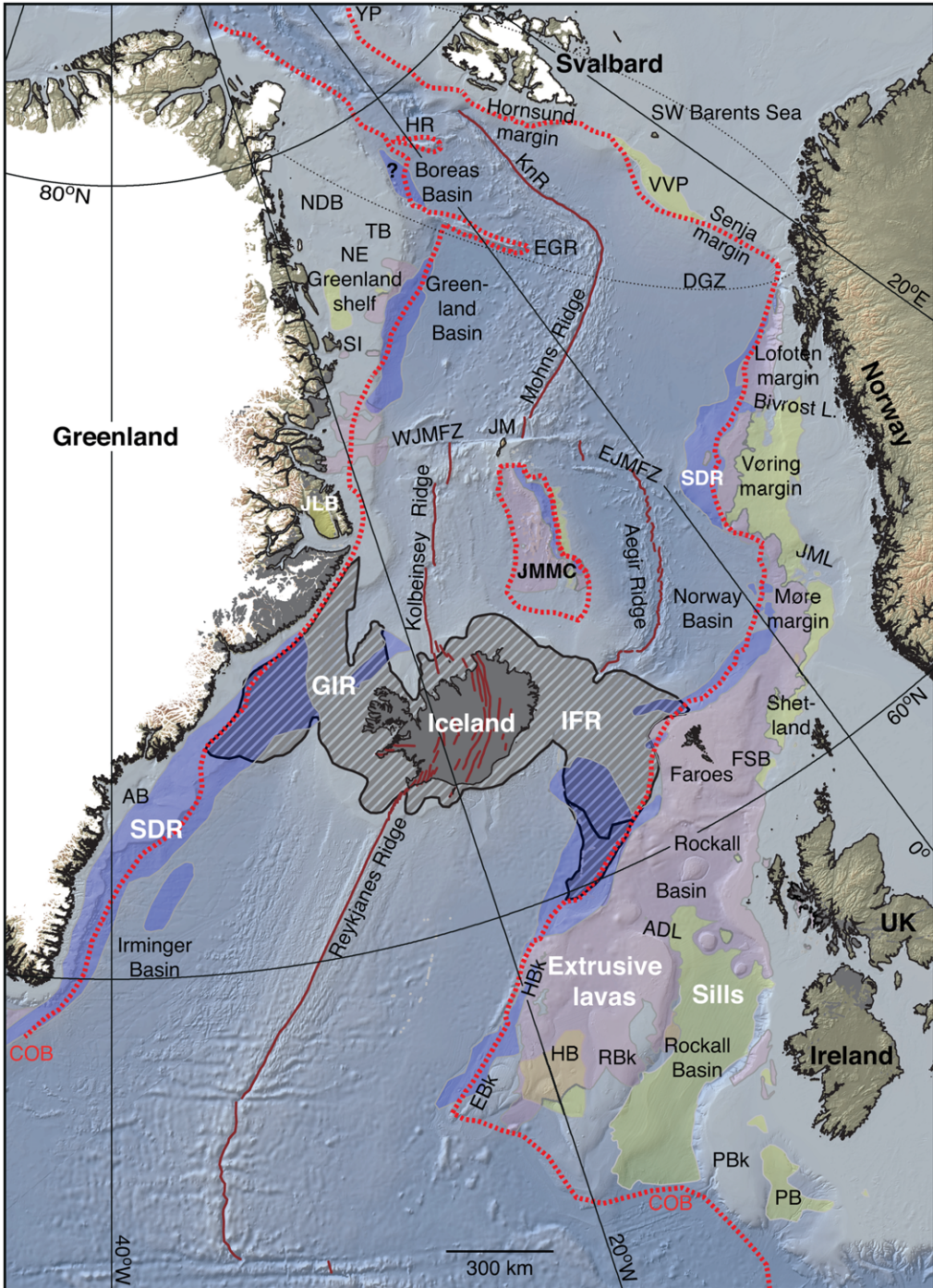
Fig. 1. Physiographical map (after Hopper et al. , this volume, in prep) of the NE Atlantic Ocean with the extent of the North Atlantic Igneous Province. The continent–ocean boundary (COB; dashed red line) is taken from Funck et al. (2014). Transparent overlays mark SDRs (blue), extrusive lavas (purple/pink), sills (green), the Greenland–Iceland–Faroe Ridge complex (hatched) and the onshore volcanic rocks (grey): all after á Horni et al. (2014), see also á Horni et al. (this volume, in review). Red lines mark the location of active and extinct spreading centres.
