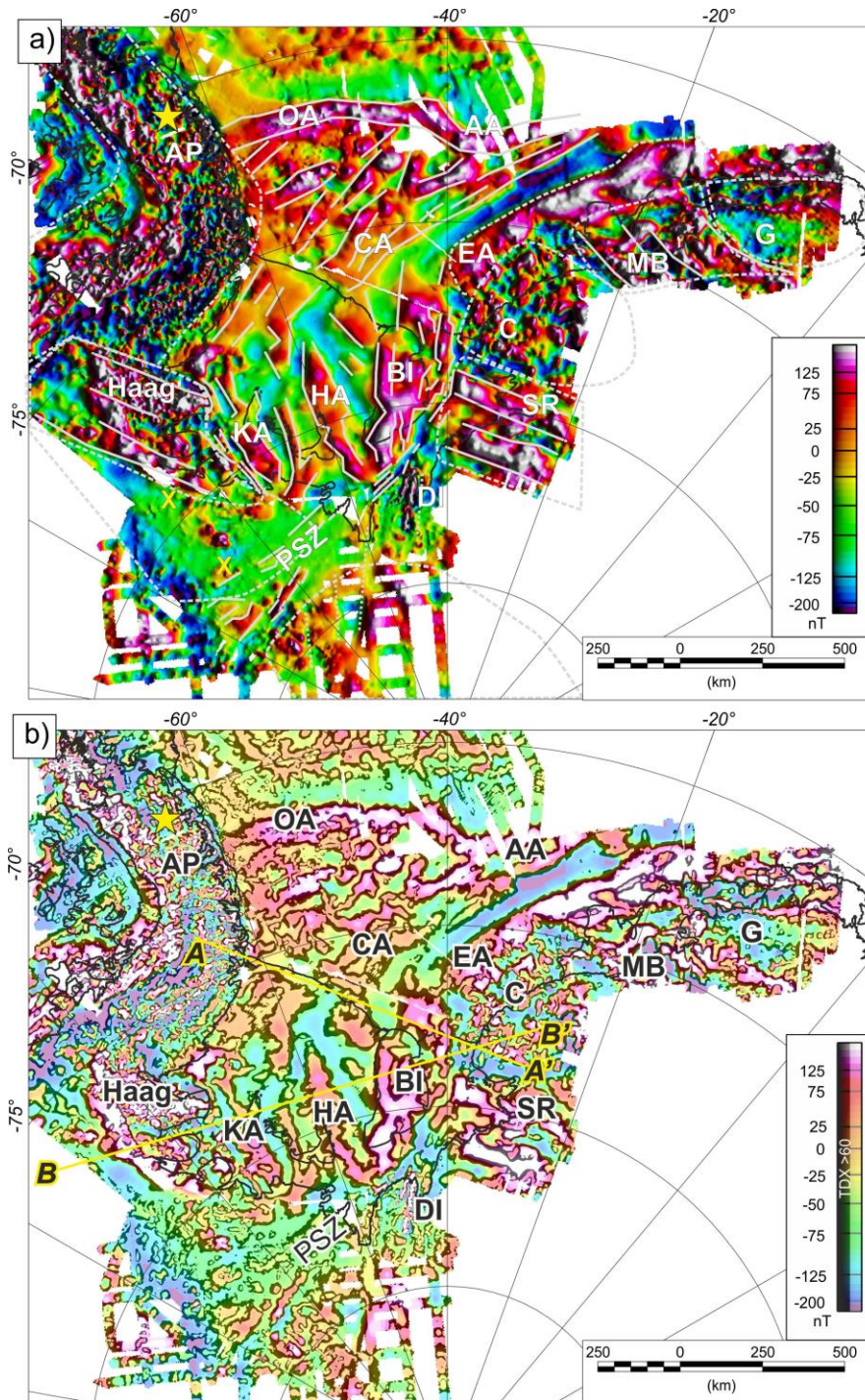
Figure 4. New aeromagnetic anomaly compilation. a) Reduced to pole (RTP) total field magnetic anomaly map. Solid grey lines show picked lineaments based on manual interpretation of TDX enhancement in (b). Dashed grey lines indicate magnetic provinces based on TDX enhancements and pseudo-gravity terrace map (Fig. 5a). Note linear north-
