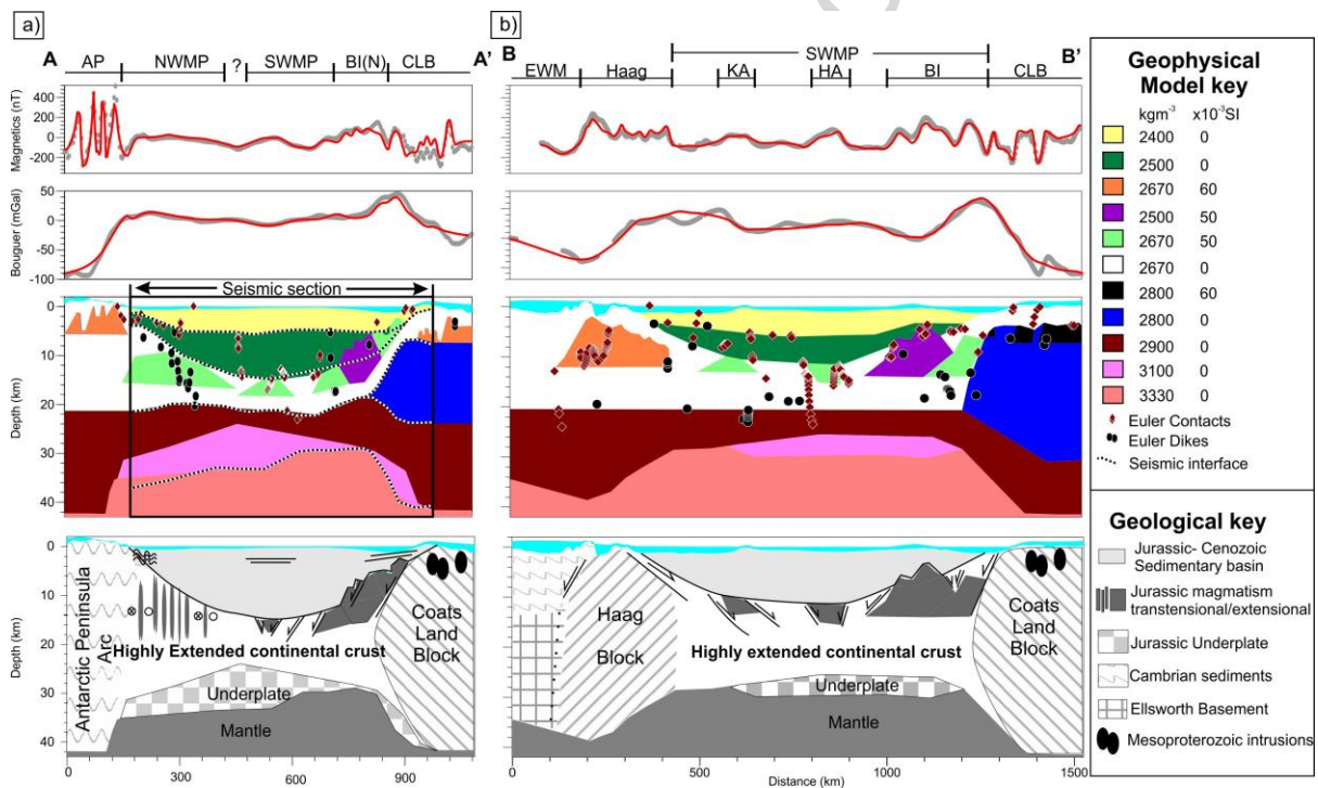
Figure 7. 2D potential field models and geological interpretation. See Fig. 6 for location. a) Profile constrained by seismic refraction data (Leitchenkov and Kudryavtzev, 1997) between Antarctic Peninsula (AP) and Coats Land Block (CLB), crossing the Northern and Southern Weddell Magnetic provinces (NWMP and SWMP), and passing north of Berkner Island (BI(N)). Note the boundary between the NWMP and SWMP is not well defined. First (top) panel shows observed (grey) and modelled (red) magnetic anomalies. Second panel shows observed (grey) and modelled (red) Bouguer gravity anomalies. Third panel shows modelled
