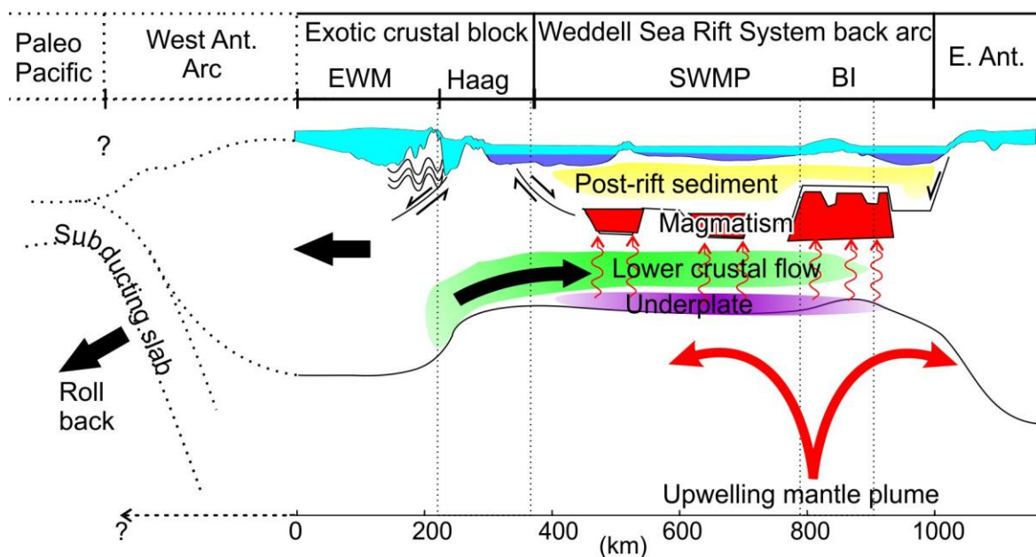
Figure 8. Interpretative sketch of the Jurassic tectonic and magmatic setting of the Weddell Sea Rift System. Structures in colour are derived from our modelling and interpretation of geophysical data between Coats Land and HEW. Dotted lines denote inferred Jurassic West Antarctic and Paleo-Pacific margin. Note inferred HEW exotic crustal block transferred from East Antarctica by crustal extension in the WSRS. WSRS extension was potentially enhanced by plume related magmatism and flow of lower crustal material from beneath the now thinned Haag region.
