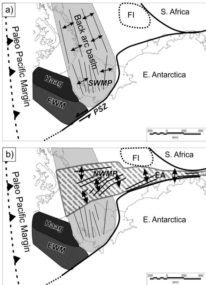
Figure 9. Cartoon showing two phase extensional model for the evolution of the WSRS. a) Early phase of back-arc extension gives rise to N/S oriented SWMP structures. b) Later phase of rifting between South Africa and East Antarctica creates NWMP, cross cutting older SWMP. Note in these sketches the Antarctic Peninsula is shown in its present day position. Structures beneath the present day Antarctic Peninsula are inferred, as this region is overprinted by Cretaceous arc processes, and the Jurassic position of the Antarctic Peninsula is not well constrained. Also note the extent and the independent rotation or translation of the Falkland Island block (FI) is not considered in these simple sketches.
