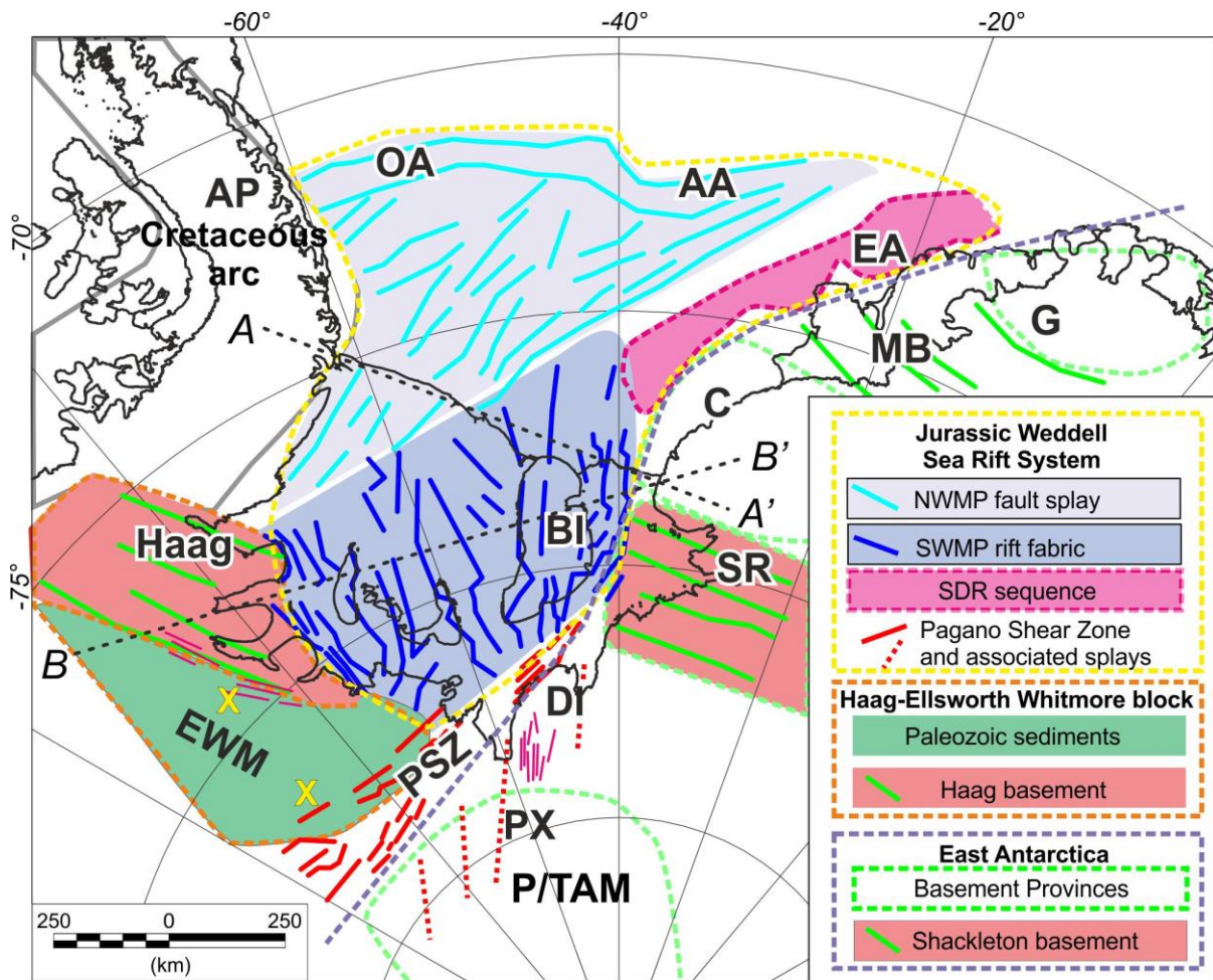
Figure 6. Interpretative sketch of key magnetic lineaments and provinces.
