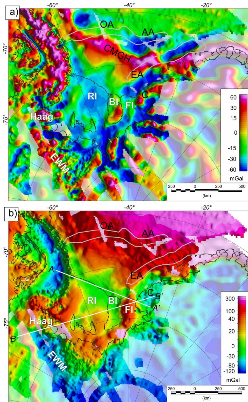
Figure 3. New gravity compilation maps. Transparent background image shows GOCO3s satellite gravity data (Mayer-Gürr et al., 2012). a) Free air anomaly map. Note general correlation with sub-ice topography/bathymetry (Fig. 1), with the exception of the positive Continental Margin Gravity High (CMGH). Thin grey lines mark extent of selected magnetic anomalies (abbreviations as in Fig.1). RI and FI mark Ronne and Filchner Ice shelves
