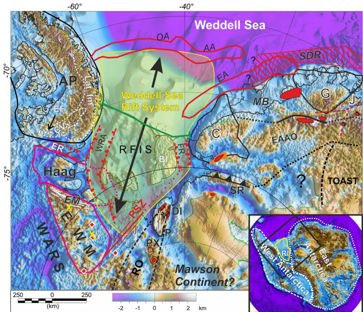
Figure 1. Regional topography and geological sketch map of the Weddell Sea Rift System (WSRS) (yellow outline). Note displaced Haag and Ellsworth Whitmore Mountains (EWM) crustal block (purple outlines). Key Jurassic features associated with Gondwana breakup include: widespread Ferrar tholeiitic rocks (solid red blocks) (Elliot and Fleming, 2004); Dufek Intrusion (DI) (black/red check) (Ferris et al., 1998); Jurassic granites (red diamonds) (Storey et al., 1988b); Seismically imaged seaward dipping reflector sequences (SDR) (red hatch) (Kristoffersen et al., 2014); Orion, Andenes and Explora magnetic anomalies (OA, AA and EA) linked to Jurassic magmatism (Ferris et al., 2000; Golynsky and Aleshkova, 1997a); Localised rifts including the Evans Rift (ER), Weddell Rift Anomaly (WRA), Filchner Rift (FR), and
