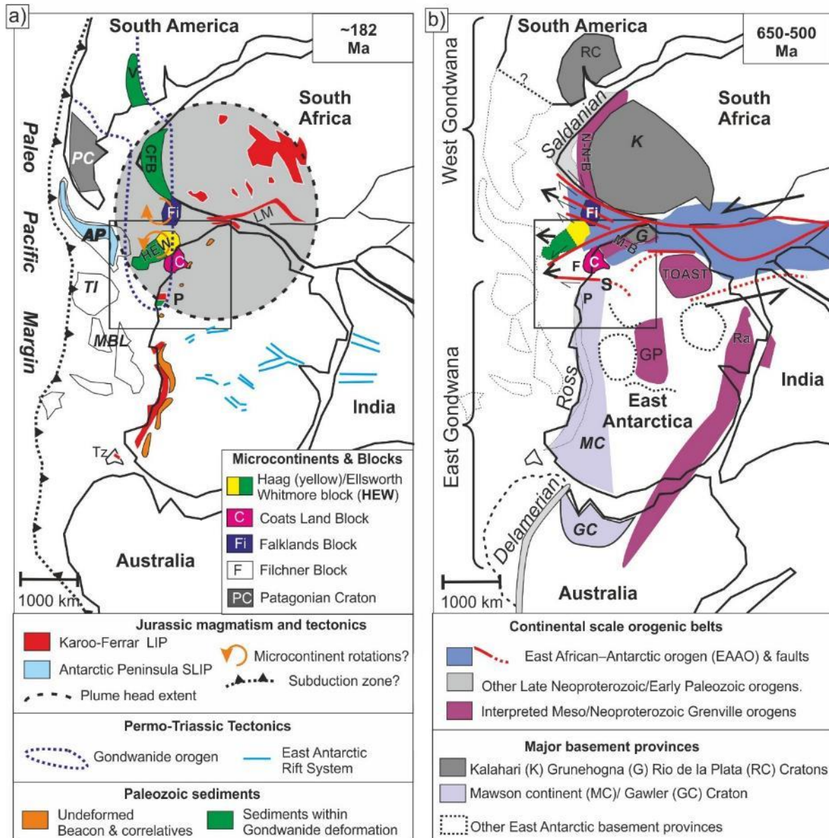
Figure 2. Tectonic and geological sketch of Gondwana. Reconstructions modified after Dalziel (2013) and Jacobs et al., (2015) respectively. a) Permian to Jurassic fragmentation of Gondwana. Note tight reconstruction of Haag-Ellsworth Whitmore Mountains (HEW) block (yellow and green respectively) assuming no pre-existing Filchner Block (Dalziel, 2013). Black box locates study area. Abbreviations: Cape Fold Belt (CFB), Lebombo Monocline (LM), Thurston Island (TI), Marie Byrd Land (MBL), Tasmania (Tz), Pensacola Mountains (P). Other abbreviations as in Fig. 1. b) Precambrian and Cambrian building of Gondwana. Early
