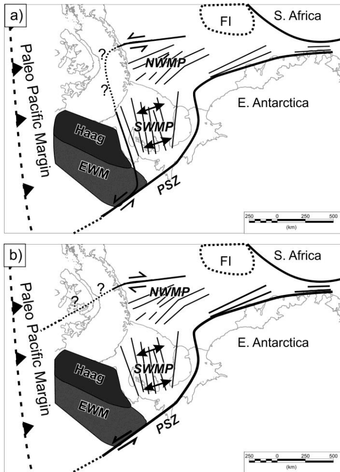
Figure 10. Cartoon showing possible scenarios for synchronous formation of Weddell Sea Rift System magnetic fabric. a) Simultaneous left lateral motion of PSZ and NWMP create a distributed transtensional releasing bend forming SWMP. b) Synchronous conjugate sinistral PSZ and dextral NWMP allows extensional SWMP to develop.
