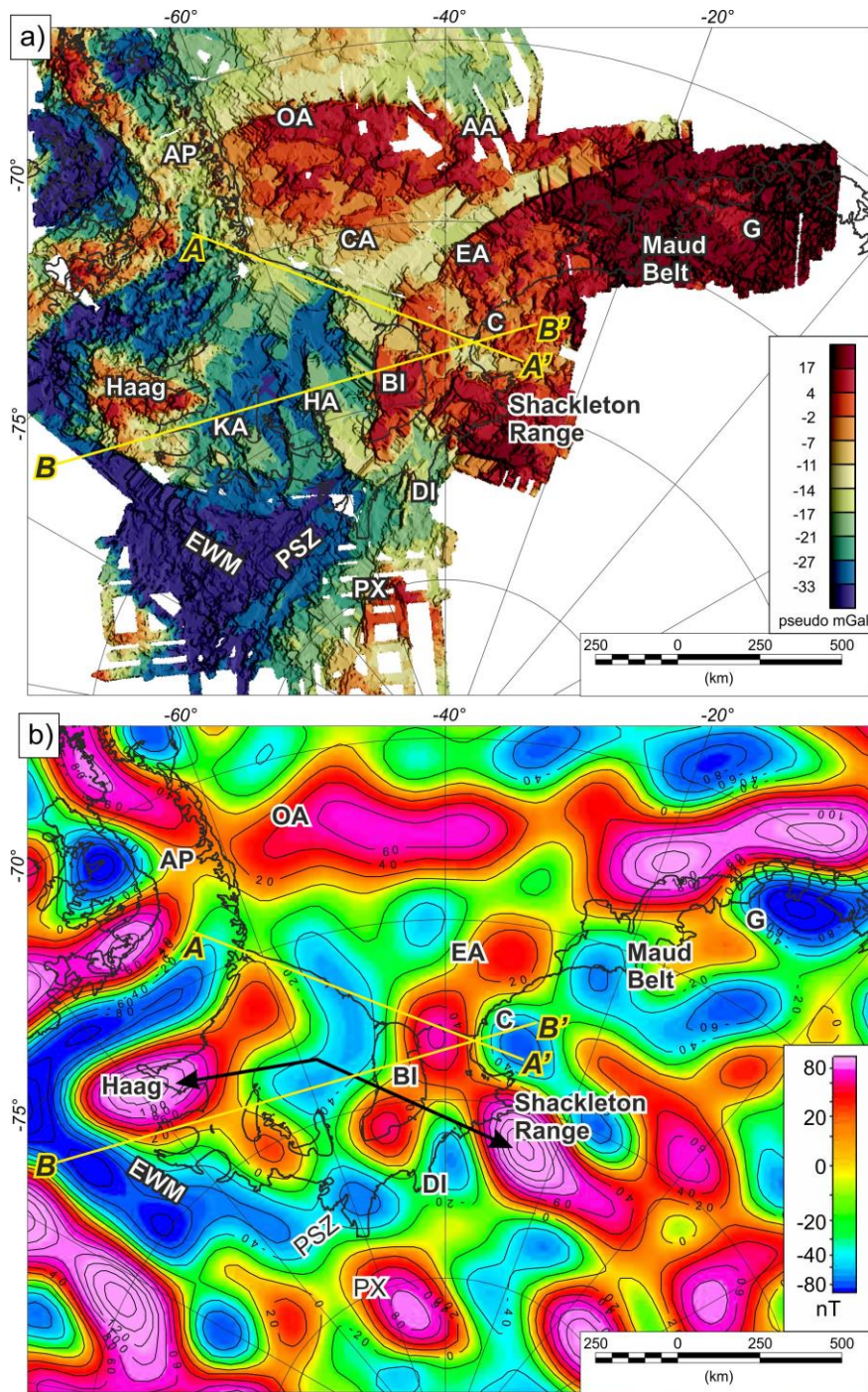
Figure 5. Regional magnetic features. a) Pseudo-gravity terrace map derived from new aeromagnetic compilation (Fig. 4a). Note distinct Haag and EWM provinces. b) MF7 satellite magnetic anomaly model, an update to the earlier MF6 model (Maus et al., 2008). Note distinct Haag and EWM provinces are also visible in this long wavelength field. Also note
