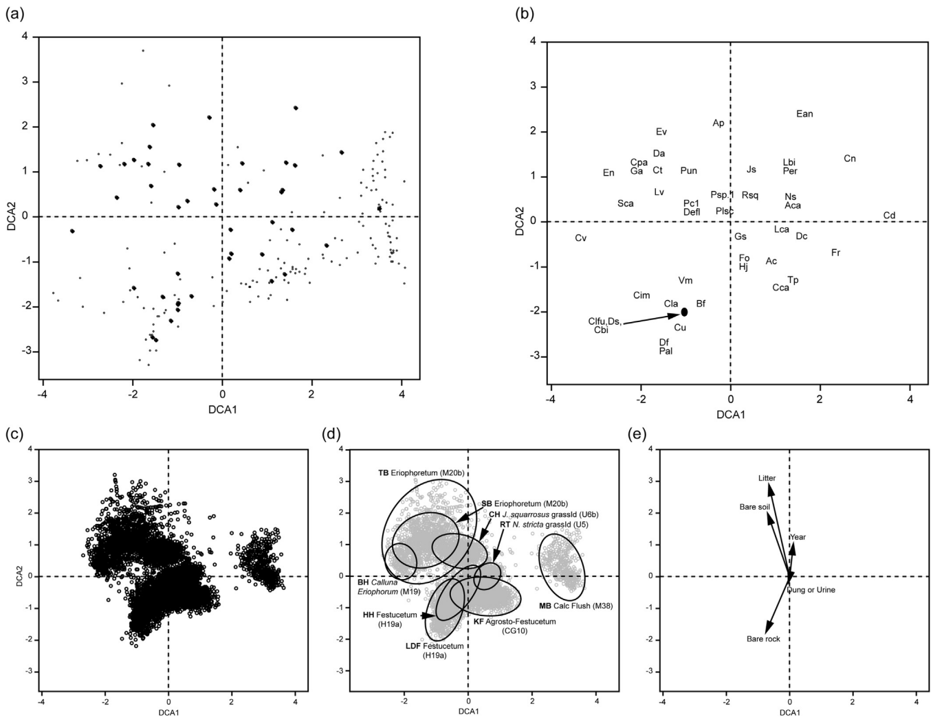
Fig. 1. Plots derived from the DCA analysis of plant species composition data within nine experiments investigating the effects of sheep-grazing versus no sheep grazing at Moor House NNR, north-west England: (a) Species plot, all species are illustrated (large dots = the most abundant species); (b) Species plot showing only the most abundant species (species with more than 500 presences in the database (max = 35,199 for Festuca ovina ); this encompassed 23% of the total number of species); (c) the distribution of sampling units; (d) the distribution of the nine experiments in ordination space illustrated using bivariate SD-ellipses (95% confidence limits) superimposed; (e) the significant environmental variables correlated with the ordination. Species codes for (b): Ac = Agrostis capillaris , Aca = Agrostis canina , Ap = Aulacomnium palustre , Bf = Barbilophozia spp, Cbi = Carex bigelowii , Cca = Carex caryophylla , Cd = Carex demissa , Cim = Cladonia impexa , Cla = Cladonia arbuscula , Clfu = Cladonia furcata , Cn = Carex nigra , Cpa = Campylopus paradoxus , Ct = Calypogeia spp, Cu = Cladonia uncialis , Cv = Calluna vulgaris , Da = Diplophyllum albicans , Dc = Deschampsia cespitosa , Df = Deschampsia flexuosa , Ds = Dicranum fuscescens , Ds = Dicranum scoparium , Ean = Eriophorum angustifolium , En = Empetrum nigrum , Ev = Eriophorum vaginatum , Fo = Festuca ovina , Fr = Festuca rubra , Ga = Green algae , Gs = Galium saxatile , Hj = Hypnum jutlandicum , Js = Juncus squarrosus , Lbi = Lophocolea bidentata , Lca = Luzula campestris/multiflora , Lv = Lophozia spp, Ns = Nardus stricta , Pal = Polytrichum alpestre , Pc1 = Ptilidium ciliare , Per = Potentilla erecta , Plsc = Pleurozium schreberi , Psp 1 = Polytrichum sp, Pun = Plagiothecium undulatum , Rsq = Rhytidiadelphus squarrosus , Sca = Sphagnum capillifolium , Tp = Thymus praecox/arcticus , Vm = Vaccinium myrtillus . Site codes for (d): BH = Bog Hill, CH = Cottage Hill, HH = Hard Hill, LDF = Little Dun Fell, KF = Knock Fell, MB = Moss Burn, RT = River Tees, SB = Silverband, TB = Troutbeck Head.
