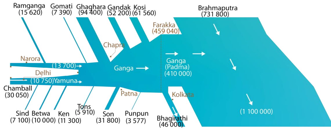
Figure 10 – Schematic of the Ganges and Brahmaputra river systems and their average annual discharge (million m³/yr) (adapted from Singh et al 2007).
