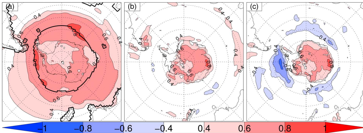
Figure 4. (a) Map of the cross-model correlations between simulated annual mean historical SH SIA and grid point \Delta T_{AS} (i.e., at each grid point a vector of n SIA values from the n=37 models is correlated with a vector of n annual mean \Delta T_{AS} values at that grid point). Positive values indicate that models with larger historical SIA give more warming over the 21st century under RCP8.5. (b) Correlation between SIA and grid point \Delta PR and (c) correlation between SIA and grid point \Delta PME . The thick solid lines in Figure 4a show the 15% contour for the multimodel mean annual mean historical sea ice concentration.
