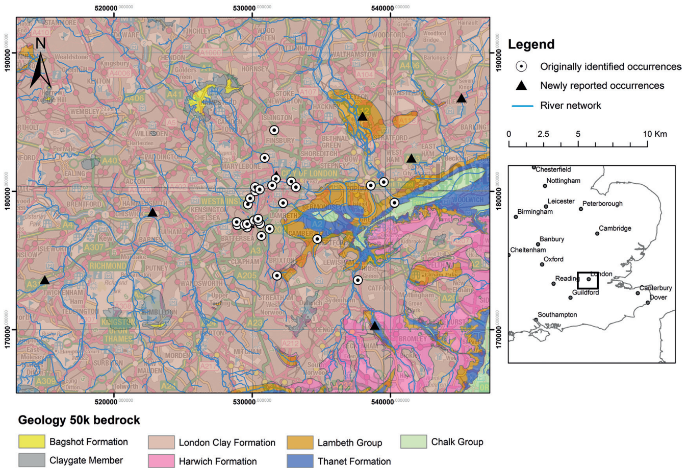
Fig. 1. Location of the originally identified and newly reported occurrences of buried hollows in central London. The underlying bedrock geology (1:50000) is shown along with the modern river drainage network. BGS©NERC. Contains Ordnance Survey data © Crown Copyright and database rights 2014. Lost rivers of London reproduced from Barton (1992).
