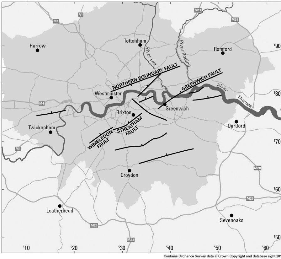
Fig. 4. Mapped faults. BGS©NERC.
