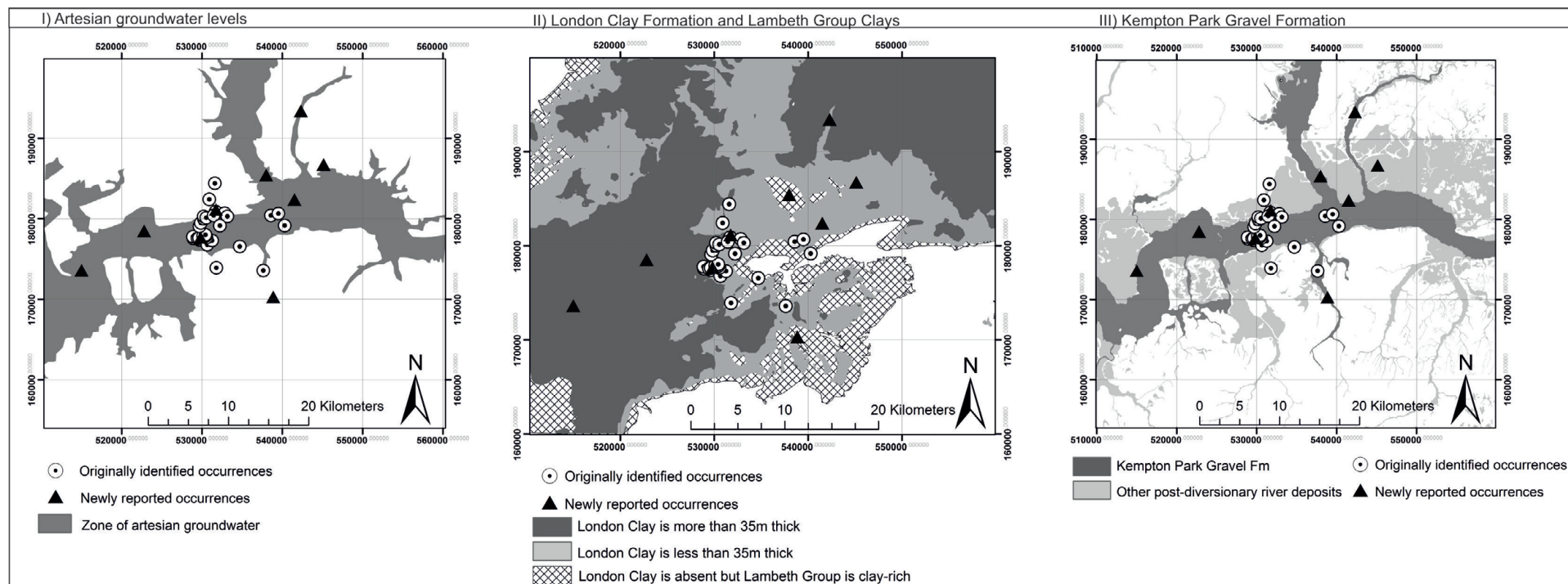
Fig. 3. Factors contributing to the susceptibility map. BGS©NERC. Zone of artesian groundwater © Environment Agency copyright and/or database rights 2012. All rights reserved. Lost rivers of London reproduced from Barton (1992).
