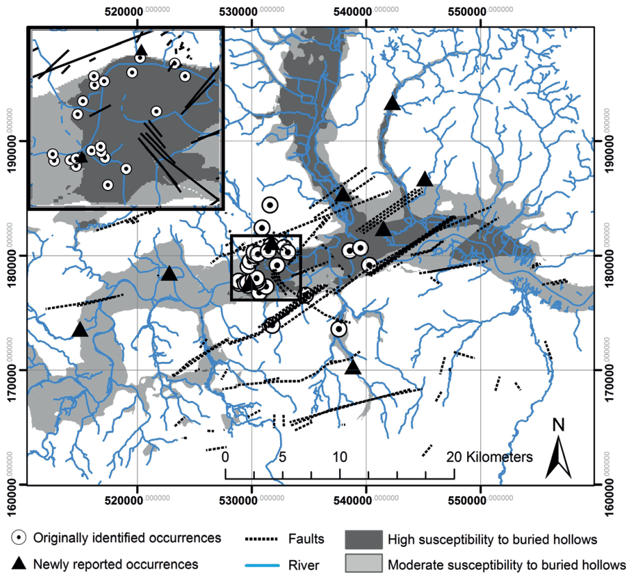
Fig. 5. Zoned hazard susceptibility map. BGS©NERC. Contains OS Open data ©Crown Copyright and database rights 2014. Lost rivers of London reproduced from Barton (1992).
