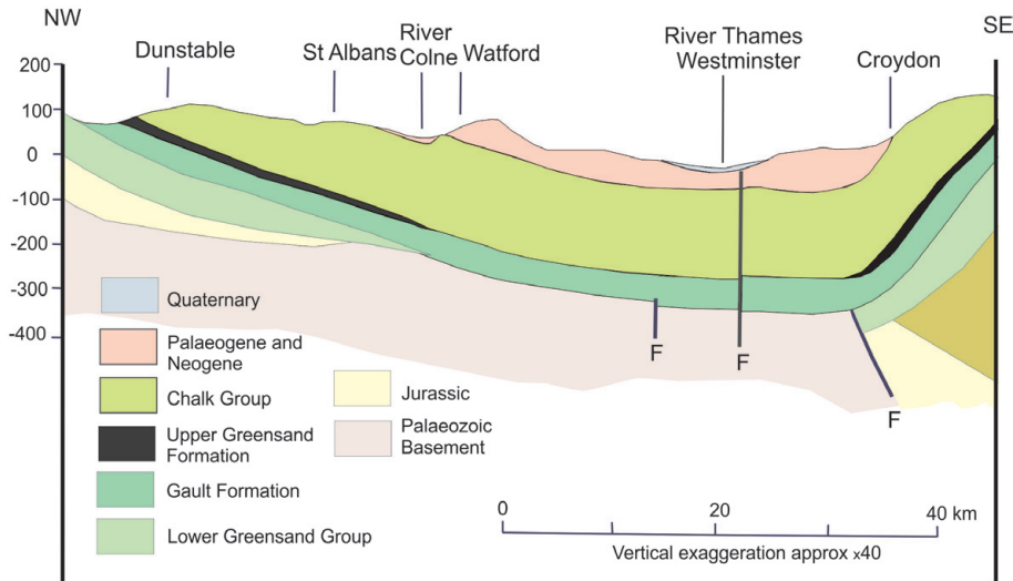
Fig. 2. Schematic, simplified geological cross-section, oriented NW–SE through the London Basin. Major faults are indicated (F); other faults (Fig. 4) are not shown (Royle et al. 2012, fig. 3).
