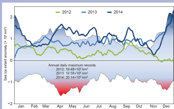
FIG. SB6.3. 5-day running mean of 2012 (green), 2013 (light blue), and 2014 (dark blue) daily sea ice extent anomaly relative to the 1981–2010 mean ( \times 10^6 km 2 ) for the Southern Hemisphere. The shaded banding represents the range of daily values for 1981–2010.
