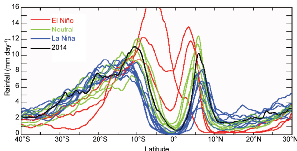
FIG. 4.14. TRMM-3B43 rainfall rate (mm day -1 ) for Jan–Mar, for each year 1998 to 2014, averaged over the longitude sector 180°–150°W. The cross-sections are color coded according to NOAA’s Oceanic Niño index, except for 2014 (an ENSO-neutral year) shown in black. The high rainfall near 5°S coincided with the extreme 1998 El Niño.
