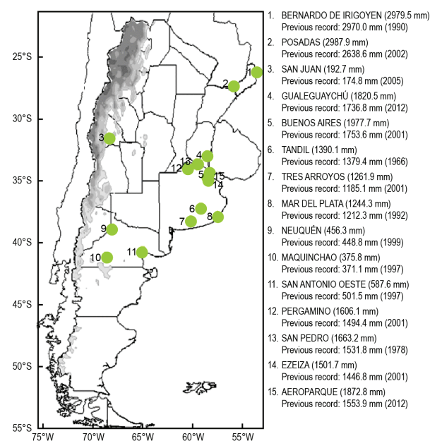
FIG. 7.15. 2014 annual precipitation records for Argentina. (Source: Argentina’s Servicio Nacional Meteorológico.)
