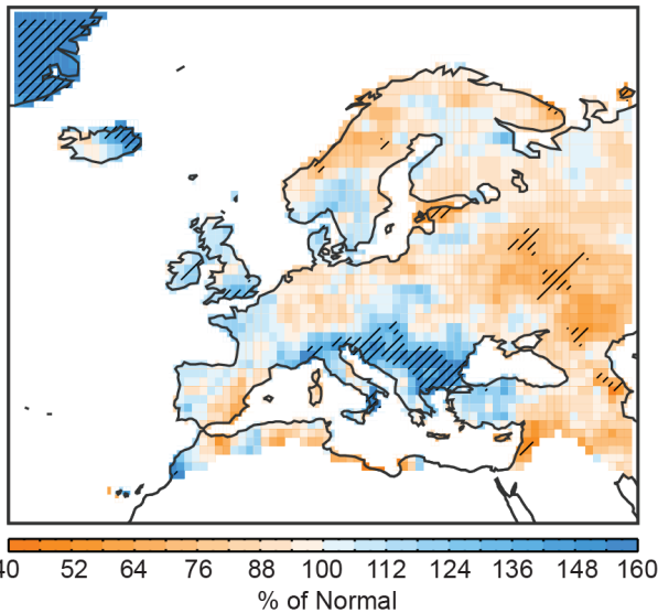
FIG. 7.28. European precipitation totals (% of 1961–90 average) for 2014. Hatched areas indicate regions where precipitation is higher (lower) than the 95th percentile (5th percentile) of the 1961–90 distribution. Only grid points with mean annual precipitation >15 mm month -1 are represented. [Source: Global Precipitation Climatology Centre (Becker et al. 2013).]
