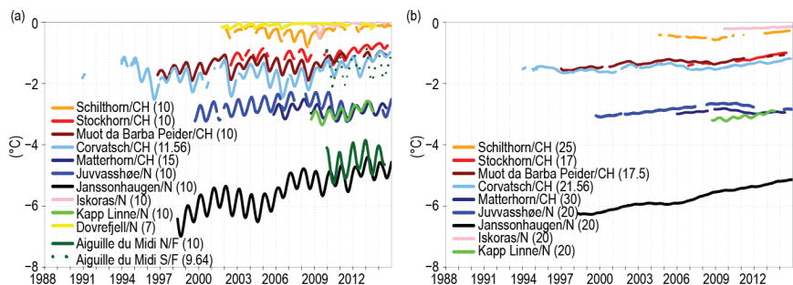
FIG. 2.8. Permafrost temperatures ( ^{\circ}\text{C} ) in daily or monthly resolution measured at (a) 10-m and (b) 20-m depth for selected boreholes in the European Alps, Scandinavia, and Svalbard showing (a) seasonal as well as (b) long-term variations of permafrost temperatures at depth. Data from Swiss sites are provided by PERMOS, for Norwegian sites by the Norwegian Meteorological Institute and the Norwegian Permafrost Database, and from the French site by EDYTEM/University of Savoie.
