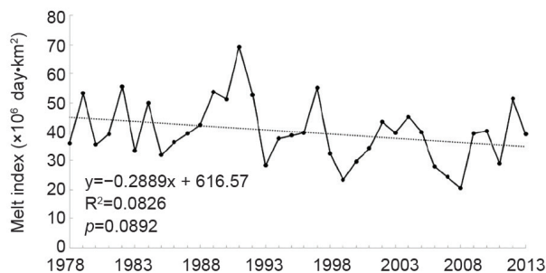
FIG. 6.8. Melt index ( 10^6 \text{ day}\cdot\text{km}^2 ) from 1978/79 to 2013/14, showing a slight negative trend ( p not significant at 95%). A record low melt was observed during 2008/09. (The year on the x-axis corresponds to the start of the austral summer melt season, e.g., 2008 corresponds to summer 2008/09.)
