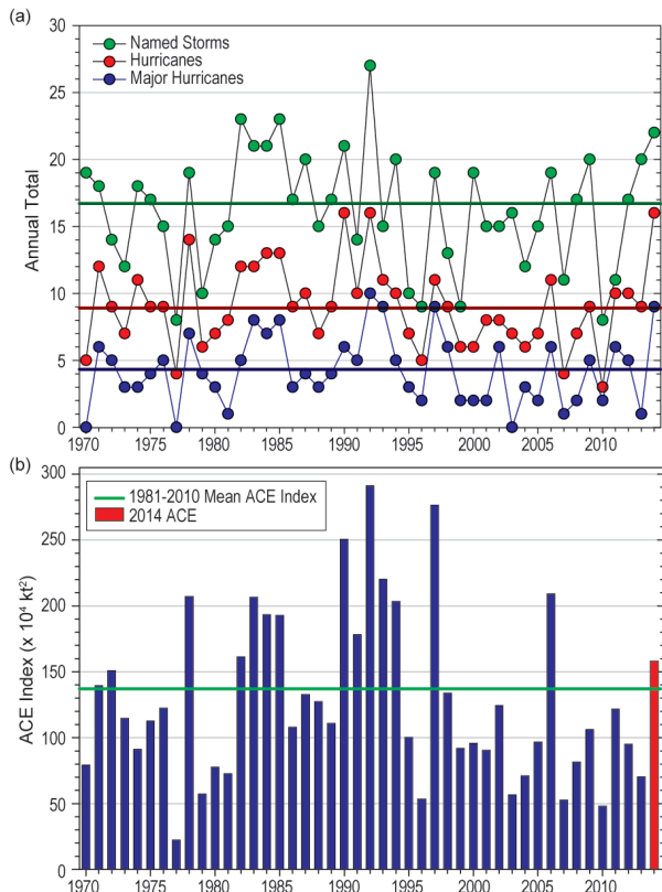
FIG. 4.24. Seasonal TC statistics for the full ENP/CNP basin over the period 1970–2014: (a) number of named storms, hurricanes, and major hurricanes, and (b) the ACE index ( \times 10^4 kt 2 ) with the 2014 seasonal total highlighted in red. The time series shown includes the corresponding 1981–2010 base period means for each parameter.
