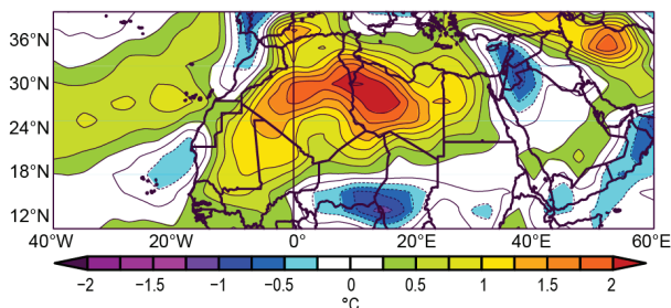
FIG. 7.17. Jul–Sep temperature anomaly (°C, 1981–2010 base period) for northern Africa.
