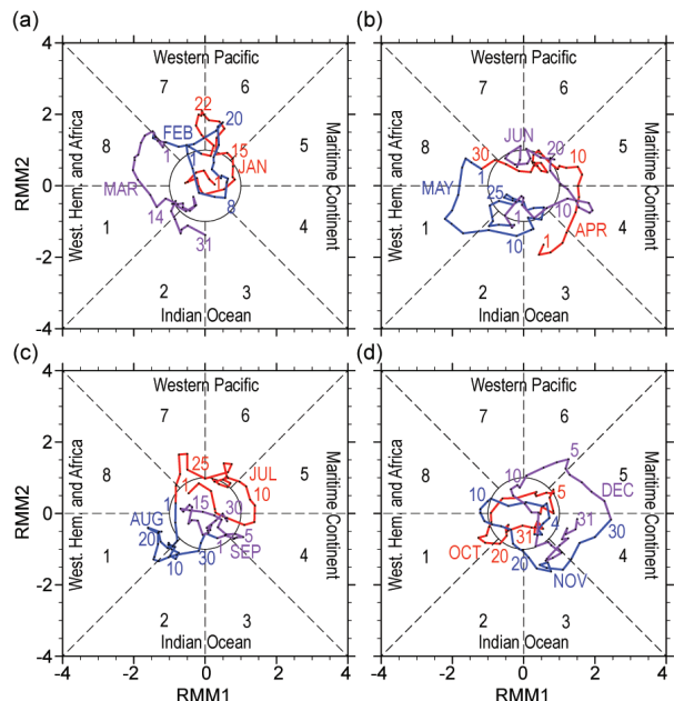
FIG. 4.9. Wheeler–Hendon (2004) Real-time Multivariate MJO (RMM) index for (a) Jan–Mar, (b) Apr–Jun, (c) Jul–Sep, and (d) Oct–Dec 2014. Each point represents the MJO’s amplitude and location on a given day and the connecting lines illustrate its propagation. Amplitude is indicated by distance from the origin, with points inside the circle representing weak or no MJO. The 8 phases around the origin identify the region experiencing enhanced convection, and counterclockwise movement is consistent with eastward propagation.
