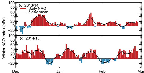
FIG. 2.26. Boreal winter sea level pressure anomalies (hPa, 1981–2010 base period) averaged over Dec–Feb for (a) 2013/14 and (b) 2014/15. NAO daily time series (hPa) for the winter of (c) 2013/14 and (d) 2014/15. The data shown are from HadSLP2r (Allan and Ansell 2006).
