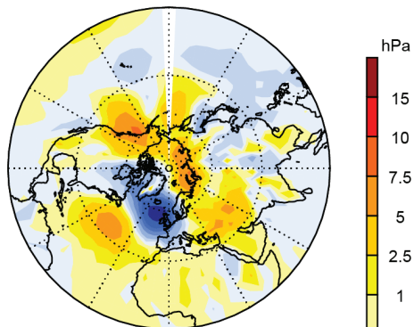
(b) Boreal Winter 2014/15
