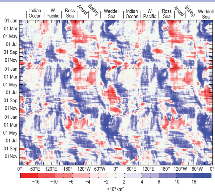
FIG. SB6.4. Anomalies of daily sea ice extent [ \times 10^3 km 2 (degree longitude) -1 ] from Jan 2012 to Dec 2014 represented as a Hovmöller. The values represent the areal extent of the anomaly integrated over a 1° longitude to the north of the continental edge ( \times 10^3 km 2 ). Note that the longitudes are repeated to display the spatial continuity of the sea ice extent anomalies.
