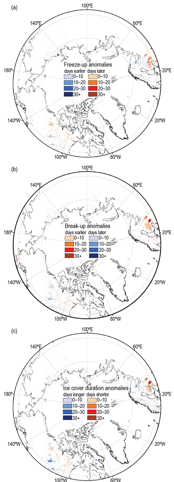
FIG. 5.20. (a) Freeze-up, (b) break-up, and (c) ice cover duration anomalies for the 2013/14 ice season relative to the 2004–13 mean from the NOAA IMS 4-km product. Freeze-up and break-up dates, and ice duration were derived at the pixel level.
