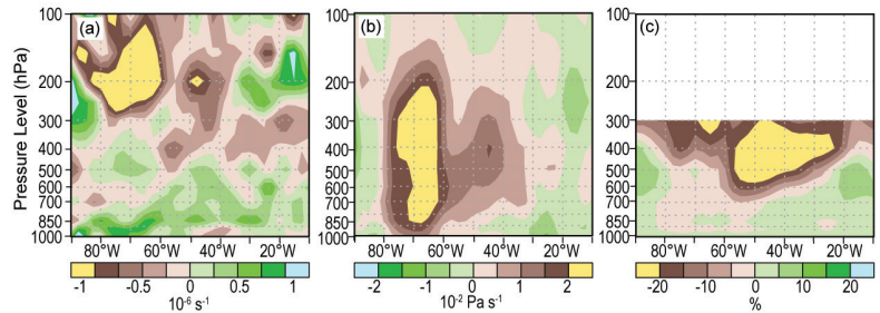
FIG. 4.22. ASO 2014: Atmospheric height-longitude sections averaged in the MDR (9.5°–21.5°N) of (a) anomalous divergence ( \times 10^{-6} \text{ s}^{-1} ), (b) anomalous vertical velocity ( \times 10^{-2} \text{ Pa s}^{-1} ), and (c) % of normal specific humidity up to 300 hPa. Green shading indicates anomalous divergence, anomalous rising motion, and increased moisture, respectively. Brown shading indicates anomalous convergence, anomalous sinking motion, and decreased moisture, respectively. Departures are with respect to the 1981–2010 monthly means.
