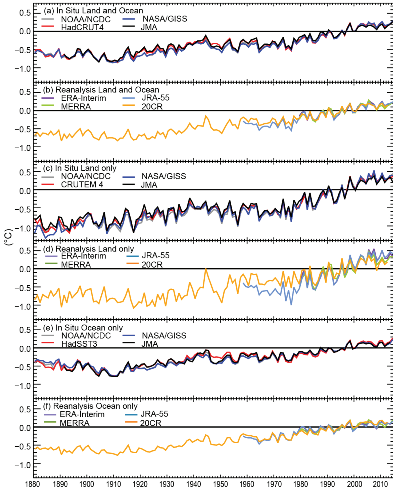
FIG. 2.1. Global average surface temperature anomalies (°C, 1981–2010 base period). In situ estimates are shown NOAA/NCDC (Smith et al. 2008), NASA/GISS (Hansen et al. 2010), HadCRUT4 (Morice et al. 2012), CRUTEM4 (Jones et al. 2012), HadSST3 (Kennedy et al. 2011a,b) and JMA (Ishihara 2006). Reanalyses estimates are shown from ERA-Interim (Dee et al. 2011a), MERRA (Rienecker et al. 2011; provided by M. Bosilovich), JRA-55 (Ebita et al. 2011; provided by S. Kobayashi), and 20CR (Compo et al. 2011; provided by C. Smith).
