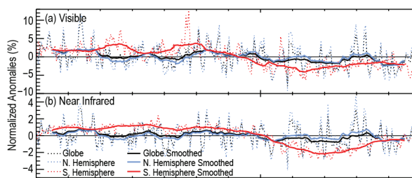
FIG. 2.54. Globally averaged MODIS White Sky broadband surface albedo (NASA) normalized anomalies in the (a) visible and (b) near-infrared domain relative to a 2003–14 base period.
