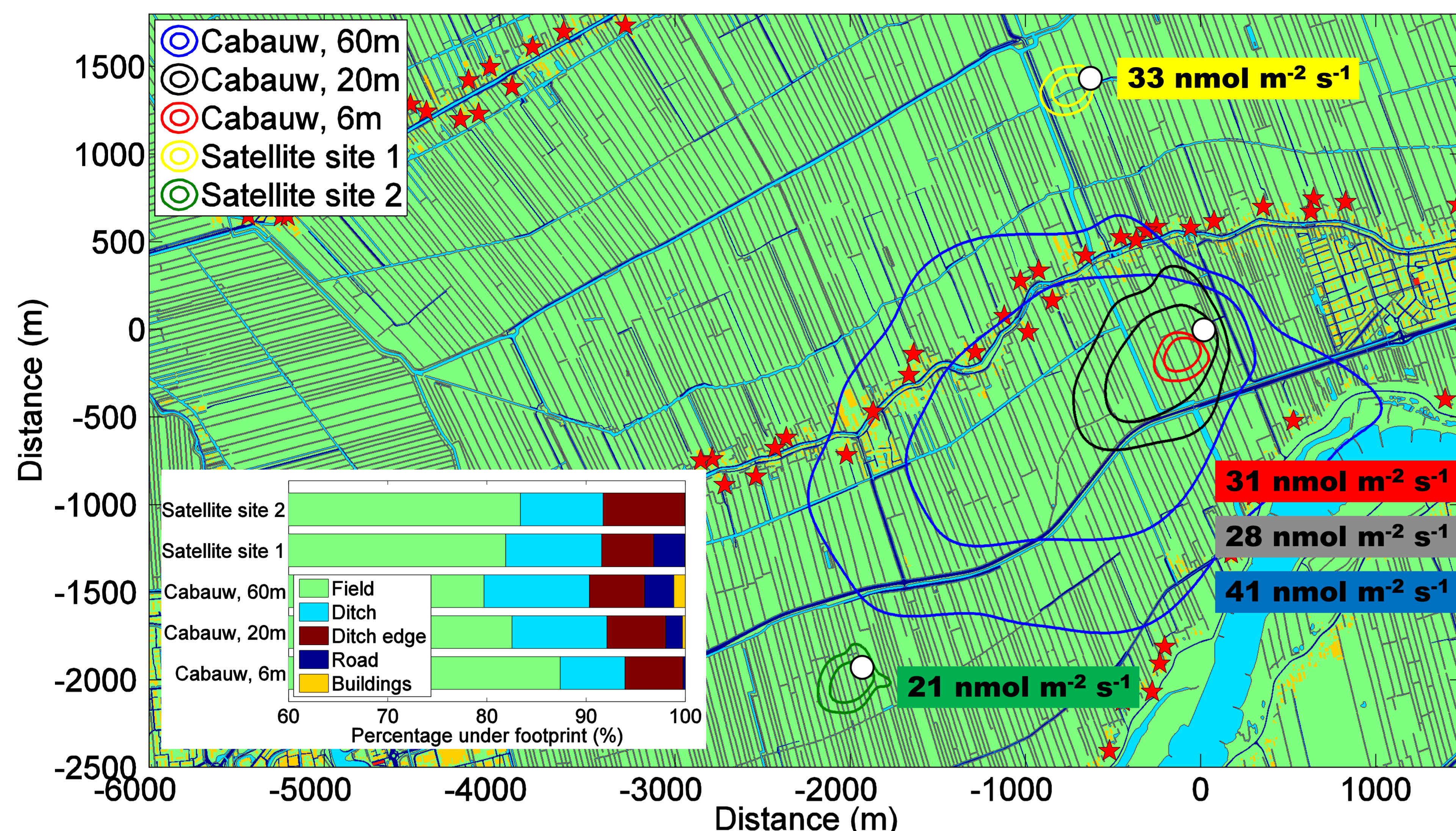
Figure 1: Cumulative footprints, i.e. source areas, for different flux measurement locations. Footprints were calculated based on Kijun et al. (2004). 80 th and 60 th percentile curves are shown, meaning that 80 % (60 %) of the measured signal originated from within the shown area. Land cover map was created using TOP10 vector product [5]. White dots show the tower and red stars show the farm locations. Average flux levels are also shown in the plot. Inset: percentage of different land use elements within the footprints on average.
