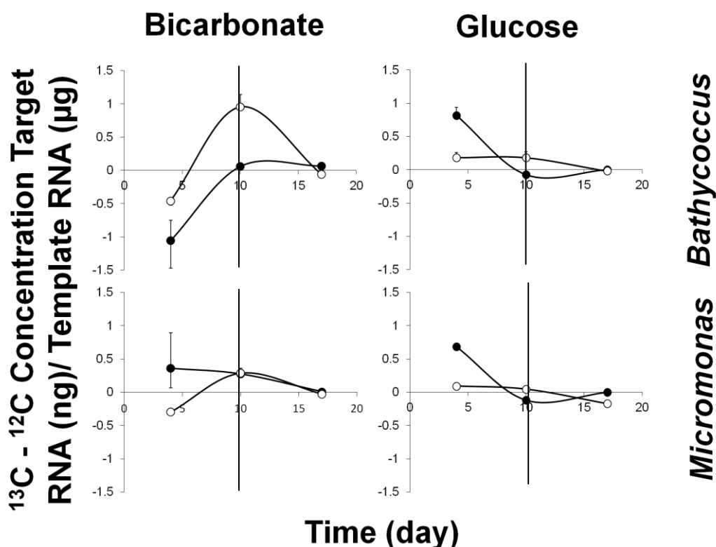
Figure 6.3: Changes in RT-qPCR abundance during stable isotope microcosm incubations for Bathycoccus and Micromonas . Relative uptake Elevated M1 CO 2 incubations (closed circles) compared to ambient M6 incubations (open circles). Relative uptake of 13 C substrate assessed by concentration of target RNA in 12 C incubations subtracted from target concentration in 13 C incubations. Positive values in bicarbonate and glucose incubations are taken to have higher activity in 13 C incubations compared to equivalent 12 C incubation (fraction 5) and were therefore assumed to be actively metabolising substrate. Error bars represent standard deviation from triplicate RT-qPCR reactions. Positive error bars corresponded to 13 C incubation values, negative to 12 C. Vertical line denotes the separation of phases 1 and 2.
