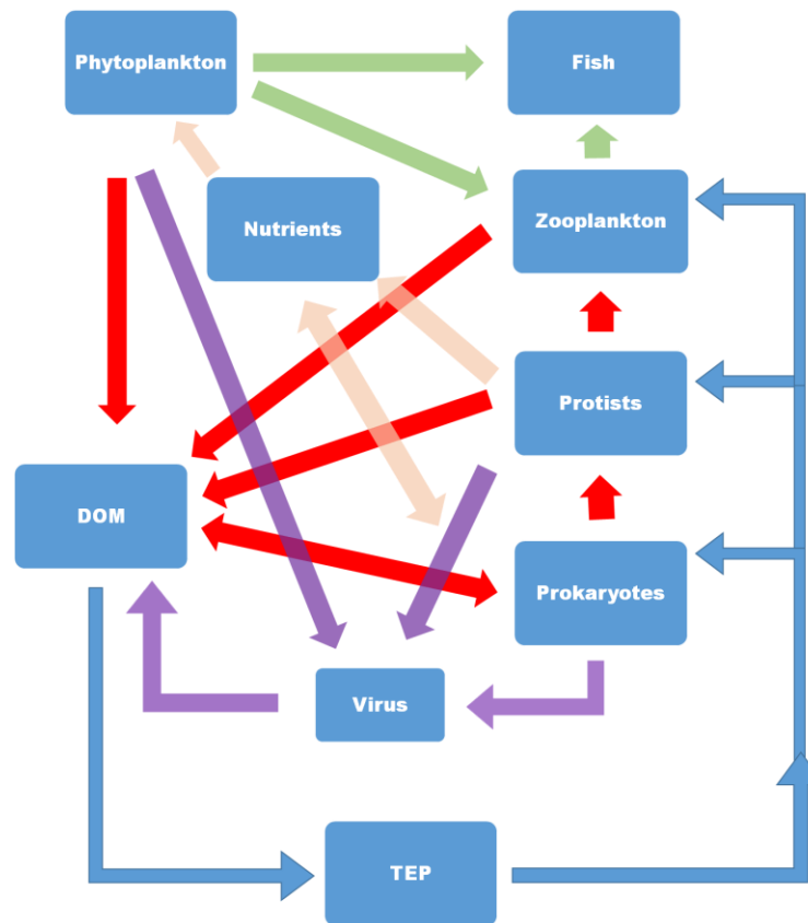
Figure 1.2: Simplified diagram of the pelagic food web. Four major pathways are illustrated, the classical food web (green), the microbial loop (red), the viral shunt (purple) and the abiotic loop (blue). Nutrient pathways are shown (pink). This figure and legend are adapted from Weinbauer et al. (2011).
