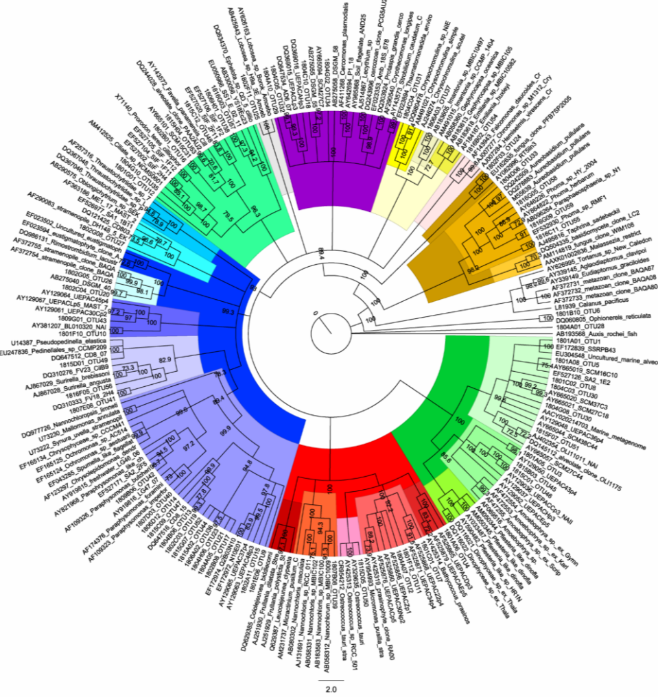
Figure 4.3b: A 70 % Majority Rule Consensus Tree of picoeukaryotic OTUs as inferred by Neighbour Joining distance criterion under GTR+I+G model. Bootstrap support from 1000 replicates are shown at nodes. Phyla/sub-phyla are highlighted as follows: Blue = Stramenopiles, Red = Archaeplastida, Purple = Rhizaria (inc Cercozoa), Yellow = Prymnesiophyceae, Orange = Fungi and Green = Alveolata. For more specific taxonomic grouping refer to key.
