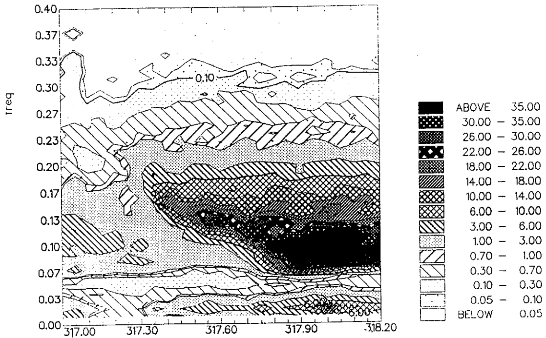
Figure 8 Time series of energy density spectra from the SBWR, covering the period from day 317 to day 318.2. The vertical axis is frequency (Hz) and the contours show the energy density ( m^2/Hz ).
