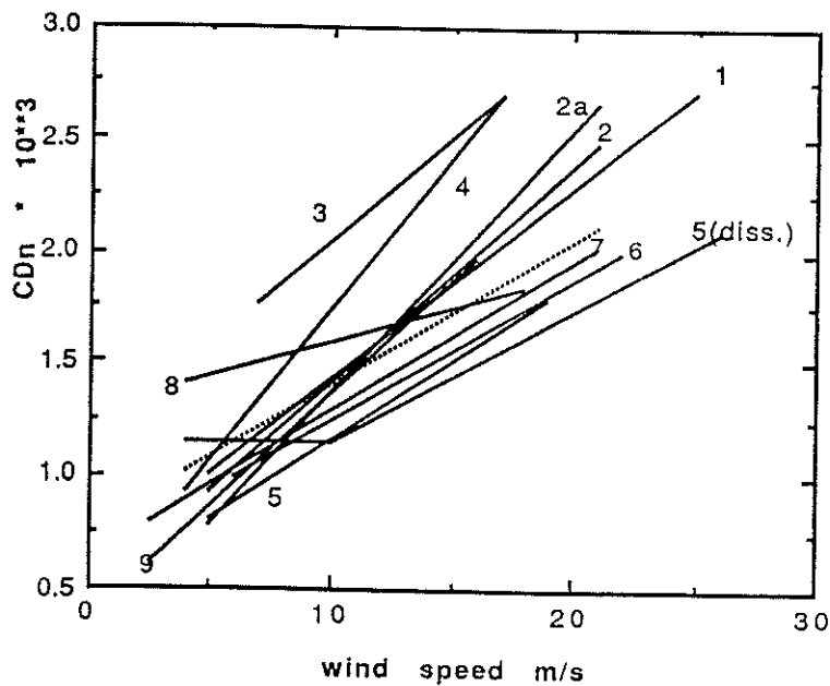
Figure 2 Data reviewed by Garratt (1977) (dotted line) and Geernaert (1990) (solid lines). The numbers refer to the references in Table 1 of the text; "2a" is the data from Geernaert (1986) where surface currents have been allowed for, and "5diss." is the Large and Pond (1991) data obtained by the dissipation method rather than by the eddy correlation method (line "5" in this figure).
