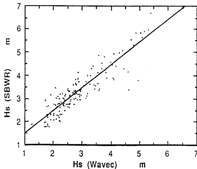
Figure 9 Comparison of significant wave height data from the Ship Borne Wave Recorder (vertical axis) and the WAVEC buoy (horizontal axis). The least squares regression line is shown.
