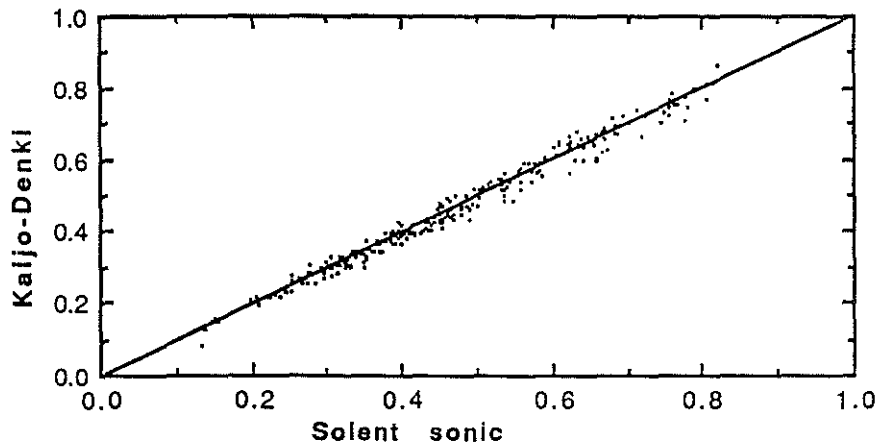
Figure 6 Friction velocity data from CD43 for the two different sonic anemometers, with the least squares regression line shown.
