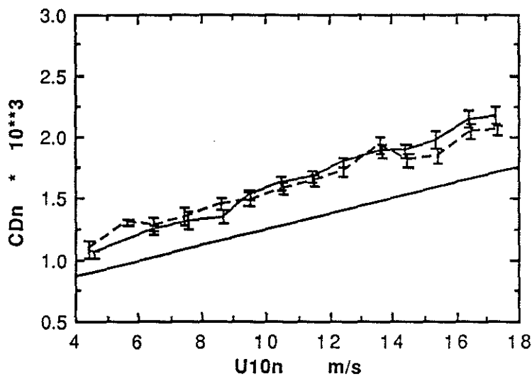
Figure 11 Drag coefficient vs. wind speed relationship from the CD43 Solent sonic data, showing the different methods used to calculate true wind speed; em log (solid line), and ship's speed over the ground (dashed line). The Smith (1980) relationship is indicated by the straight solid line.
