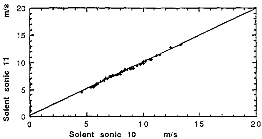
Figure 7 Wind speed comparison for the two Solent sonic anemometers used during CD62a. The least squares regression is shown.
