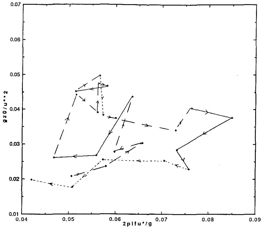
Figure 14 Non-dimensional roughness length against non-dimensional inverse wave age for day 317. Data from the Solent sonic anemometer is used. Periods of increasing wind are indicated by a dashed line, steady winds by a solid line and decreasing wind by a dotted line.
