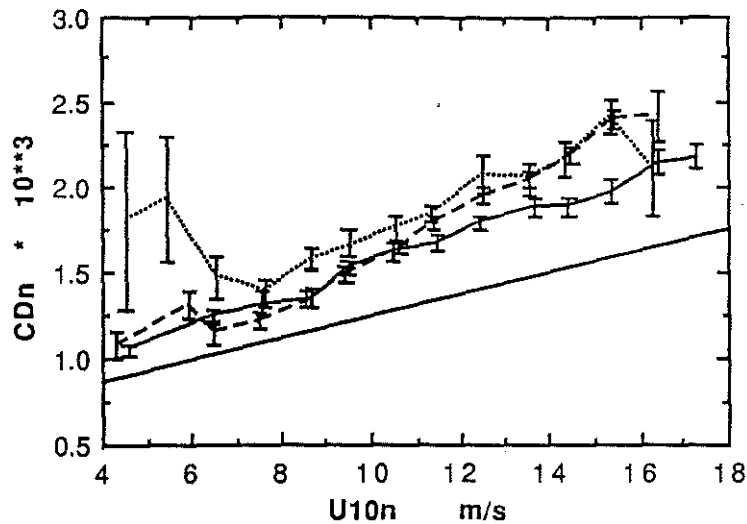
Figure 10 Drag coefficient vs. wind speed relationship from the three anemometers used during CD43; the Solent sonic (solid line), the Kaijo-Denki (dashed line) and the Young (dotted line). Error bars indicate the standard deviation. The Smith (1980) relationship is shown by the straight solid line.
