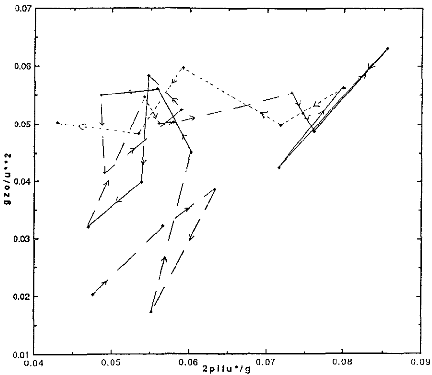
Figure 15 As for Figure 14 but data from the Kaijo-Denki anemometer has been used instead of that from the Solent sonic anemometer.
