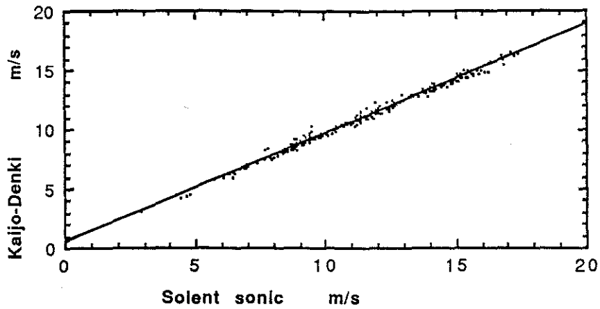
Figure 5 Wind speed data from CD43 for the two different sonic anemometers, with the least squares regression line shown.
