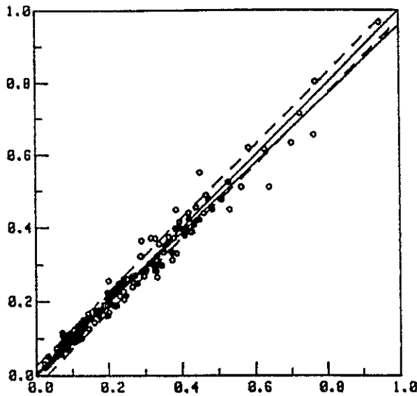
Figure 3 Reproduction of fig.13a from Edson et.al.(1991), showing stress estimates obtained by the dissipation method on the vertical axis ( \rho u_*^2 ), and from the eddy correlation method on the horizontal axis ( -\rho \langle uw \rangle ).
