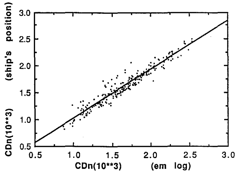
Figure 12 Scatter plot of the drag coefficients calculated using the two different methods of obtaining true wind speed from the same data. The least squares regression line is shown.
