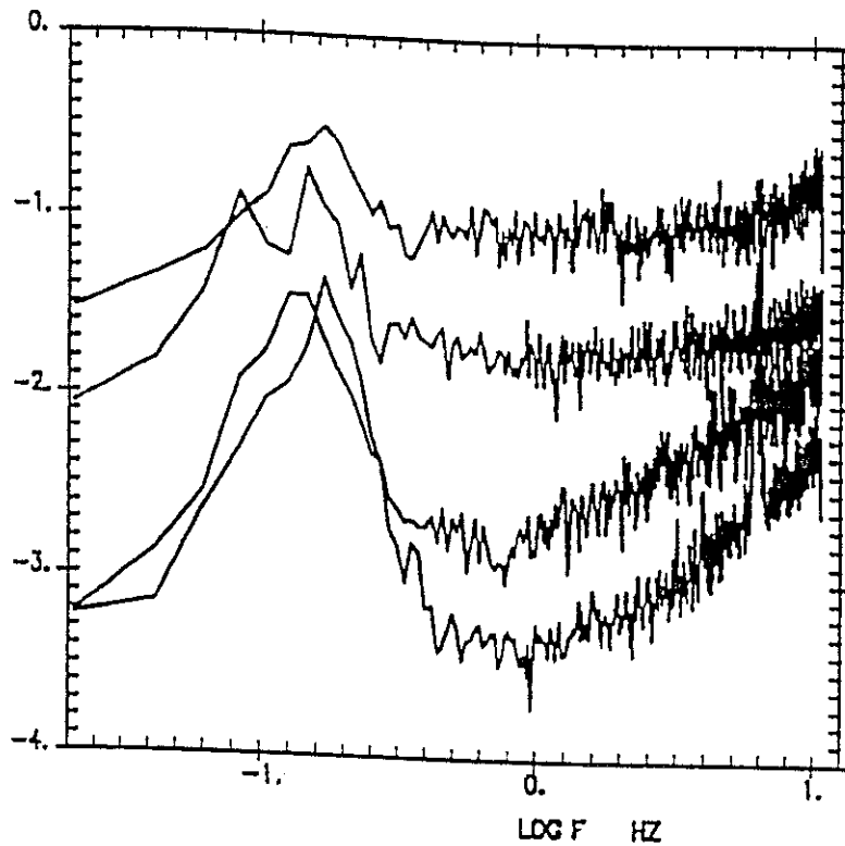
Figure 1 Wind speed spectra obtained at mean wind speeds of, from the top down, 15.5, 10, 3 and 2.5 m/s. The vertical axis is \log_{10}(S f^{5/3}) , where S is the power spectral density, and the horizontal axis is \log_{10} f .
