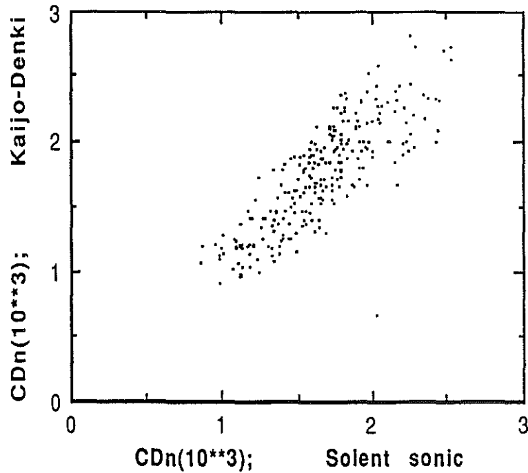
Figure 17 Drag coefficients produced from the Kaijo-Denki anemometer against those from the Solent sonic.
