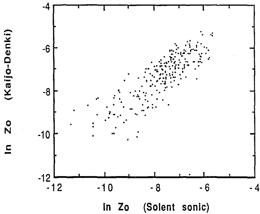
Figure 16 \log_e of the roughness lengths from the two sonic anemometers.
