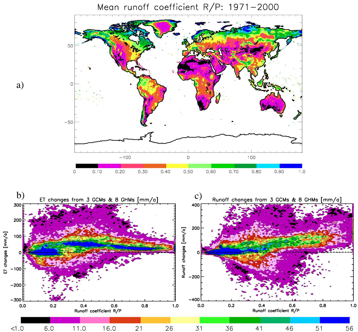
Fig. 6. (a) Ensemble mean runoff coefficient ( R/P ) for present day (1971–2000), and scatter plots showing how the runoff coefficient relates to the A2 changes in (b) evapotranspiration and (c) runoff obtained from the GCM–GHM ensemble. For (b) and (c), the colours show the number of scatter points.
