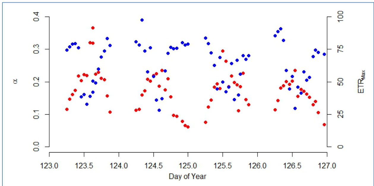
Fig. 43 Discrete rapid light curves measured during JC071 showing diurnal variations in light limited electron transport rates ( \alpha ) and maximum electron transport rates ( ETR_{\text{MAX}} ).
