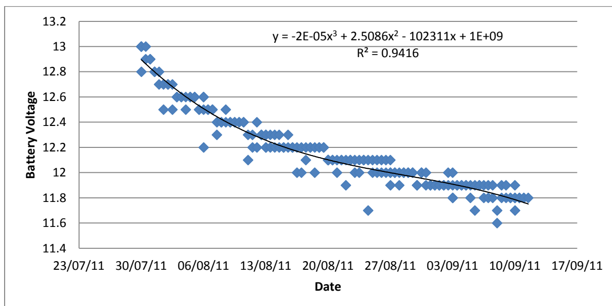
Fig. 16 Change in NAS battery voltage over time.
