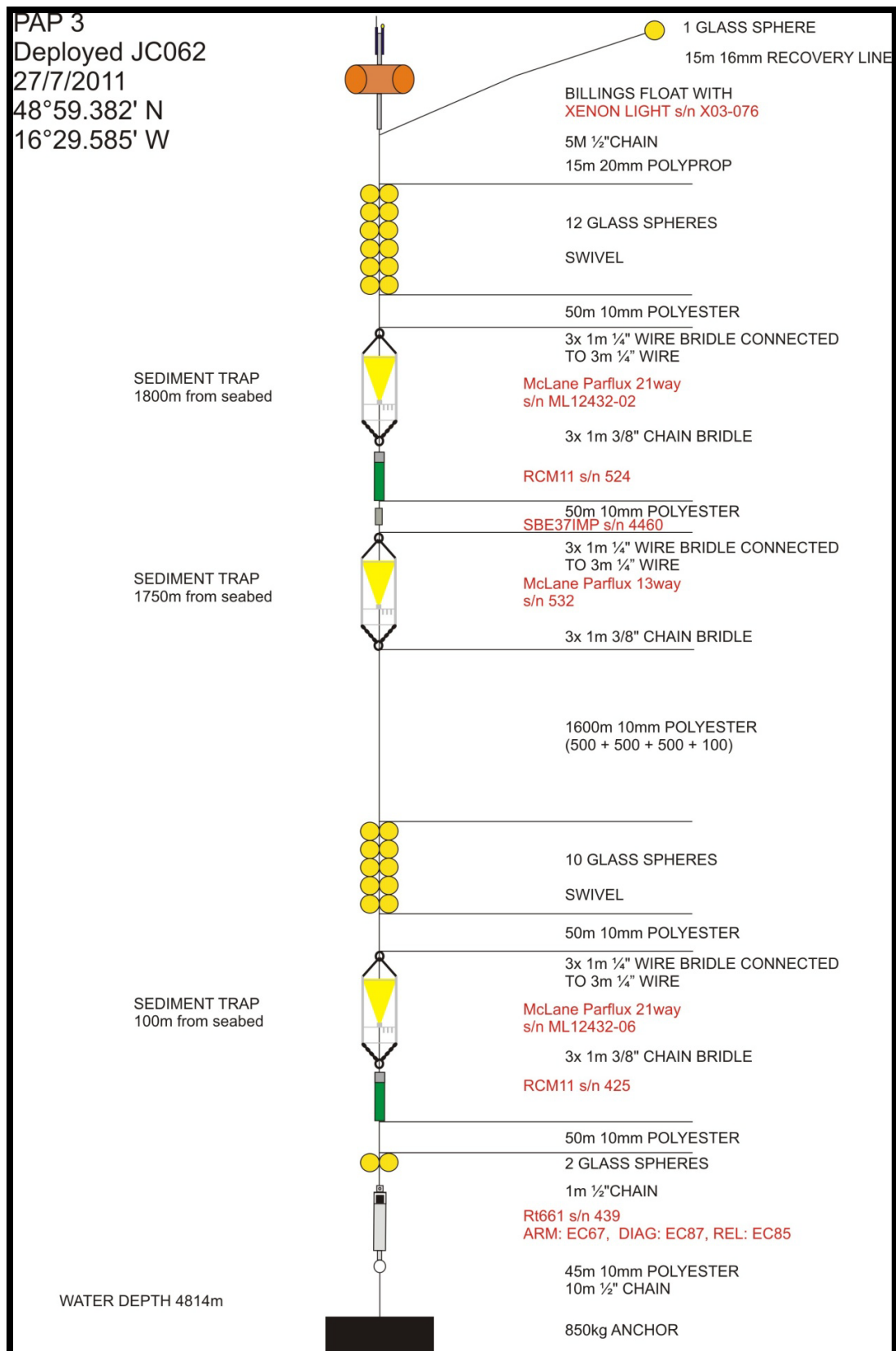
Fig. 28 PAP3 recovered mooring.
