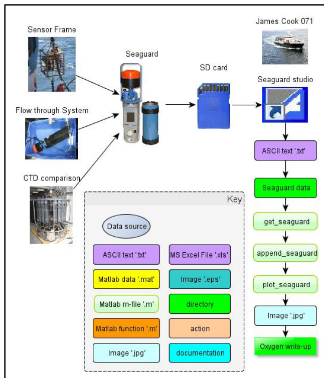
Fig. 25 Process flowchart.
