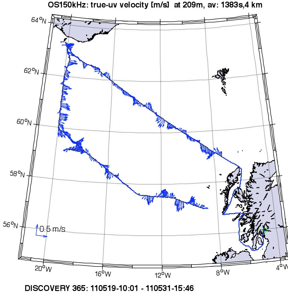
Figure 8. Absolute velocity vectors at 209 m, 4 km averages for all transects I – IV.
