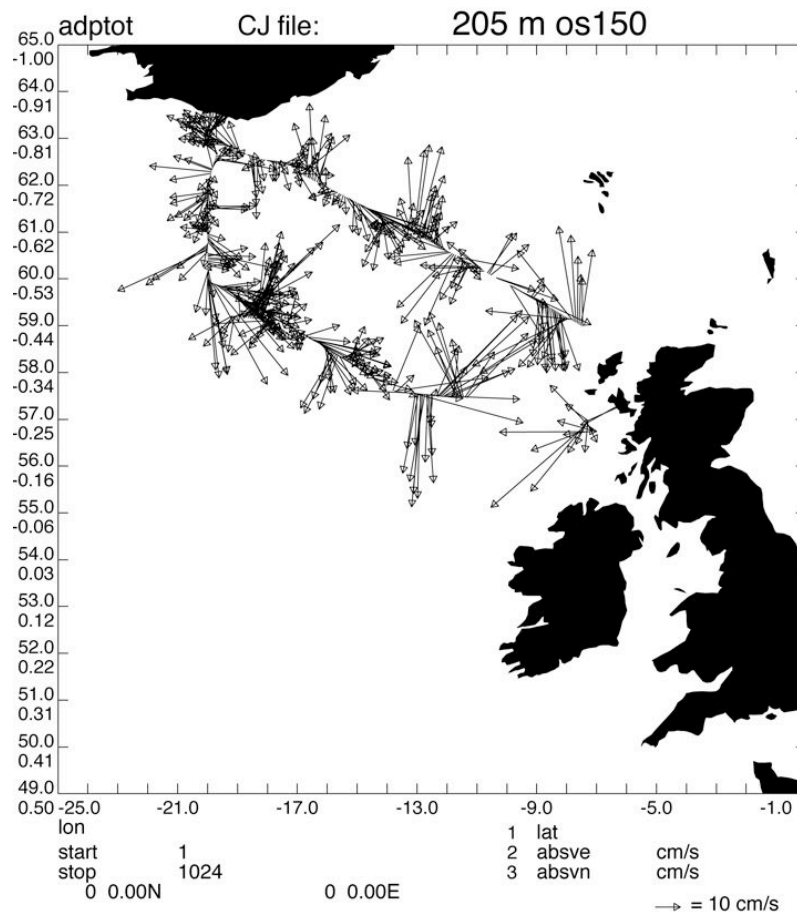
Figure 6. Absolute velocity vectors for 4 km averages at 205 m bindepth.
