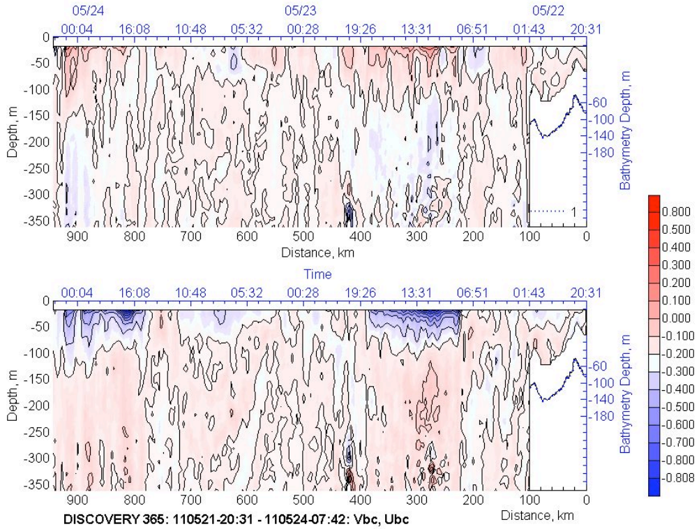
Figure 10b. Meridional ( V_{bc}=v-V_{bt} ) and zonal ( U_{bc}=u-U_{bt} ) velocity, transect II (8 m × 4 km).
