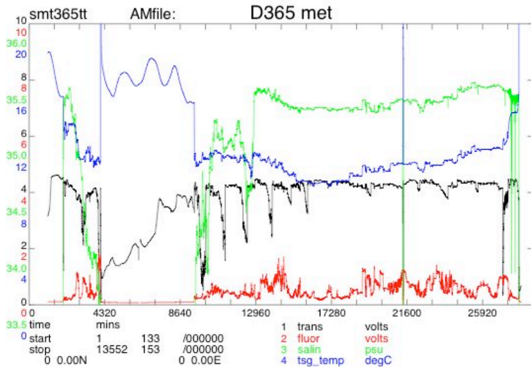
Figure 15. Surface water conditions as measured by the thermosalinograph during RRS Discovery cruise 365 (trans – transmittance, fluor – fluorescence, salin – salinity, tsg_temp – sea surface temperature).
