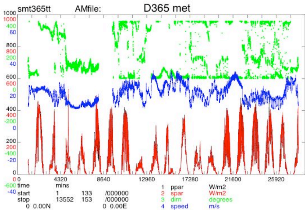
Figure 14. Wind speed and direction during RRS Discovery cruise 365 (ppar, spar – port, starboard photosynthetically active radiation, speed, dirn – wind speed and direction).
