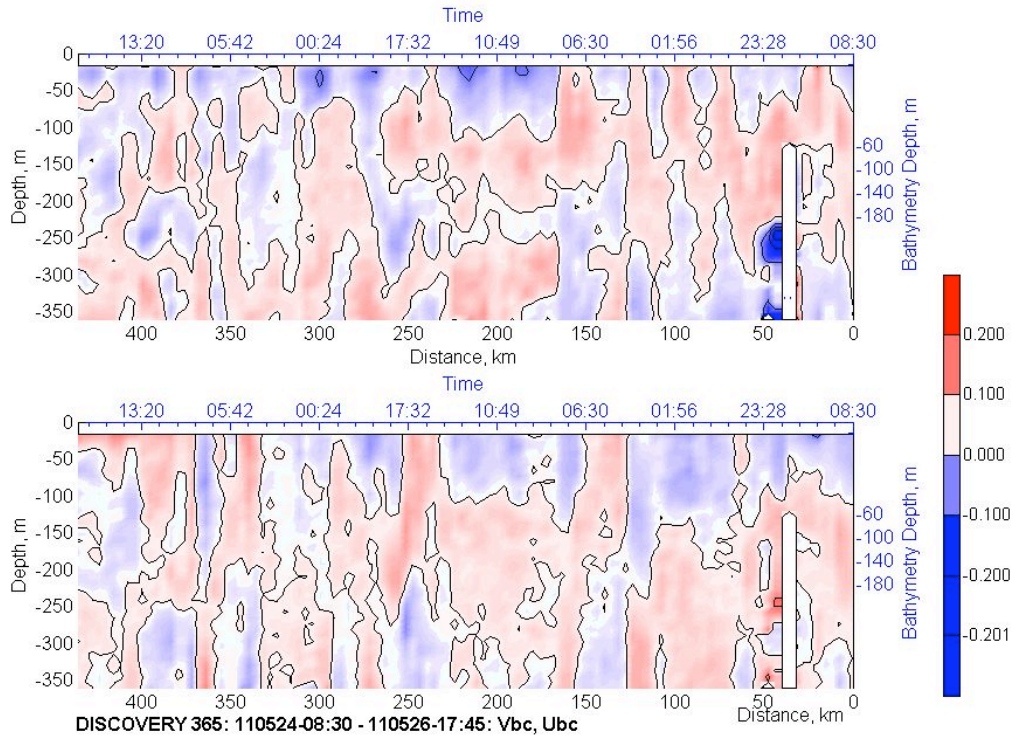
Figure 11a. Total Meridional ( v ) and zonal ( u ) velocity, transect II ( 8 \text{ m} \times 4 \text{ km} ).
