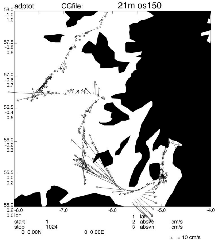
Figure 5. Absolute velocity vectors for 4 km averages at 21 m bindepth.
