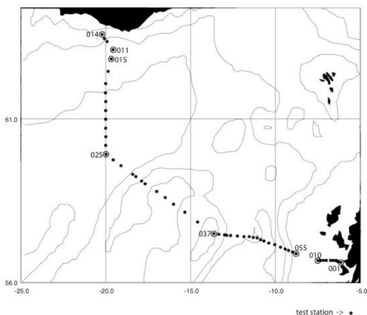
Figure 1. CTD station positions during RRS Discovery cruise 365 (bathymetry contoured at 200, 1000, 2000, 3000 m).
