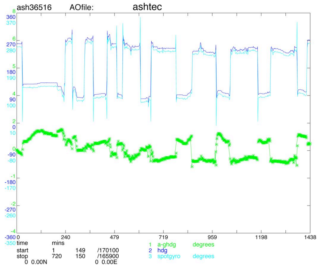
Figure 4. Example of the onscreen output of daily navigation hdg data generated by gyro (light blue line), ashtech ADU5 (dark blue line) and the difference between them (green line).
