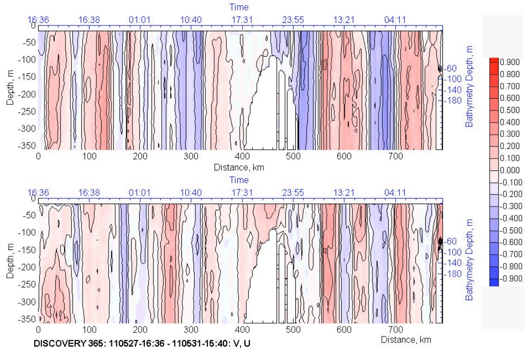
Figure 12a. Total Meridional ( v ) and zonal ( u ) velocity, transect IV ( 8 \text{ m} \times 4 \text{ km} ).
