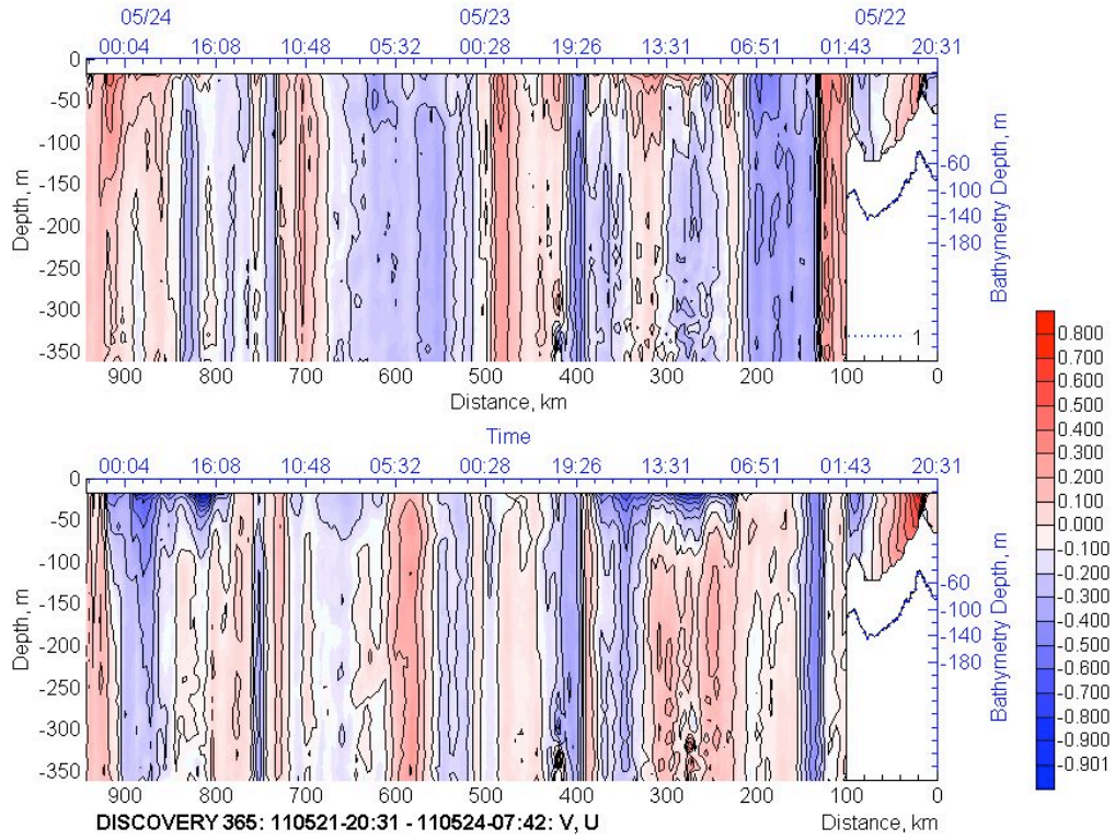
Figure 10a. Total Meridional ( v ) and zonal ( u ) velocity, transect II (8 m × 4 km).
