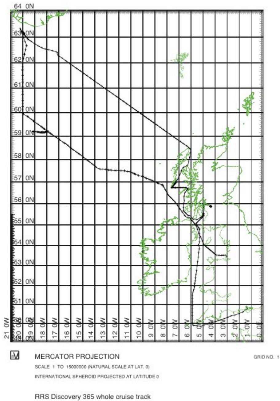
Figure 2. RRS Discovery cruise 365 track.
