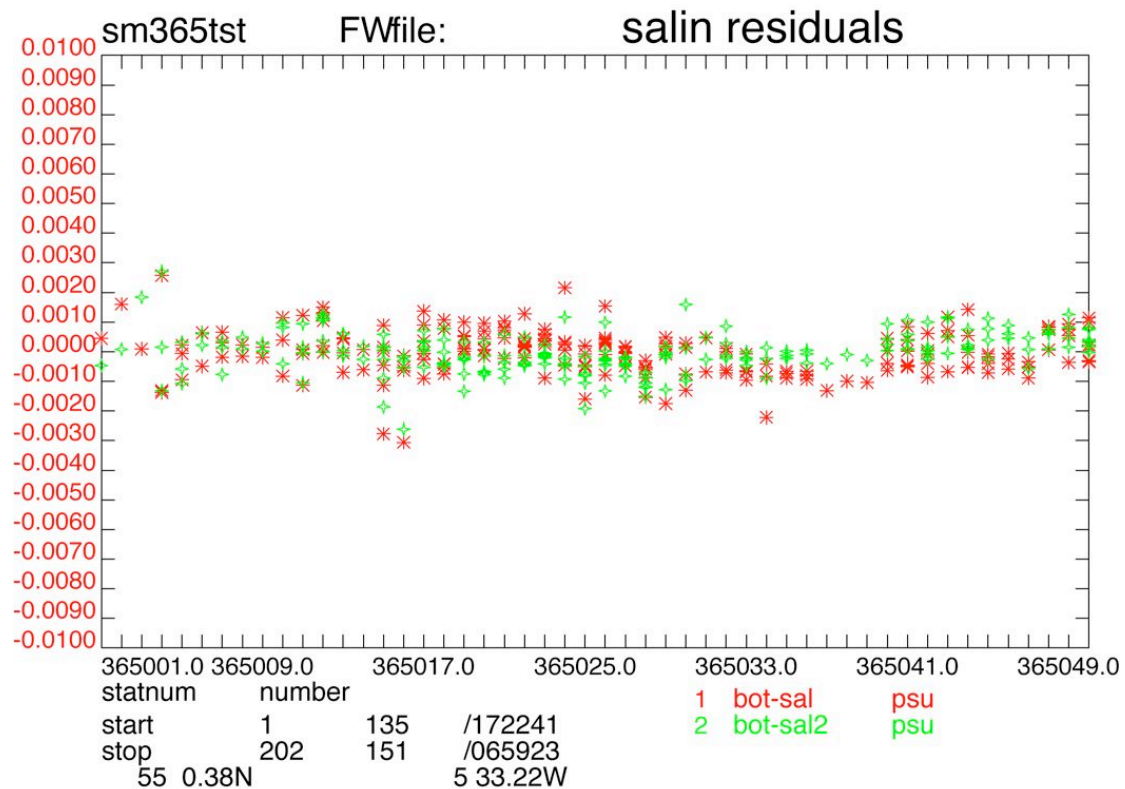
Figure 3. Bottle-CTD salinity residuals after calibration
