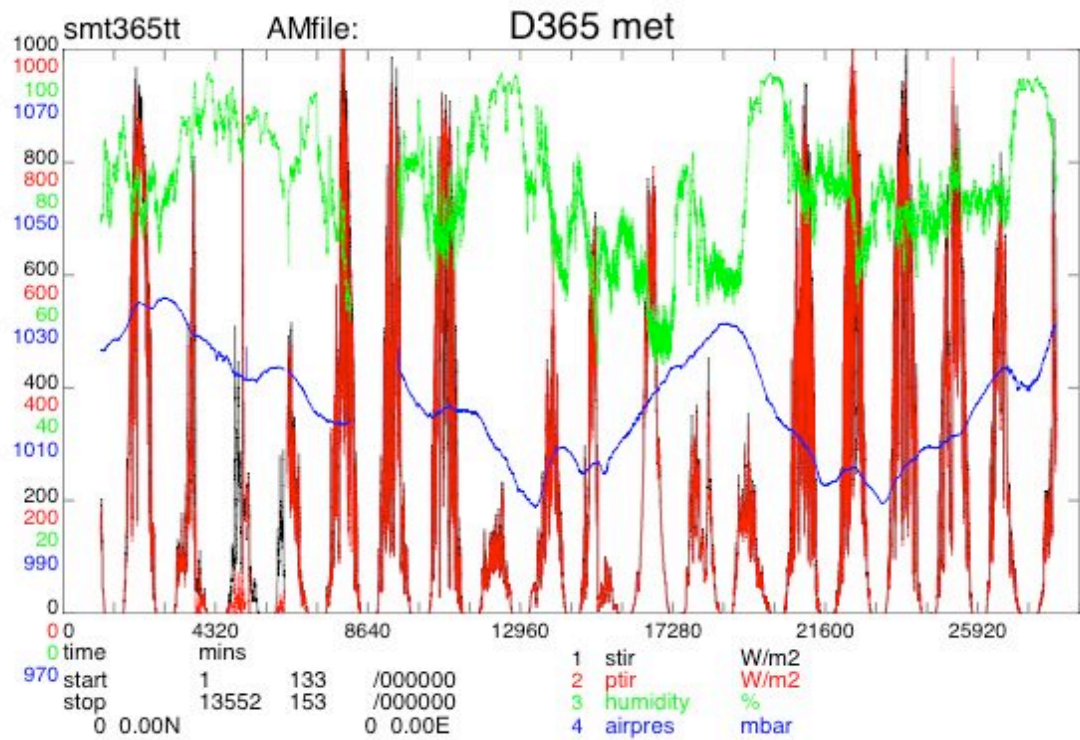
Figure 13. Meteorological conditions during RRS Discovery cruise 365 (stir, ptir – starboard, port total irradiance, airpres – atmospheric air pressure).
