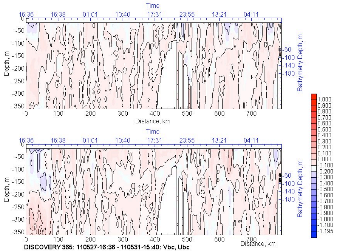
Figure 12a. Total Meridional ( v ) and zonal ( u ) velocity, transect IV ( 8 \text{ m} \times 4 \text{ km} ).
