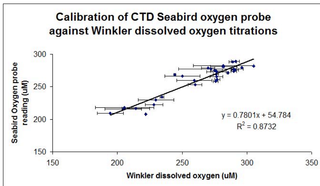
Figure 16. Comparison of CTD Seabird oxygen probe against Winkler dissolved oxygen titrations.
